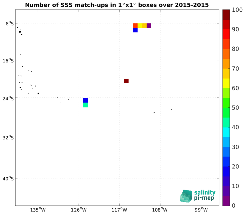
Figure 4: Number of SSS match-ups between Surface drifters SSS and the Aquarius SSS L3 CAP v5 - Monthly (JPL) SSS product for the OTT zone Pi-MEP region over 1°×1° boxes and for the full satellite product period.
