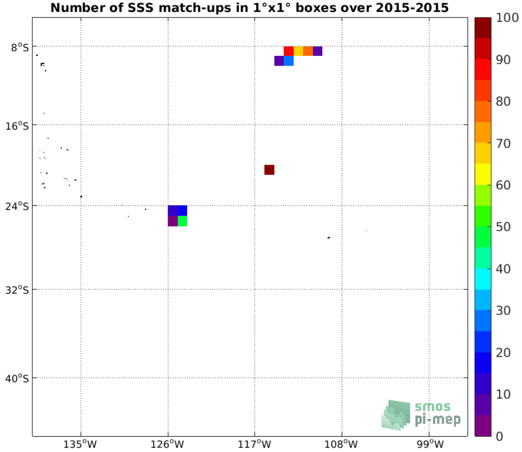
Figure 3: Number of SSS match-ups between Surface drifters SSS and the Aquarius SSS L3 CAP v5 - Monthly (JPL) SSS product for the OTT zone Pi-MEP region over 1°x1° boxes and for the full satellite product period.
