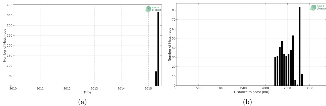
Figure 1: Number of match-ups between Surface drifters and Aquarius-L3-JPL-V5-MONTHLY SSS as a function of time (a) and as function of the distance to coast (b) over the OTT zone Pi-MEP region and for the full satellite product period.
