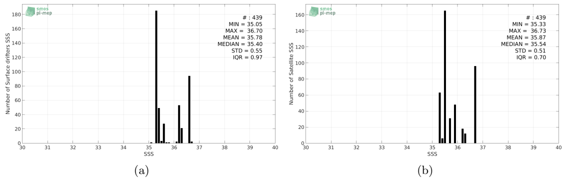
Figure 2: Histograms of SSS from Surface drifters (a) and Aquarius-L3-JPL-V5-MONTHLY (b) considering all match-up pairs per bins of 0.1 over the OTT zone Pi-MEP region and for the full satellite product period.
