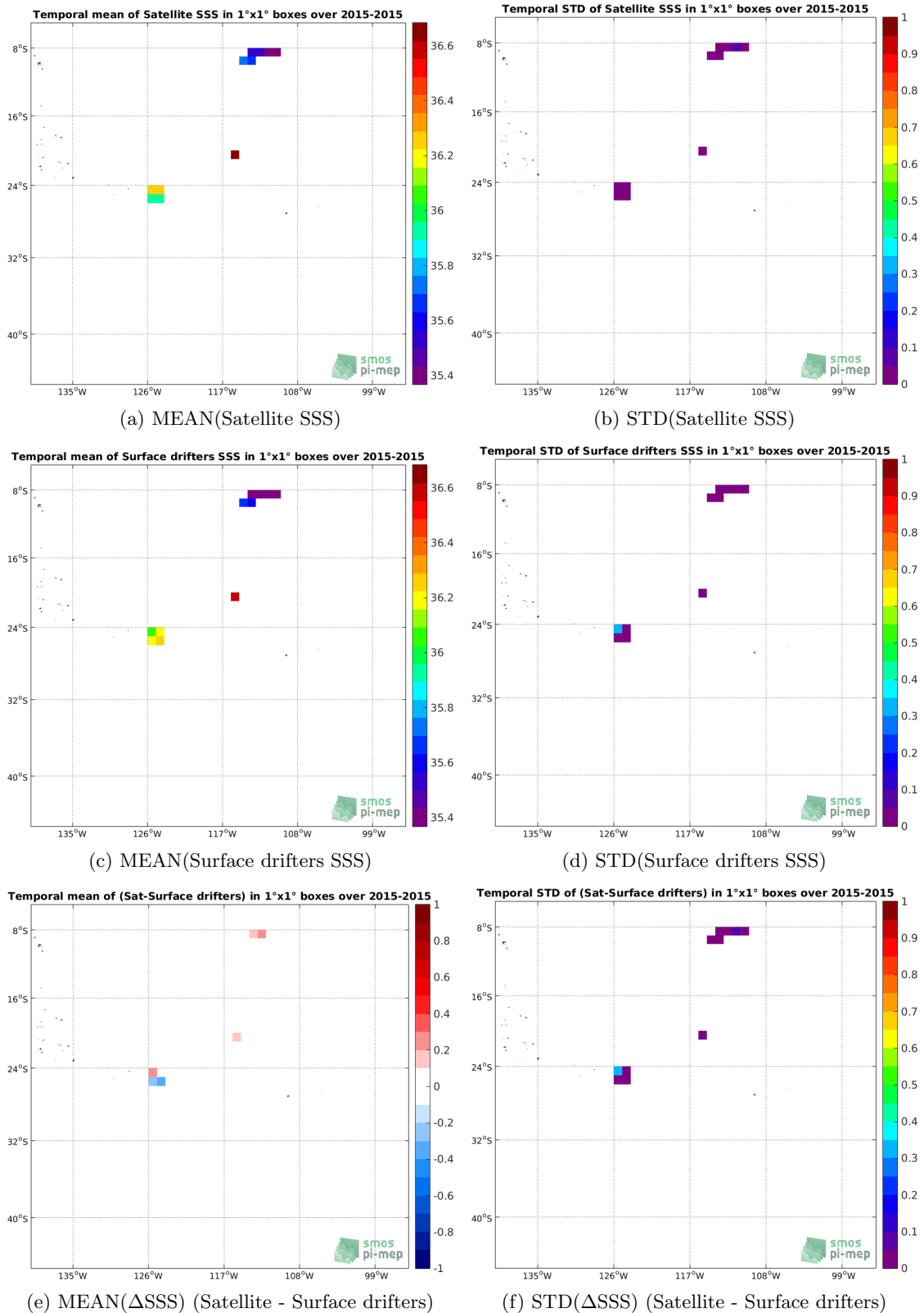
Figure 5: Temporal mean (left) and STD (right) of SSS from Aquarius-L3-JPL-V5-MONTHLY (top), Surface drifters (middle), and of \Delta SSS (Satellite - Surface drifters). Only match-up pairs are used to generate these maps.
