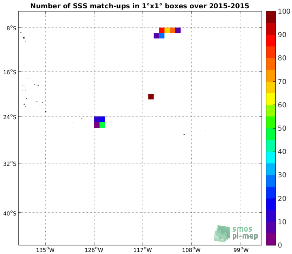
Figure 3: Number of SSS match-ups between Surface drifters SSS and the Aquarius-L3-JPL-V5-MONTHLY SSS product for the OTT zone Pi-MEP region over 1°x1° boxes and for the full satellite product period.
