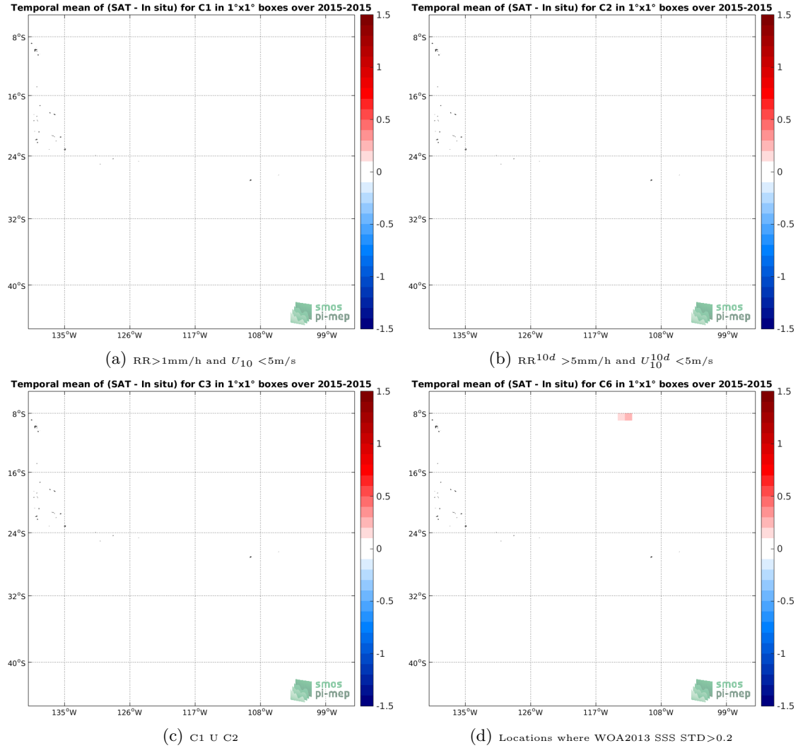
Figure 11: Temporal mean gridded over spatial boxes of size 1^\circ \times 1^\circ of \Delta SSS (Aquarius-L3-JPL-V5-MONTHLY - Surface drifters) for 4 different subdatasets corresponding to: RR > 1\text{mm/h} and U_{10} < 5\text{m/s} (a), RR^{10d} > 5\text{mm/h} and U_{10}^{10d} < 5\text{m/s} (b), C1 U C2 (c), Locations where WOA2013 SSS STD > 0.2 (d).
