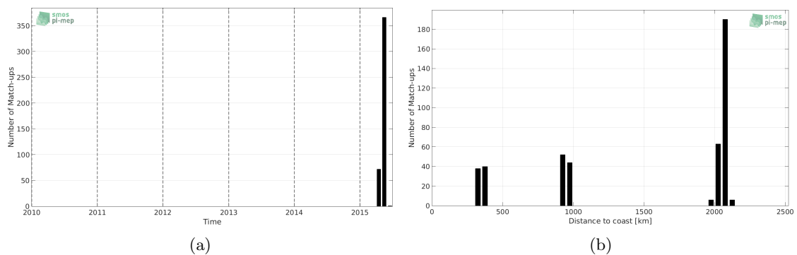
Figure 1: Number of match-ups between Surface drifters and Aquarius-L3-JPL-V5-MONTHLY SSS as a function of time (a) and as function of the distance to coast (b) over the OTT zone Pi-MEP region and for the full satellite period.
