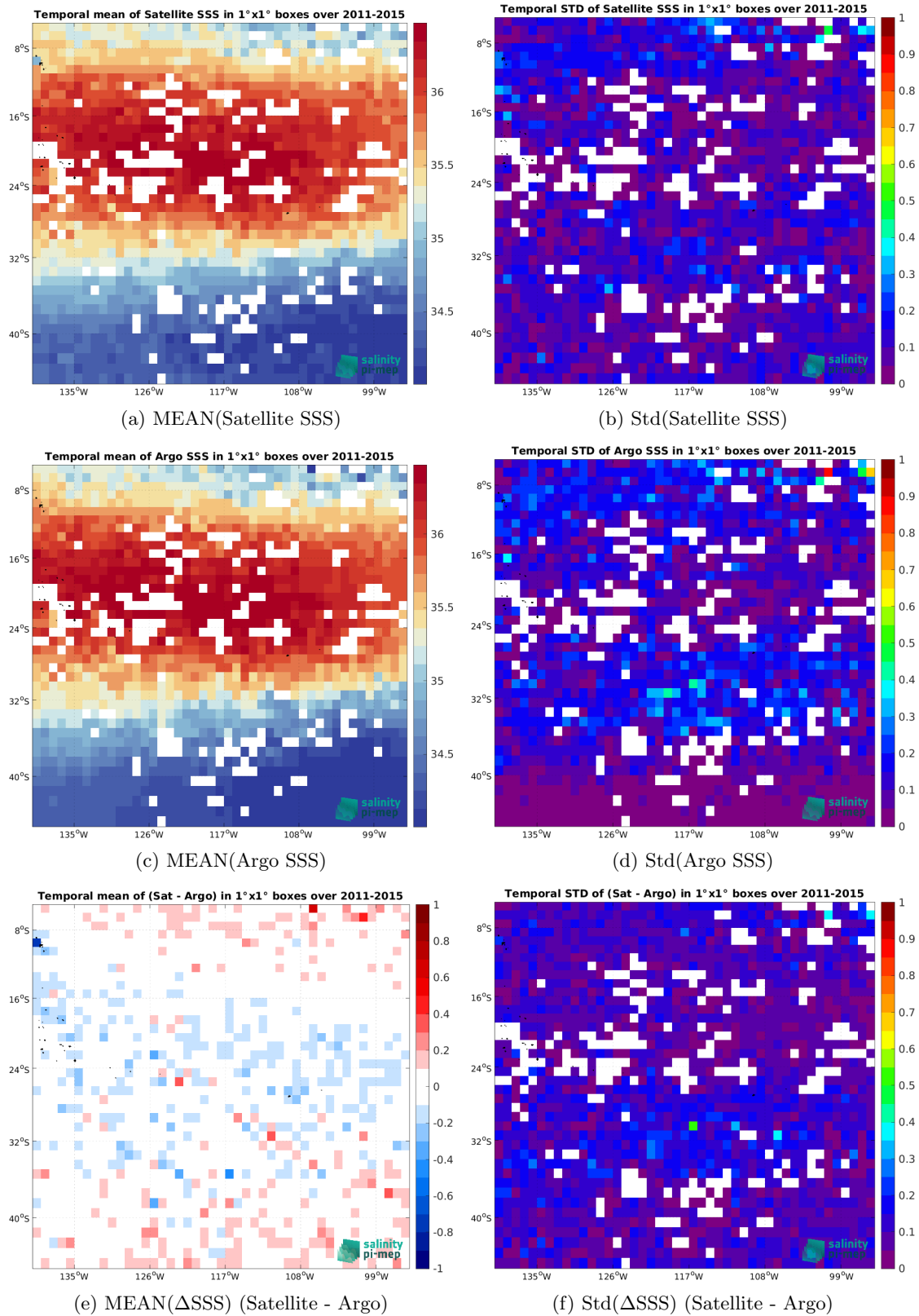
Figure 7: Temporal mean (left) and Std (right) of SSS from Aquarius SSS L3 CAP v5 - Monthly (JPL) (top), Argo (middle), and of \Delta SSS (Satellite - Argo). Only match-up pairs are used to generate these maps.
