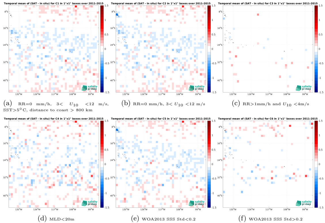
Figure 14: Temporal mean gridded over spatial boxes of size 1^\circ \times 1^\circ of \Delta SSS (Aquarius SSS L3 CAP v5 - Monthly (JPL) - Argo) for 6 different subdatasets corresponding to:RR=0 mm/h, 3 < U_{10} < 12 m/s, SST >5^\circ\text{C} , distance to coast > 800 km (a), RR=0 mm/h, 3 < U_{10} < 12 m/s (b), RR >1 mm/h and U_{10} < 4 m/s (c),MLD <20 m (d),WOA2013 SSS Std <0.2 (e),WOA2013 SSS Std >0.2 (f).
