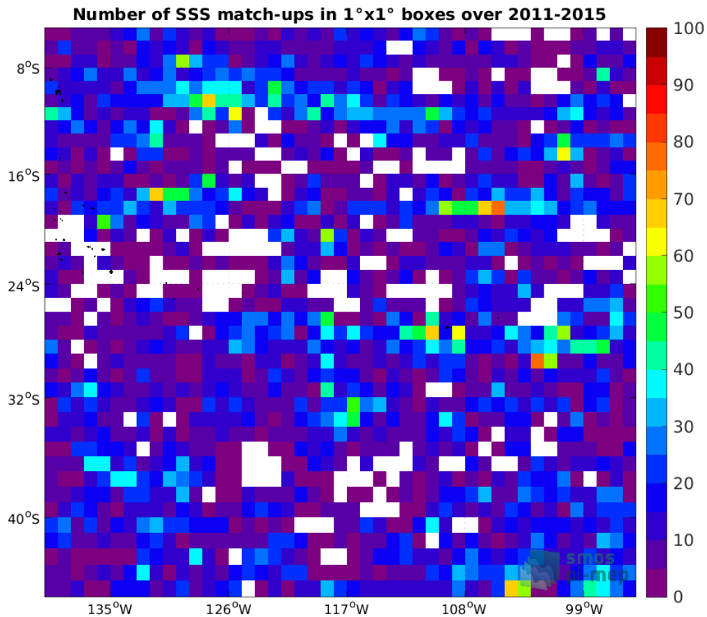
Figure 4: Number of SSS match-ups between Argo SSS and the Aquarius SSS L3 CAP v5 - Monthly (JPL) SSS product for the OTT zone Pi-MEP region over 1°x1° boxes and for the full satellite product period.
