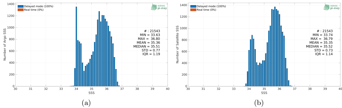
Figure 2: Histograms of SSS from Argo (a) and Aquarius SSS L3 CAP v5 - Monthly (JPL) (b) considering all match-up pairs per bins of 0.1 over the OTT zone Pi-MEP region and for the full satellite product period.
