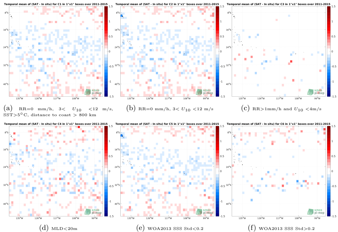
Figure 12: Temporal mean gridded over spatial boxes of size 1^\circ \times 1^\circ of \Delta SSS (Aquarius SSS L3 CAP v5 - Monthly (JPL) - Argo) for 6 different subdatasets corresponding to:RR=0 mm/h, 3 < U_{10} < 12 m/s, SST > 5^\circ\text{C} , distance to coast > 800 km (a), RR=0 mm/h, 3 < U_{10} < 12 m/s (b), RR > 1 mm/h and U_{10} < 4 m/s (c),MLD < 20 m (d),WOA2013 SSS Std < 0.2 (e),WOA2013 SSS Std > 0.2 (f).
