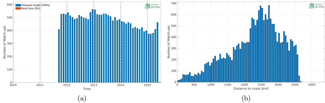
Figure 1: Number of match-ups between Argo and Aquarius SSS L3 CAP v5 - Monthly (JPL) SSS as a function of time (a) and as function of the distance to coast (b) over the OTT zone Pi-MEP region and for the full satellite product period.
