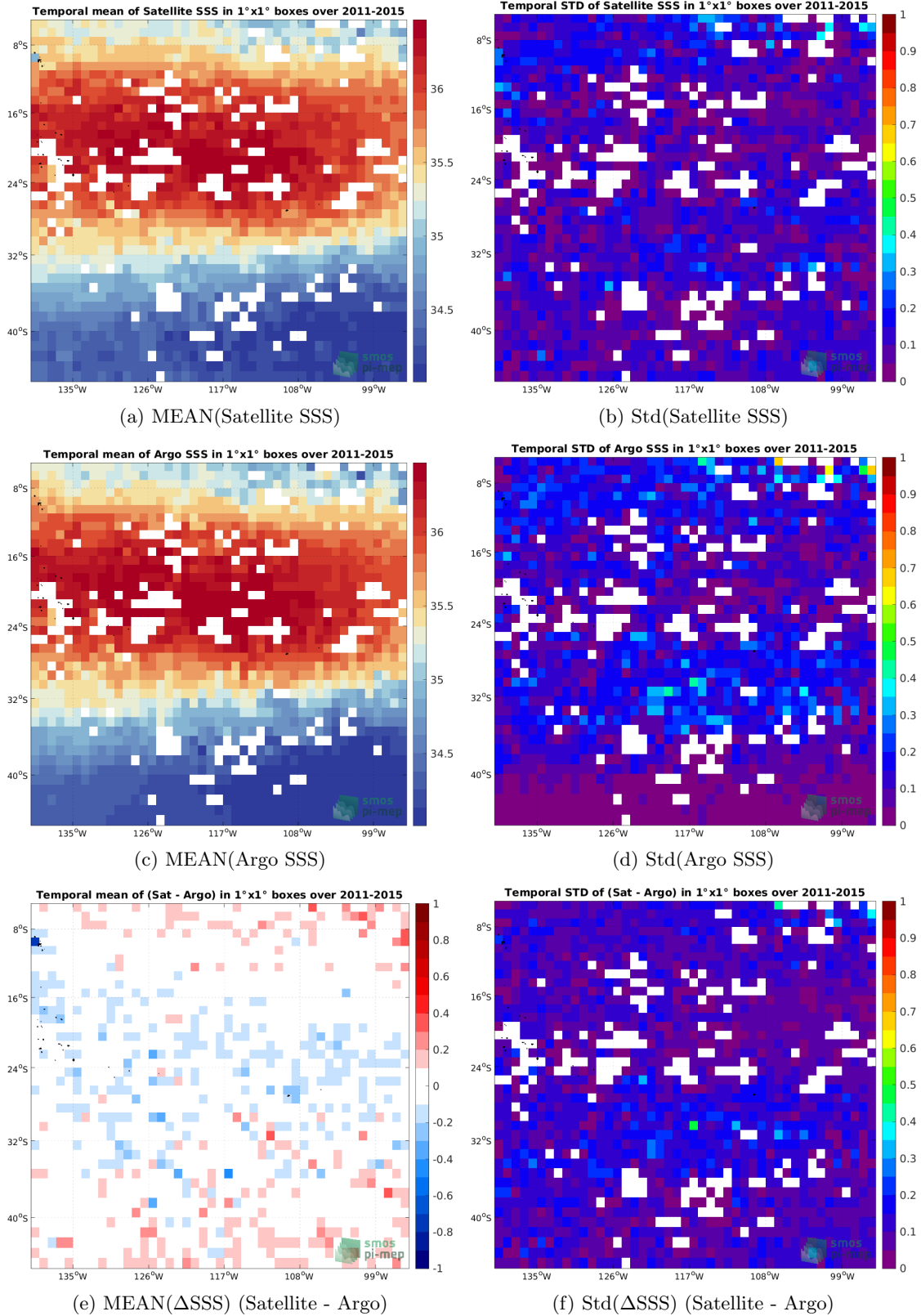
Figure 6: Temporal mean (left) and Std (right) of SSS from Aquarius SSS L3 CAP v5 - Monthly (JPL) (top), Argo (middle), and of \Delta SSS (Satellite - Argo). Only match-up pairs are used to generate these maps.
