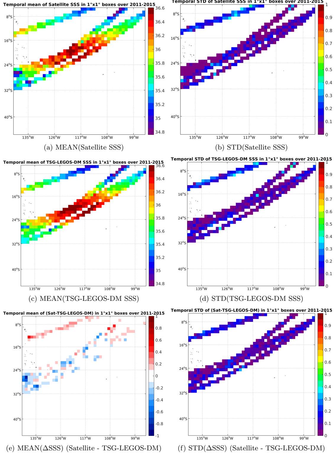
Figure 6: Temporal mean (left) and STD (right) of SSS from Aquarius-L3-JPL-V4-7DAY-RUNNING (top), TSG-LEGOS-DM (middle), and of \Delta SSS (Satellite - TSG-LEGOS-DM). Only match-up pairs are used to generate these maps.
