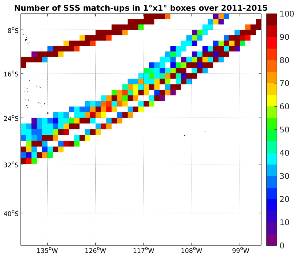
Figure 4: Number of SSS match-ups between TSG-LEGOS-DM SSS and the Aquarius-L3-JPL-V4-7DAY-RUNNING SSS product for the OTT zone Pi-MEP region over 1°x1° boxes and for the full satellite product period.
