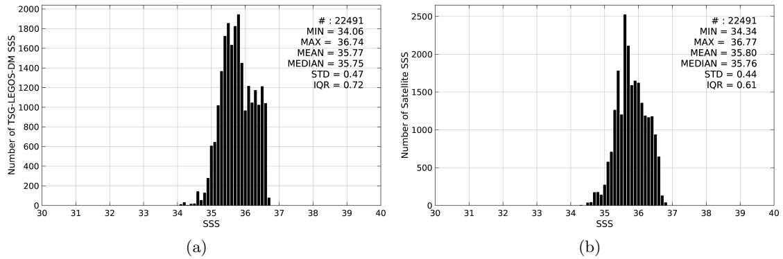
Figure 2: Histograms of SSS from TSG-LEGOS-DM (a) and Aquarius-L3-JPL-V4-7DAY-RUNNING (b) considering all match-up pairs per bins of 0.1 over the OTT zone Pi-MEP region and for the full satellite product period.
