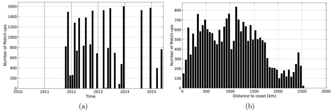
Figure 1: Number of match-ups between TSG-LEGOS-DM and Aquarius-L3-JPL-V4-7DAY-RUNNING SSS as a function of time (a) and as function of the distance to coast (b) over the OTT zone Pi-MEP region and for the full satellite product period.
