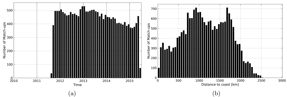
Figure 1: Number of match-ups between Argo and Aquarius-L3-JPL-V4-7DAY-RUNNING SSS as a function of time (a) and as function of the distance to coast (b) over the OTT zone Pi-MEP region and for the full satellite product period.
