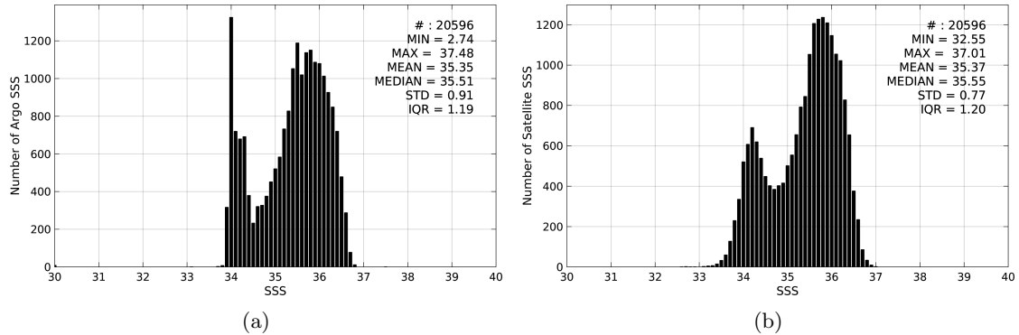
Figure 2: Histograms of SSS from Argo (a) and Aquarius-L3-JPL-V4-7DAY-RUNNING (b) considering all match-up pairs per bins of 0.1 over the OTT zone Pi-MEP region and for the full satellite product period.
