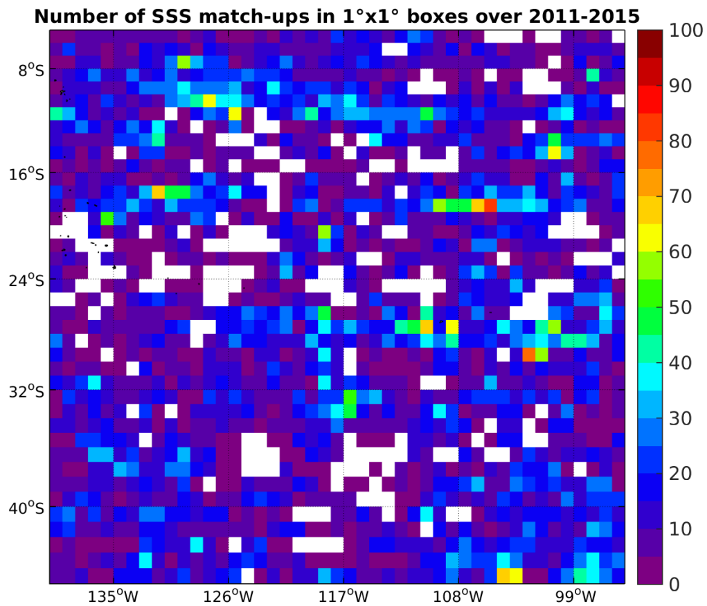
Figure 4: Number of SSS match-ups between Argo SSS and the Aquarius-L3-JPL-V4-7DAY-RUNNING SSS product for the OTT zone Pi-MEP region over 1°x1° boxes and for the full satellite product period.
