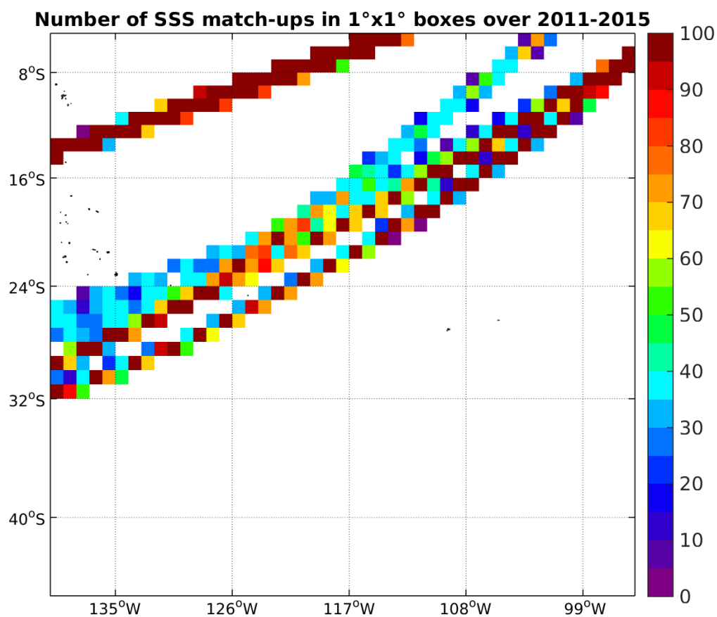
Figure 4: Number of SSS match-ups between TSG-LEGOS-DM SSS and the Aquarius-L3-JPL-V4-MONTHLY SSS product for the OTT zone Pi-MEP region over 1°x1° boxes and for the full satellite product period.
