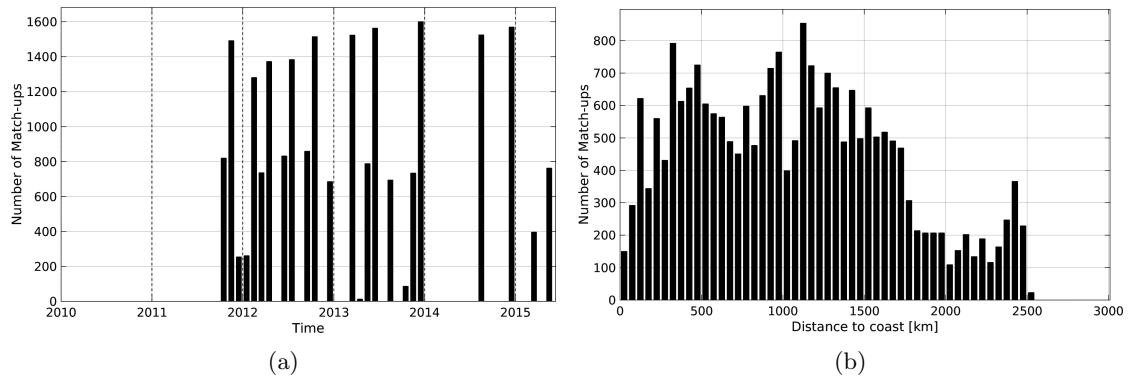
Figure 1: Number of match-ups between TSG-LEGOS-DM and Aquarius-L3-JPL-V4-MONTHLY SSS as a function of time (a) and as function of the distance to coast (b) over the OTT zone Pi-MEP region and for the full satellite product period.
