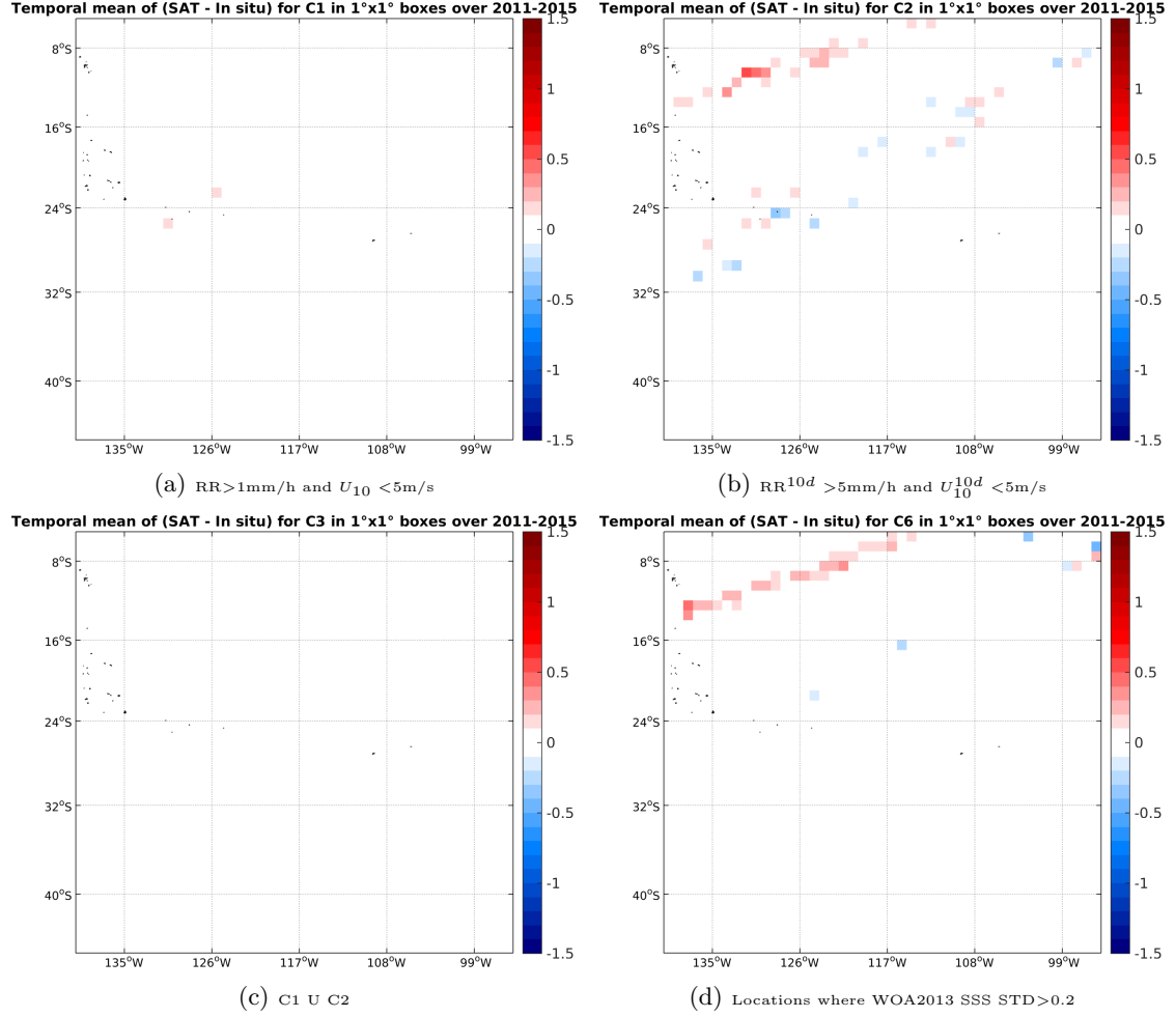
Figure 12: Temporal mean gridded over spatial boxes of size 1^\circ \times 1^\circ of \Delta SSS (Aquarius-L3-JPL-V4-MONTHLY - TSG-LEGOS-DM) for 4 different subdatasets corresponding to: RR > 1mm/h and U_{10} < 5 m/s (a), RR 10d > 5mm/h and U_{10}^{10d} < 5 m/s (b), C1 U C2 (c), Locations where WOA2013 SSS STD > 0.2 (d).
