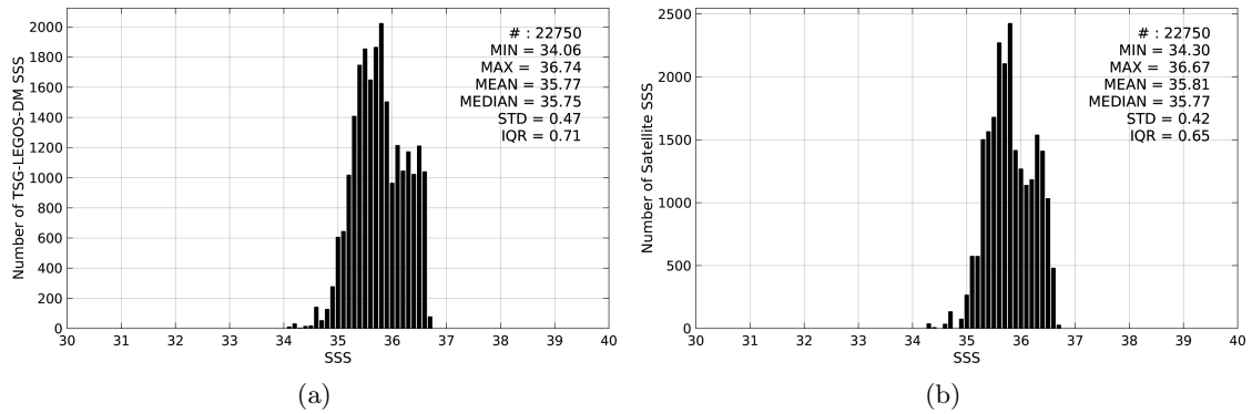
Figure 2: Histograms of SSS from TSG-LEGOS-DM (a) and Aquarius-L3-JPL-V4-MONTHLY (b) considering all match-up pairs per bins of 0.1 over the OTT zone Pi-MEP region and for the full satellite product period.
