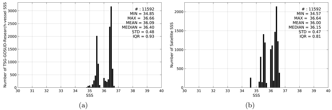
Figure 2: Histograms of SSS from TSG-GOSUD-Research-vessel (a) and Aquarius-L3-JPL-V4-MONTHLY (b) considering all match-up pairs per bins of 0.1 over the OTT zone Pi-MEP region and for the full satellite product period.
