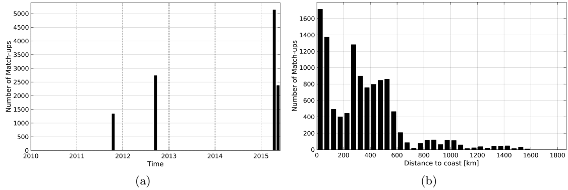
Figure 1: Number of match-ups between TSG-GOSUD-Research-vessel and Aquarius-L3-JPL-V4-MONTHLY SSS as a function of time (a) and as function of the distance to coast (b) over the OTT zone Pi-MEP region and for the full satellite product period.
