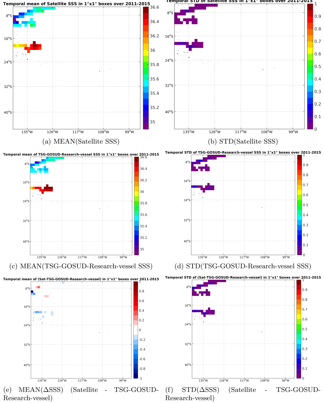
Figure 6: Temporal mean (left) and STD (right) of SSS from Aquarius-L3-JPL-V4-MONTHLY (top), TSG-GOSUD-Research-vessel (middle), and of \Delta SSS (Satellite - TSG-GOSUD-Research-vessel). Only match-up pairs are used to generate these maps.
