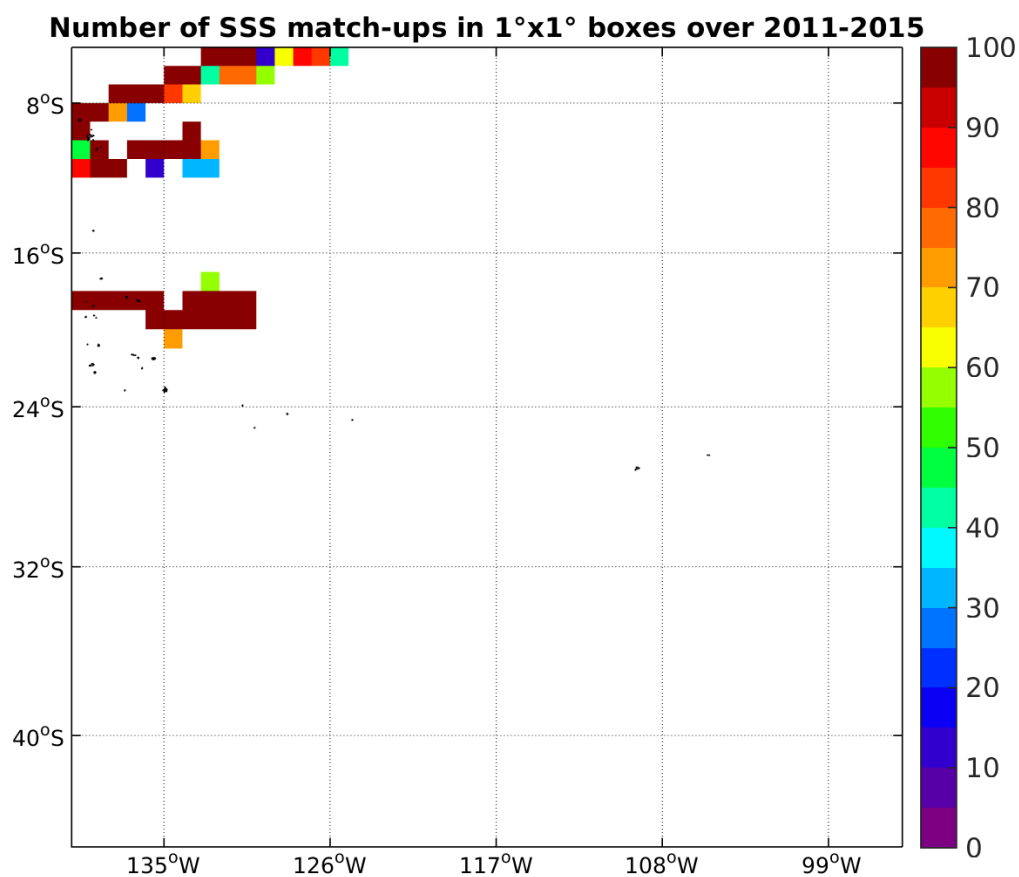
Figure 4: Number of SSS match-ups between TSG-GOSUD-Research-vessel SSS and the Aquarius-L3-JPL-V4-MONTHLY SSS product for the OTT zone Pi-MEP region over 1°x1° boxes and for the full satellite product period.
