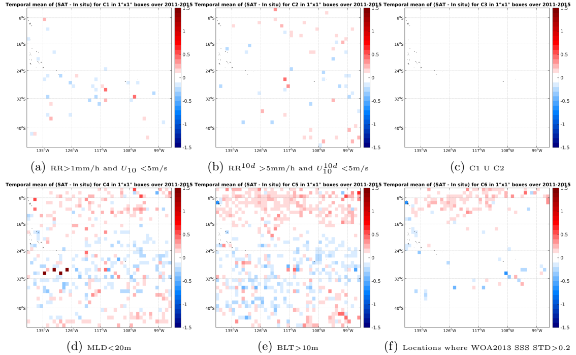
Figure 12: Temporal mean gridded over spatial boxes of size 1^\circ \times 1^\circ of \Delta SSS (Aquarius-L3-JPL-V4-MONTHLY - Argo) for 6 different subdatasets corresponding to: RR > 1mm/h and U_{10} < 5\text{m/s} (a), RR^{10d} > 5\text{mm/h} and U_{10}^{10d} < 5\text{m/s} (b), C1 U C2 (c), MLD < 20m (d), BLT > 10m (e), Locations where WOA2013 SSS STD > 0.2 (f).
