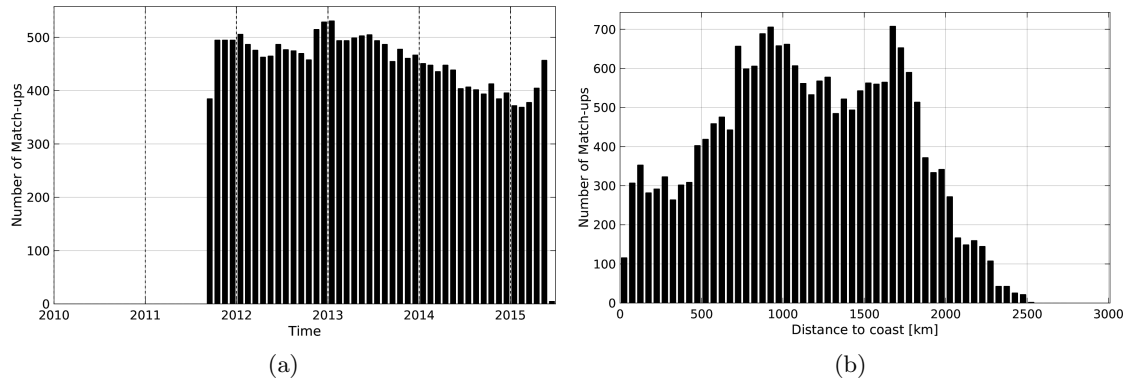
Figure 1: Number of match-ups between Argo and Aquarius-L3-JPL-V4-MONTHLY SSS as a function of time (a) and as function of the distance to coast (b) over the OTT zone Pi-MEP region and for the full satellite product period.
