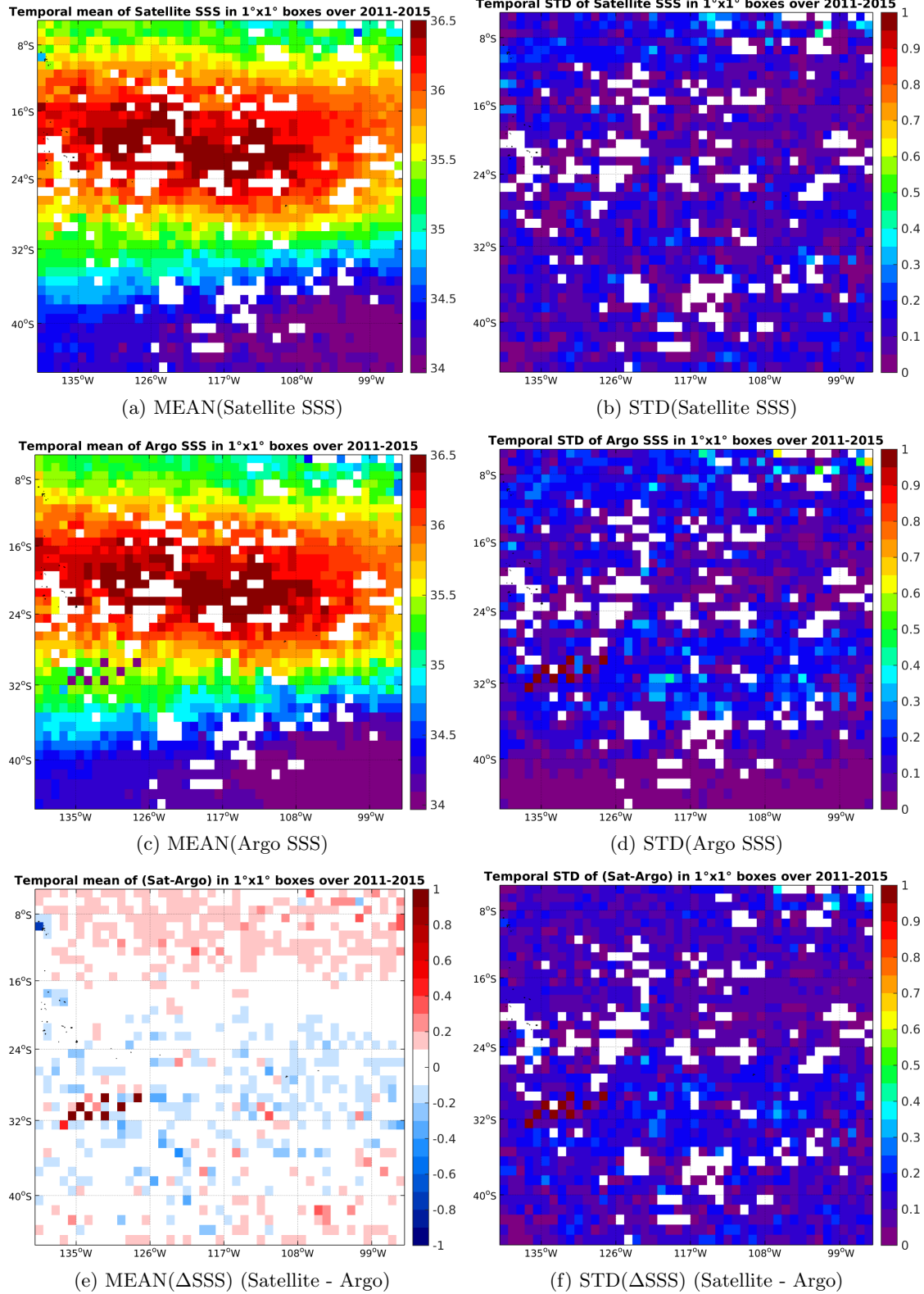
Figure 6: Temporal mean (left) and STD (right) of SSS from Aquarius-L3-JPL-V4-MONTHLY (top), Argo (middle), and of \Delta SSS (Satellite - Argo). Only match-up pairs are used to generate these maps.
