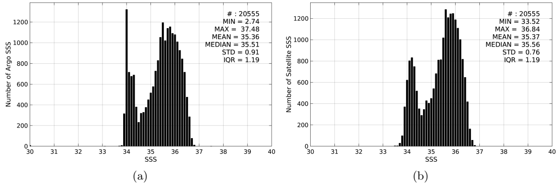
Figure 2: Histograms of SSS from Argo (a) and Aquarius-L3-JPL-V4-MONTHLY (b) considering all match-up pairs per bins of 0.1 over the OTT zone Pi-MEP region and for the full satellite product period.
