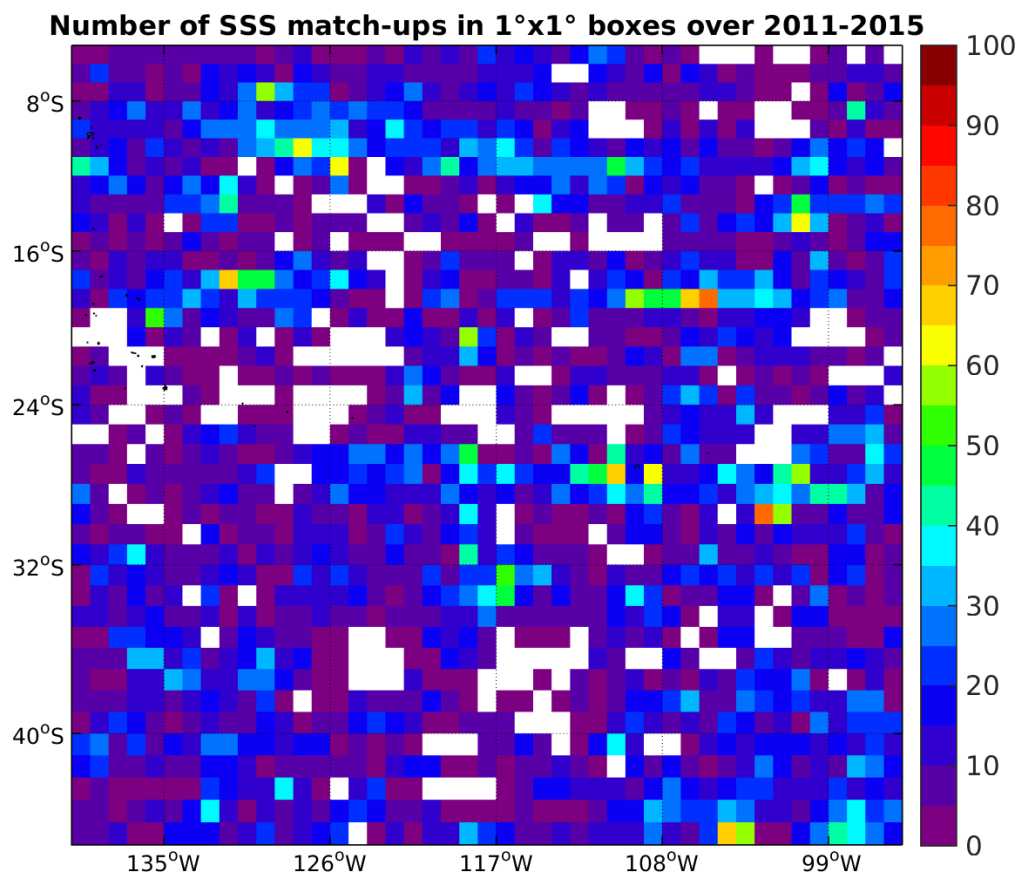
Figure 4: Number of SSS match-ups between Argo SSS and the Aquarius-L3-JPL-V4-MONTHLY SSS product for the OTT zone Pi-MEP region over 1°x1° boxes and for the full satellite product period.
