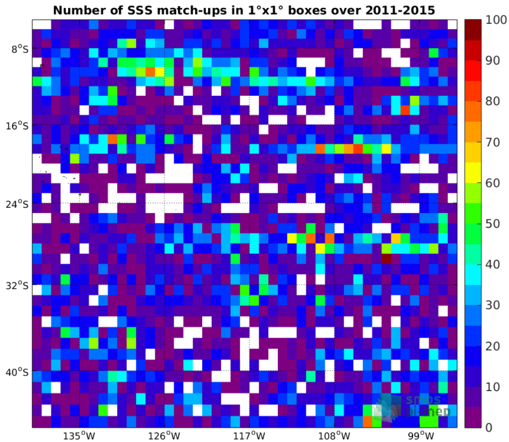
Figure 4: Number of SSS match-ups between Argo SSS and the Aquarius SSS L2-AVERAGED OR v5 (NASA-GSFC) SSS product for the OTT zone Pi-MEP region over 1°x1° boxes and for the full satellite product period.
