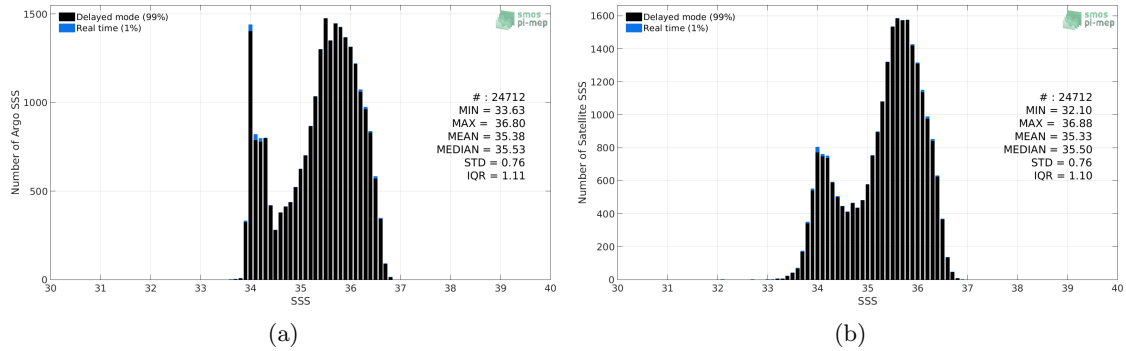
Figure 2: Histograms of SSS from Argo (a) and Aquarius SSS L2-AVERAGED OR v5 (NASA-GSFC) (b) considering all match-up pairs per bins of 0.1 over the OTT zone Pi-MEP region and for the full satellite product period.
