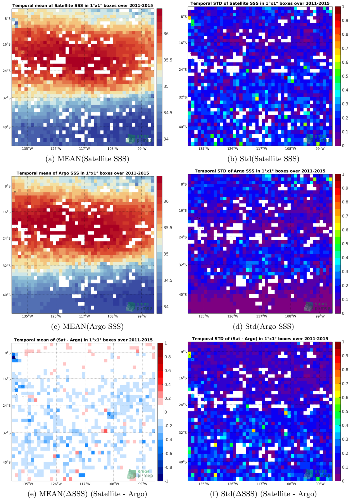
Figure 6: Temporal mean (left) and Std (right) of SSS from Aquarius SSS L2-AVERAGED OR v5 (NASA-GSFC) (top), Argo (middle), and of \Delta SSS (Satellite - Argo). Only match-up pairs are used to generate these maps.
