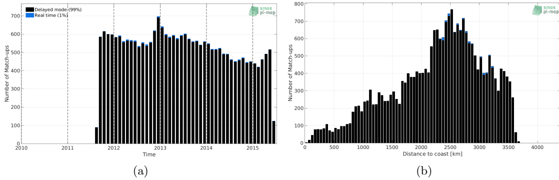
Figure 1: Number of match-ups between Argo and Aquarius SSS L2-AVERAGED OR v5 (NASA-GSFC) SSS as a function of time (a) and as function of the distance to coast (b) over the OTT zone Pi-MEP region and for the full satellite product period.
