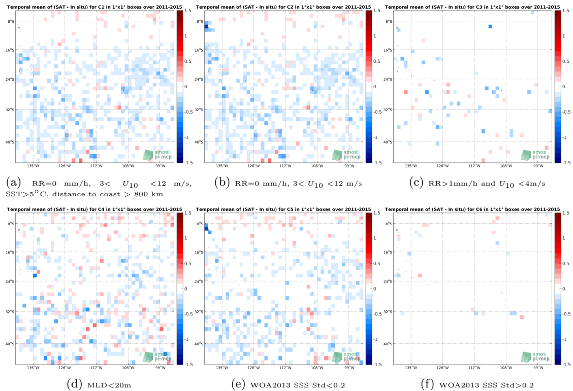
Figure 12: Temporal mean gridded over spatial boxes of size 1^\circ \times 1^\circ of \Delta SSS (Aquarius SSS L2-AVERAGED OR v5 (NASA-GSFC) - Argo) for 6 different subdatasets corresponding to:RR=0 mm/h, 3 < U_{10} < 12 m/s, SST >5^\circ C, distance to coast > 800 km (a), RR=0 mm/h, 3 < U_{10} < 12 m/s (b), RR >1 mm/h and U_{10} < 4 m/s (c),MLD <20 m (d),WOA2013 SSS Std <0.2 (e),WOA2013 SSS Std >0.2 (f).
