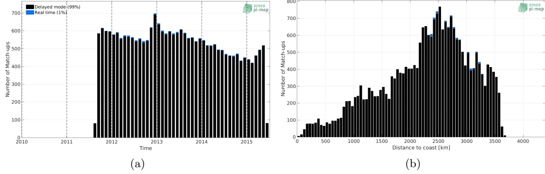
Figure 1: Number of match-ups between Argo and Aquarius SSS L2-AVERAGED CAP v5 (JPL) SSS as a function of time (a) and as function of the distance to coast (b) over the OTT zone Pi-MEP region and for the full satellite product period.
