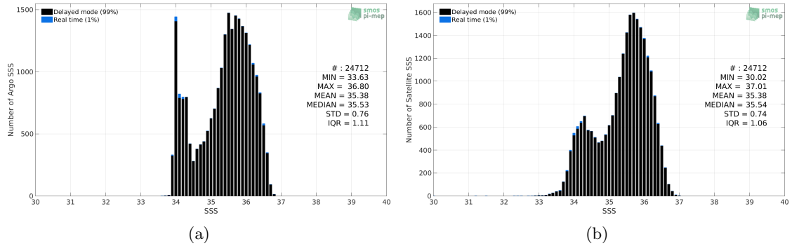
Figure 2: Histograms of SSS from Argo (a) and Aquarius SSS L2-AVERAGED CAP v5 (JPL) (b) considering all match-up pairs per bins of 0.1 over the OTT zone Pi-MEP region and for the full satellite product period.
