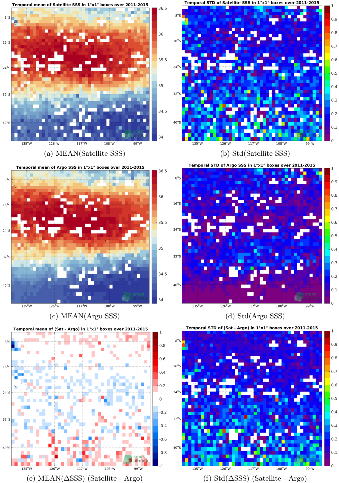
Figure 6: Temporal mean (left) and Std (right) of SSS from Aquarius SSS L2-AVERAGED CAP v5 (JPL) (top), Argo (middle), and of \Delta SSS (Satellite - Argo). Only match-up pairs are used to generate these maps.
