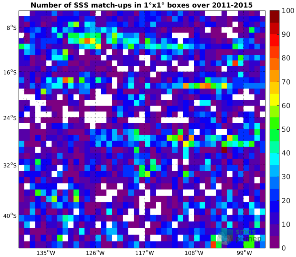
Figure 4: Number of SSS match-ups between Argo SSS and the Aquarius SSS L2-AVERAGED CAP v5 (JPL) SSS product for the OTT zone Pi-MEP region over 1°x1° boxes and for the full satellite product period.
