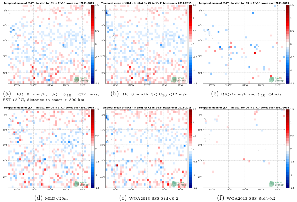
Figure 12: Temporal mean gridded over spatial boxes of size 1^\circ \times 1^\circ of \Delta SSS (Aquarius SSS L2-AVERAGED CAP v5 (JPL) - Argo) for 6 different subdatasets corresponding to:RR=0 mm/h, 3 < U_{10} < 12 m/s, SST > 5^\circ\text{C} , distance to coast > 800 km (a), RR=0 mm/h, 3 < U_{10} < 12 m/s (b), RR > 1 mm/h and U_{10} < 4 m/s (c),MLD < 20 m (d),WOA2013 SSS Std < 0.2 (e),WOA2013 SSS Std > 0.2 (f).
