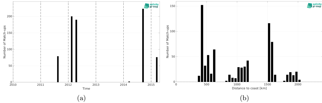
Figure 2: Number of match-ups between TSG (SAMOS) and Aquarius SSS L2 OR v5 (NASA-GSFC) SSS as a function of time (a) and as function of the distance to coast (b) over the OTT zone Pi-MEP region and for the full satellite product period.
