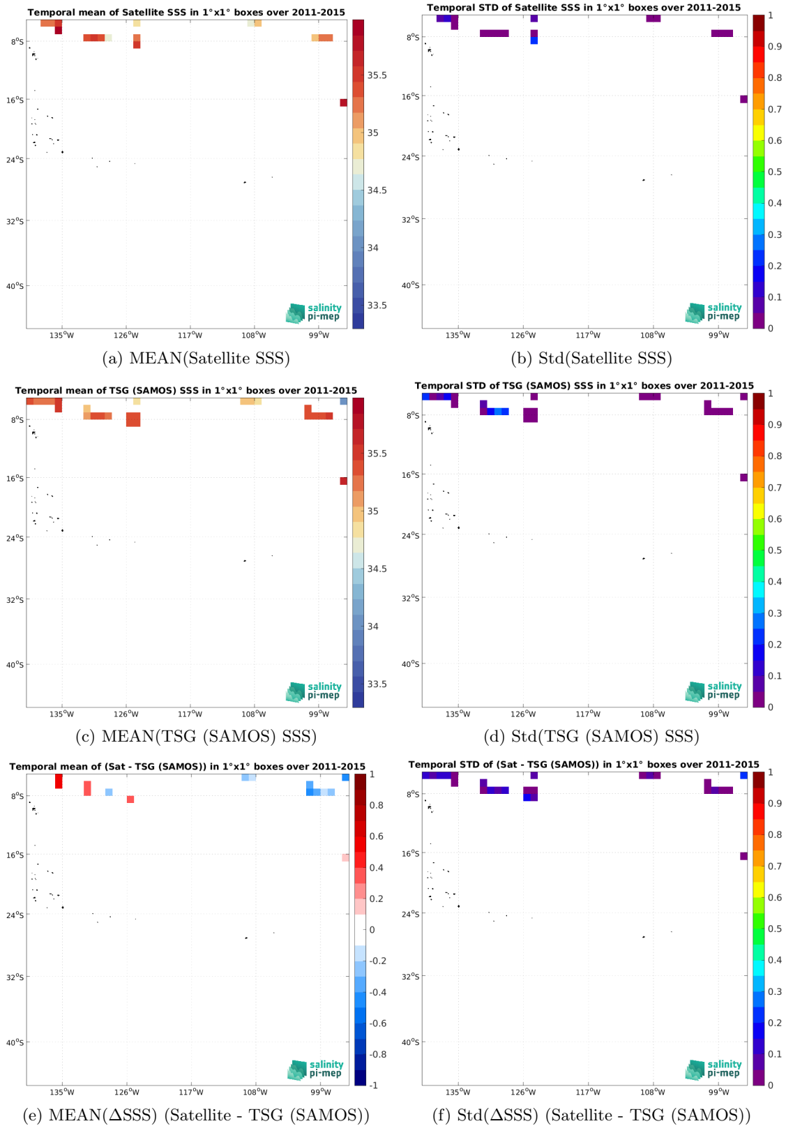
Figure 7: Temporal mean (left) and Std (right) of SSS from Aquarius SSS L2 OR v5 (NASA-GSFC) (top), TSG (SAMOS) (middle), and of \Delta SSS (Satellite - TSG (SAMOS)). Only match-up pairs are used to generate these maps.
