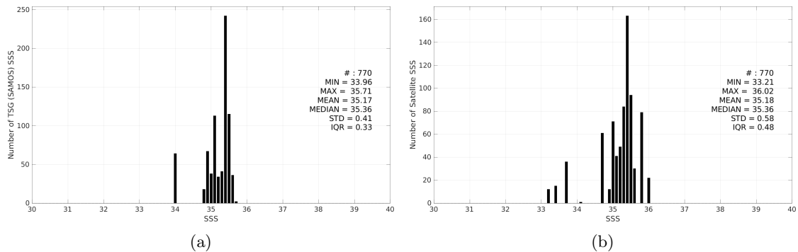
Figure 3: Histograms of SSS from TSG (SAMOS) (a) and Aquarius SSS L2 OR v5 (NASA-GSFC) (b) considering all match-up pairs per bins of 0.1 over the OTT zone Pi-MEP region and for the full satellite product period.
