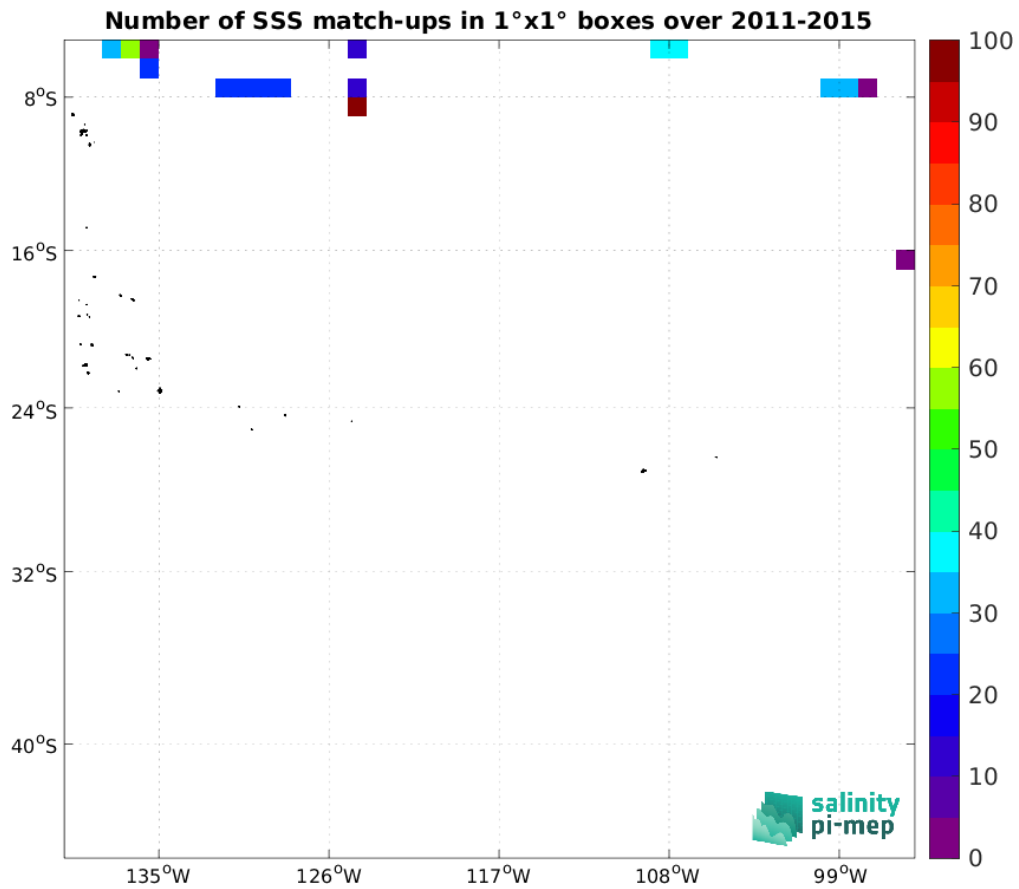
Figure 5: Number of SSS match-ups between TSG (SAMOS) SSS and the Aquarius SSS L2 OR v5 (NASA-GSFC) SSS product for the OTT zone Pi-MEP region over 1^\circ \times 1^\circ boxes and for the full satellite product period.
