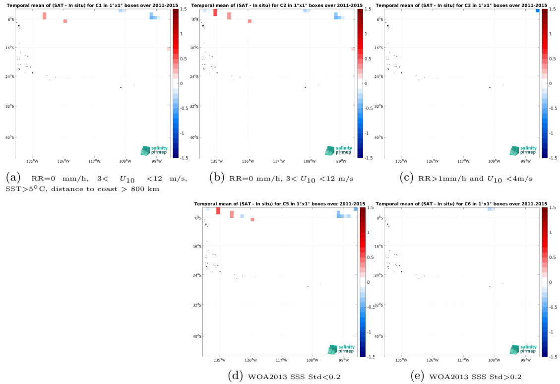
Figure 12: Temporal mean gridded over spatial boxes of size 1^\circ \times 1^\circ of \Delta SSS (Aquarius SSS L2 OR v5 (NASA-GSFC) - TSG (SAMOS)) for 5 different subdatasets corresponding to: RR=0 mm/h, 3 < U_{10} < 12 m/s, SST > 5^\circ C , distance to coast > 800 km (a), RR=0 mm/h, 3 < U_{10} < 12 m/s (b), RR > 1 mm/h and U_{10} < 4 m/s (c), WOA2013 SSS Std < 0.2 (d), WOA2013 SSS Std > 0.2 (e).
