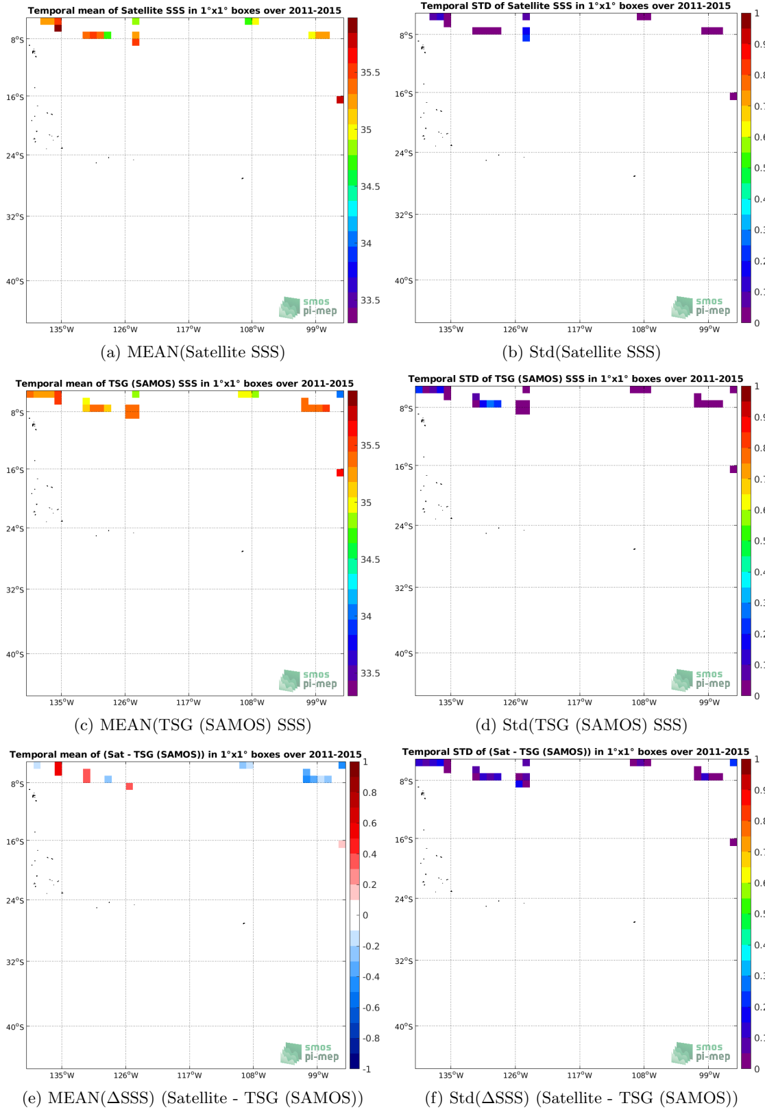
Figure 6: Temporal mean (left) and Std (right) of SSS from Aquarius SSS L2 OR v5 (NASA-GSFC) (top), TSG (SAMOS) (middle), and of \Delta SSS (Satellite - TSG (SAMOS)). Only match-up pairs are used to generate these maps.
