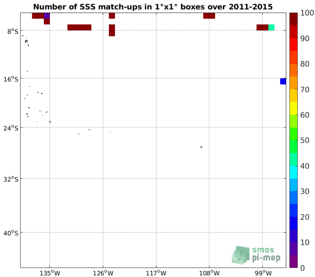
Figure 4: Number of SSS match-ups between TSG (SAMOS) SSS and the Aquarius SSS L2 OR v5 (NASA-GSFC) SSS product for the OTT zone Pi-MEP region over 1°×1° boxes and for the full satellite product period.
