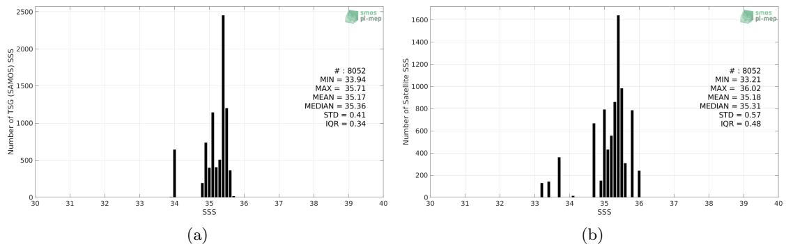
Figure 2: Histograms of SSS from TSG (SAMOS) (a) and Aquarius SSS L2 OR v5 (NASA-GSFC) (b) considering all match-up pairs per bins of 0.1 over the OTT zone Pi-MEP region and for the full satellite product period.
