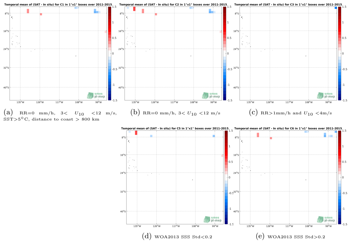
Figure 12: Temporal mean gridded over spatial boxes of size 1^\circ \times 1^\circ of \Delta\text{SSS} (Aquarius SSS L2 OR v5 (NASA-GSFC) - TSG (SAMOS)) for 5 different subdatasets corresponding to:RR=0 mm/h, 3 < U_{10} < 12 m/s, SST >5^\circ\text{C} , distance to coast > 800 km (a), RR=0 mm/h, 3 < U_{10} < 12 m/s (b), RR >1 mm/h and U_{10} < 4 m/s (c), WOA2013 SSS Std <0.2 (d), WOA2013 SSS Std >0.2 (e).
