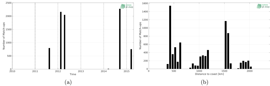
Figure 1: Number of match-ups between TSG (SAMOS) and Aquarius SSS L2 OR v5 (NASA-GSFC) SSS as a function of time (a) and as function of the distance to coast (b) over the OTT zone Pi-MEP region and for the full satellite product period.
