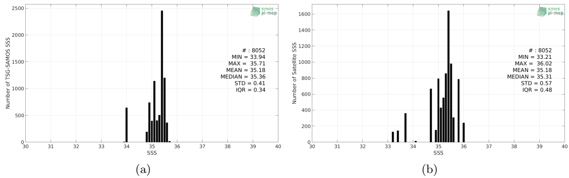
Figure 2: Histograms of SSS from TSG-SAMOS (a) and Aquarius-L2-OR-V5 (b) considering all match-up pairs per bins of 0.1 over the OTT zone Pi-MEP region and for the full satellite product period.
