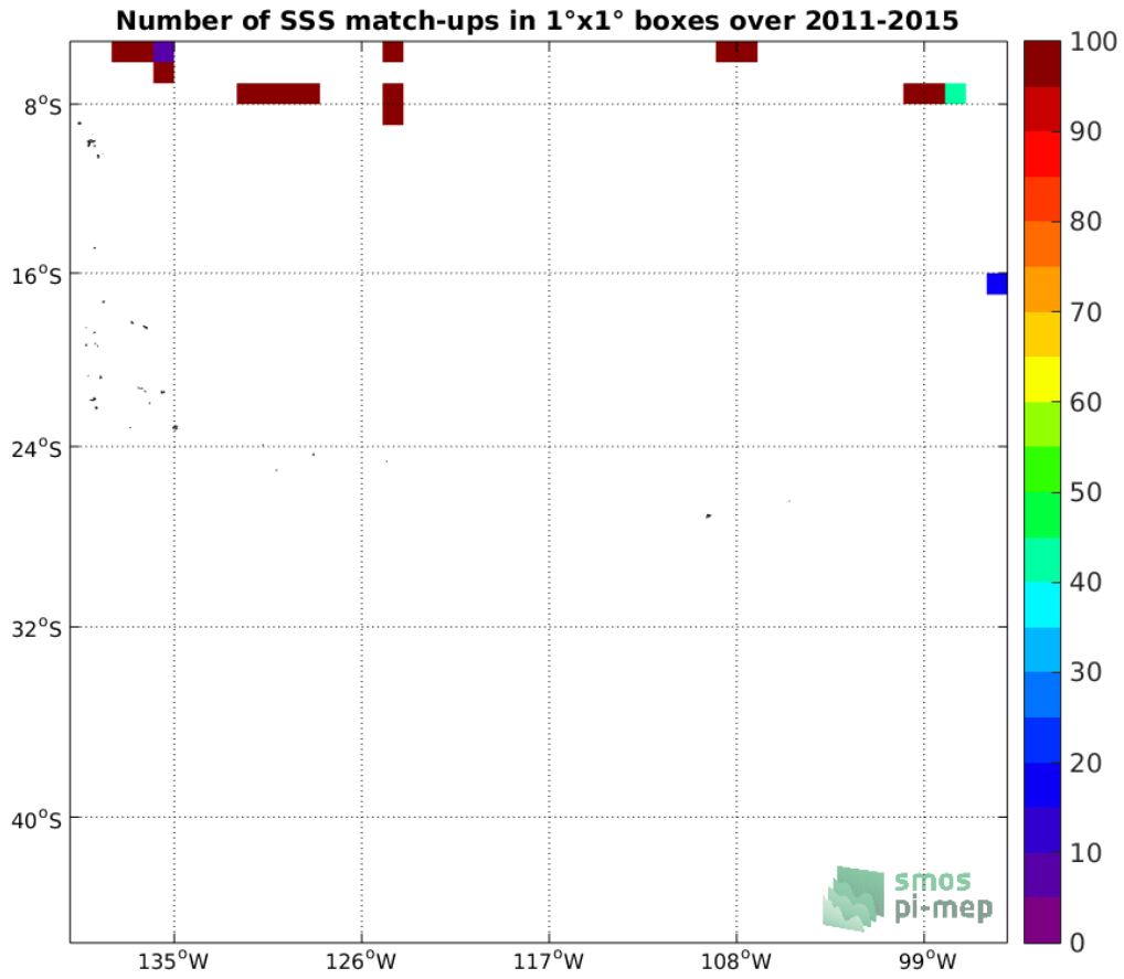
Figure 4: Number of SSS match-ups between TSG-SAMOS SSS and the Aquarius-L2-OR-V5 SSS product for the OTT zone Pi-MEP region over 1°x1° boxes and for the full satellite product period.
