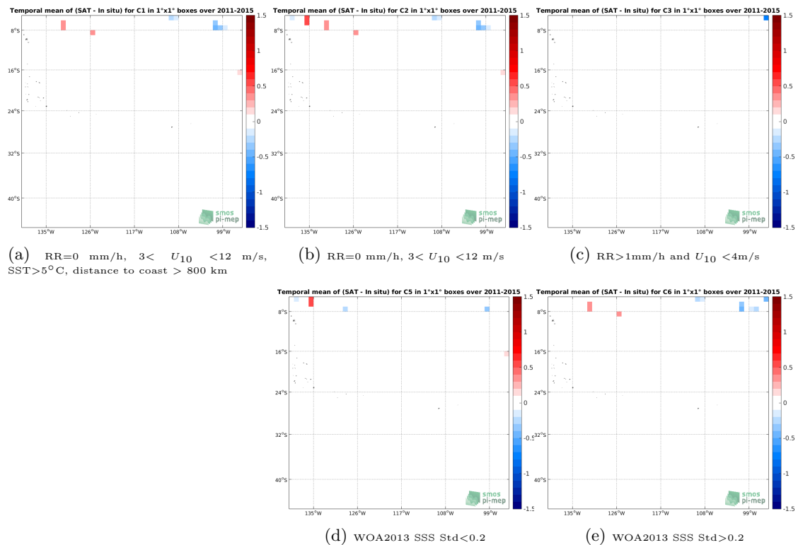
Figure 12: Temporal mean gridded over spatial boxes of size 1^\circ \times 1^\circ of \Delta SSS (Aquarius-L2-OR-V5 - TSG-SAMOS) for 5 different subdatasets corresponding to:RR=0 mm/h, 3 < U_{10} < 12 m/s, SST >5^\circ C, distance to coast > 800 km (a), RR=0 mm/h, 3 < U_{10} < 12 m/s (b), RR >1 mm/h and U_{10} < 4 m/s (c), WOA2013 SSS Std <0.2 (d), WOA2013 SSS Std >0.2 (e).
