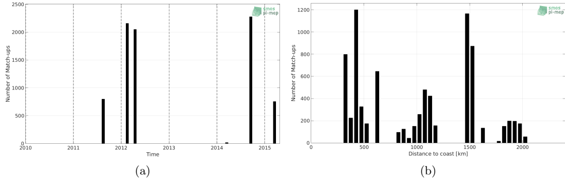
Figure 1: Number of match-ups between TSG-SAMOS and Aquarius-L2-OR-V5 SSS as a function of time (a) and as function of the distance to coast (b) over the OTT zone Pi-MEP region and for the full satellite product period.
