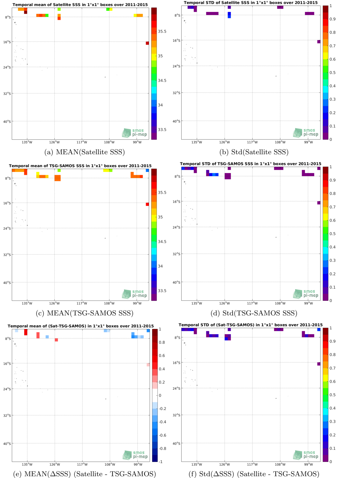
Figure 6: Temporal mean (left) and Std (right) of SSS from Aquarius-L2-OR-V5 (top), TSG-SAMOS (middle), and of \Delta SSS (Satellite - TSG-SAMOS). Only match-up pairs are used to generate these maps.
