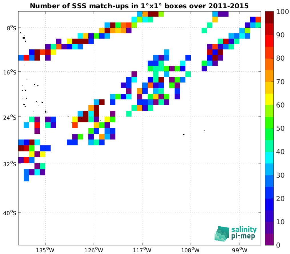
Figure 4: Number of SSS match-ups between TSG (LEGOS-DM) SSS and the Aquarius SSS L2 OR v5 (NASA-GSFC) SSS product for the OTT zone Pi-MEP region over 1°x1° boxes and for the full satellite product period.
