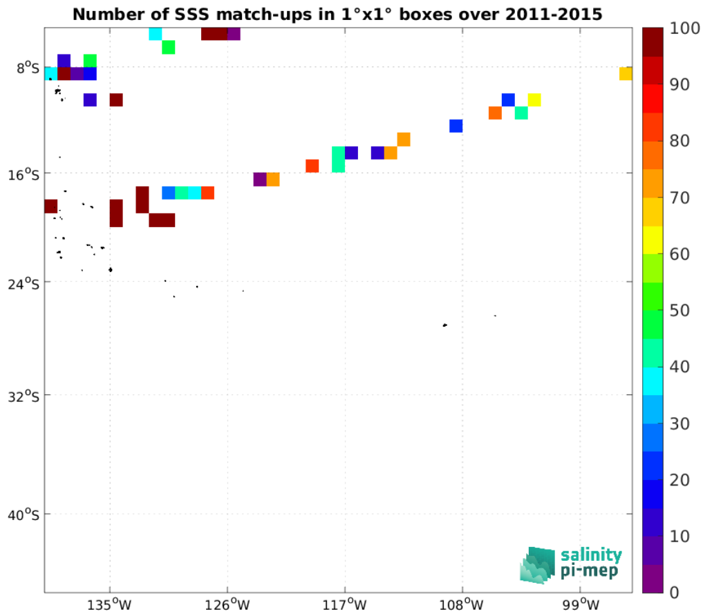
Figure 4: Number of SSS match-ups between TSG (GOSUD-Research-vessel) SSS and the Aquarius SSS L2 OR v5 (NASA-GSFC) SSS product for the OTT zone Pi-MEP region over 1^\circ \times 1^\circ boxes and for the full satellite product period.
