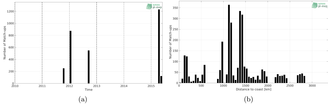
Figure 1: Number of match-ups between TSG (GOSUD-Research-vessel) and Aquarius SSS L2 OR v5 (NASA-GSFC) SSS as a function of time (a) and as function of the distance to coast (b) over the OTT zone Pi-MEP region and for the full satellite product period.
