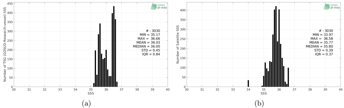
Figure 2: Histograms of SSS from TSG (GOSUD-Research-vessel) (a) and Aquarius SSS L2 OR v5 (NASA-GSFC) (b) considering all match-up pairs per bins of 0.1 over the OTT zone Pi-MEP region and for the full satellite product period.
