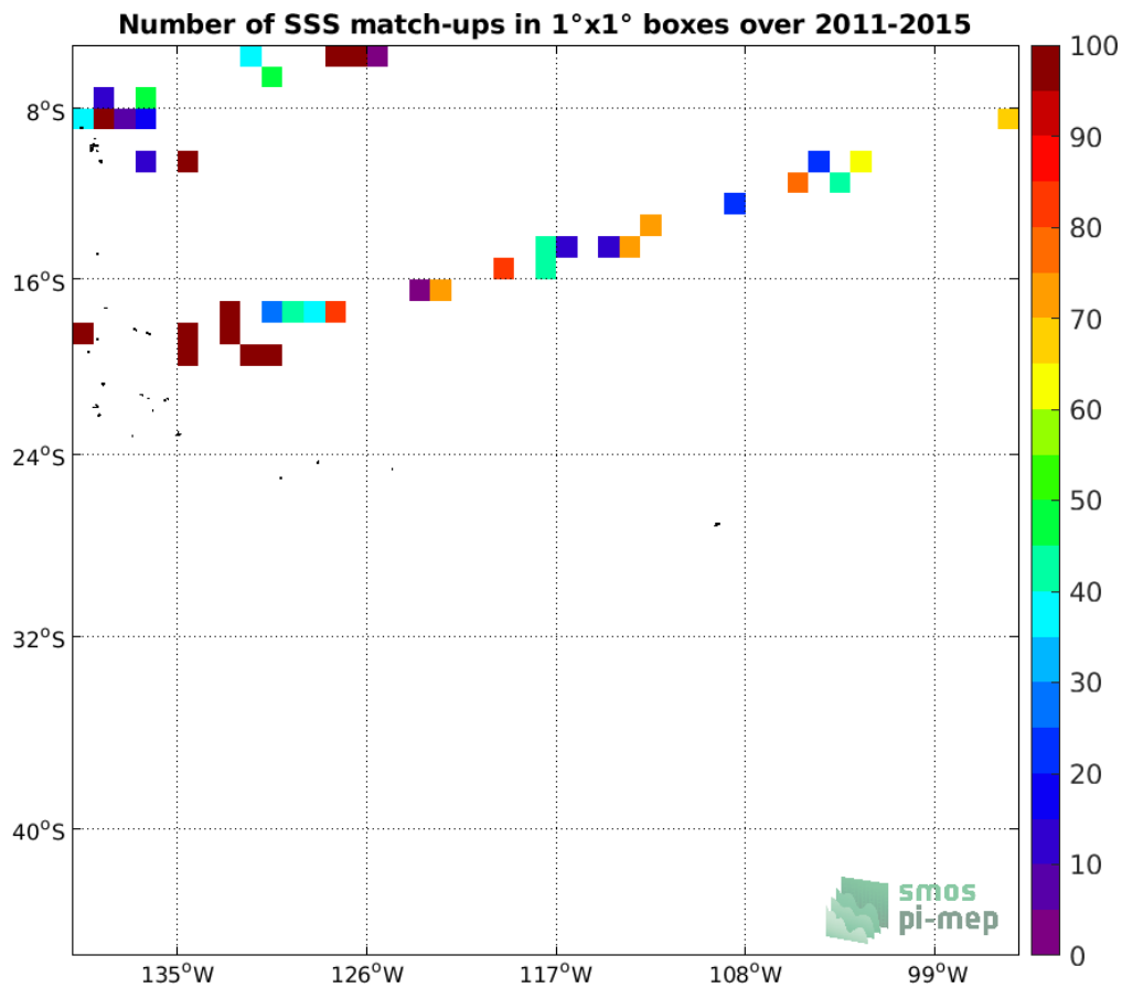
Figure 4: Number of SSS match-ups between TSG (GOSUD-Research-vessel) SSS and the Aquarius SSS L2 OR v5 (NASA-GSFC) SSS product for the OTT zone Pi-MEP region over 1°x1° boxes and for the full satellite product period.
