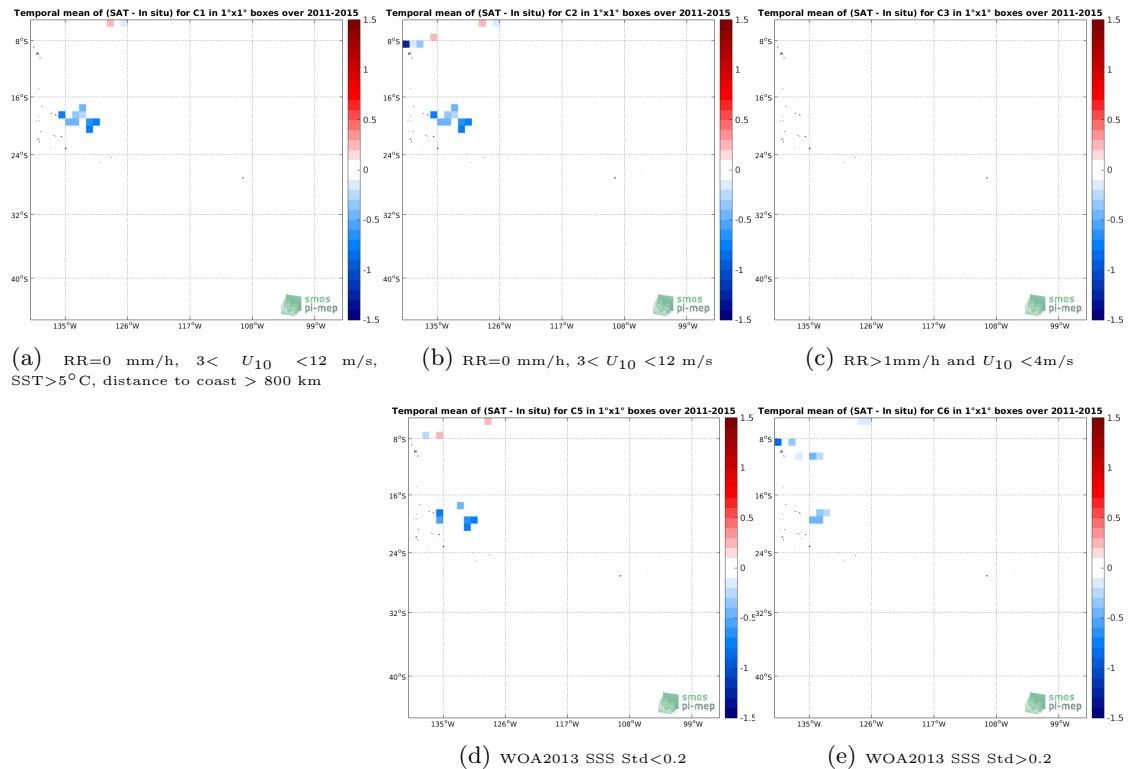
Figure 12: Temporal mean gridded over spatial boxes of size 1^\circ \times 1^\circ of \Delta SSS (Aquarius-L2-OR-V5 - TSG-GOSUD-Research-vessel) for 5 different subdatasets corresponding to:RR=0 mm/h, 3 < U_{10} < 12 m/s, SST > 5^\circ\text{C} , distance to coast > 800 km (a), RR=0 mm/h, 3 < U_{10} < 12 m/s (b), RR > 1 mm/h and U_{10} < 4 m/s (c), WOA2013 SSS Std < 0.2 (d), WOA2013 SSS Std > 0.2 (e).
