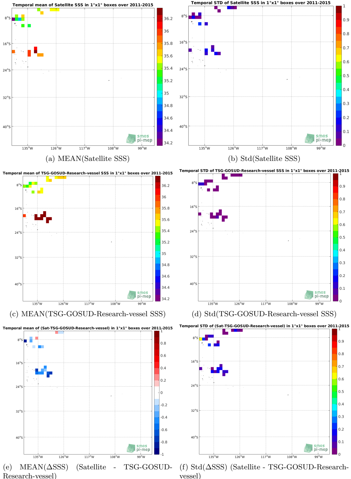
Figure 6: Temporal mean (left) and Std (right) of SSS from Aquarius-L2-OR-V5 (top), TSG-GOSUD-Research-vessel (middle), and of \Delta SSS (Satellite - TSG-GOSUD-Research-vessel). Only match-up pairs are used to generate these maps
