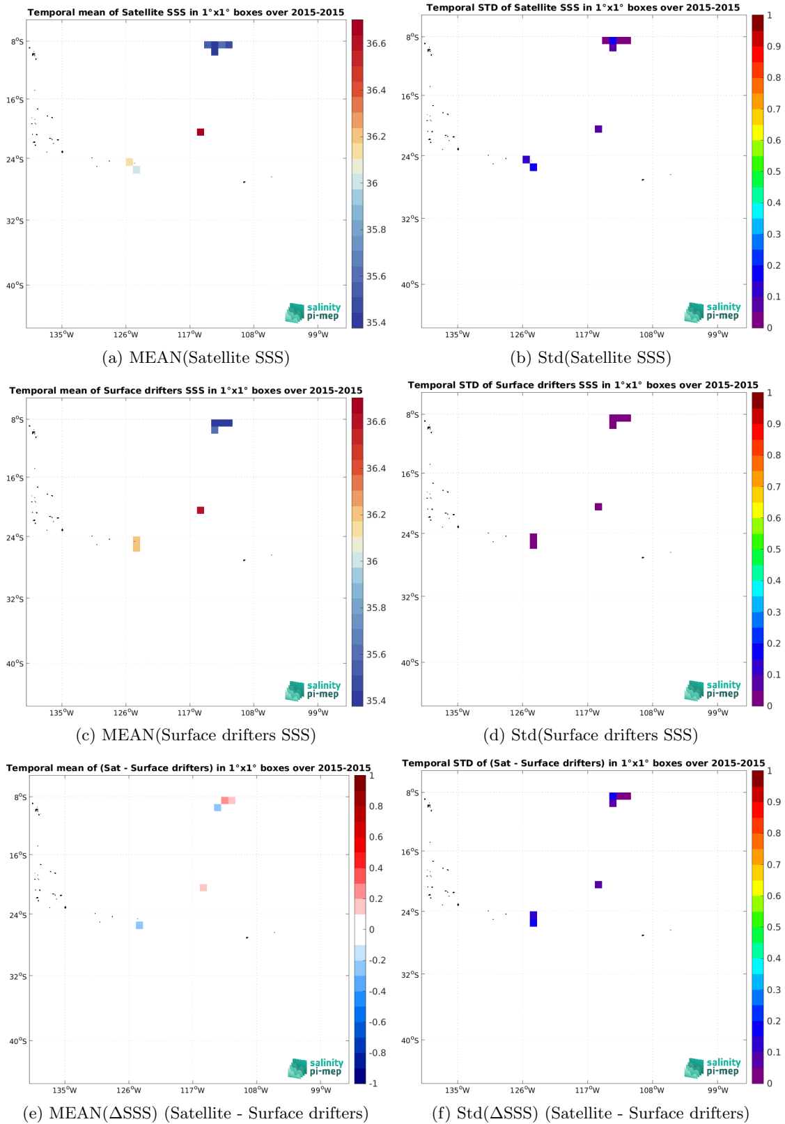
Figure 6: Temporal mean (left) and Std (right) of SSS from Aquarius SSS L2 OR v5 (NASA-GSFC) (top), Surface drifters (middle), and of \Delta SSS (Satellite - Surface drifters). Only match-up pairs are used to generate these maps.
