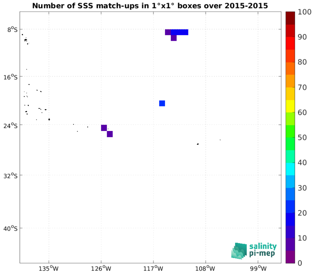
Figure 4: Number of SSS match-ups between Surface drifters SSS and the Aquarius SSS L2 OR v5 (NASA-GSFC) SSS product for the OTT zone Pi-MEP region over 1^\circ \times 1^\circ boxes and for the full satellite product period.
