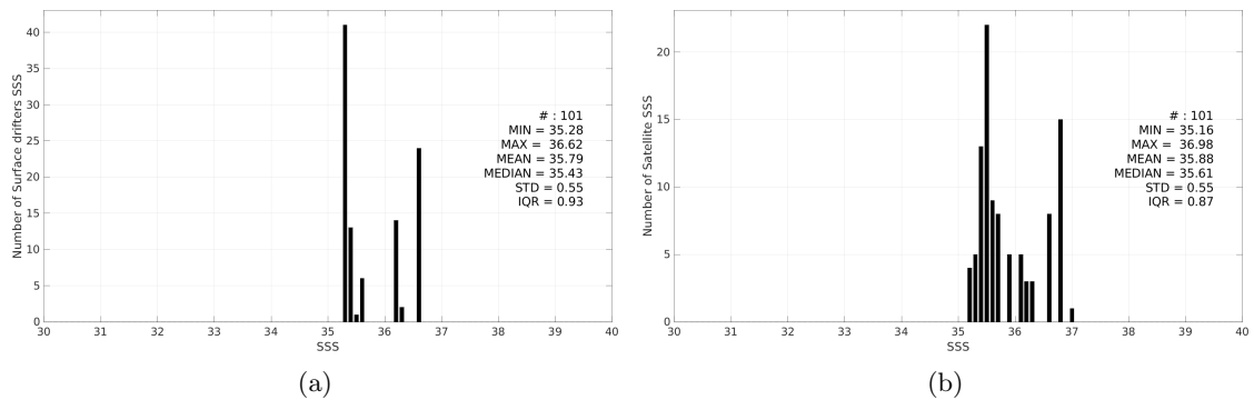
Figure 3: Histograms of SSS from Surface drifters (a) and Aquarius SSS L2 OR v5 (NASA-GSFC) (b) considering all match-up pairs per bins of 0.1 over the OTT zone Pi-MEP region and for the full satellite product period.
