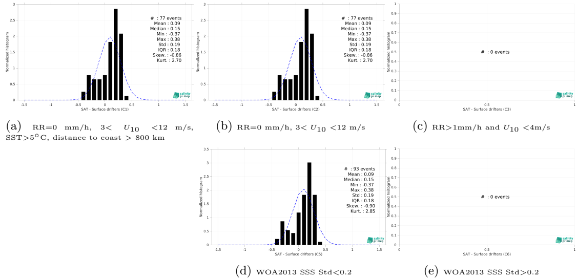
Figure 14: Normalized histogram of \Delta SSS (Aquarius SSS L2 OR v5 (NASA-GSFC) - Surface drifters) for 5 different subdatasets corresponding to: RR=0 mm/h, 3 < U_{10} < 12 m/s, SST > 5°C, distance to coast > 800 km (a), RR=0 mm/h, 3 < U_{10} < 12 m/s (b), RR > 1mm/h and U_{10} < 4 m/s (c), WOA2013 SSS Std < 0.2 (d), WOA2013 SSS Std > 0.2 (e).
