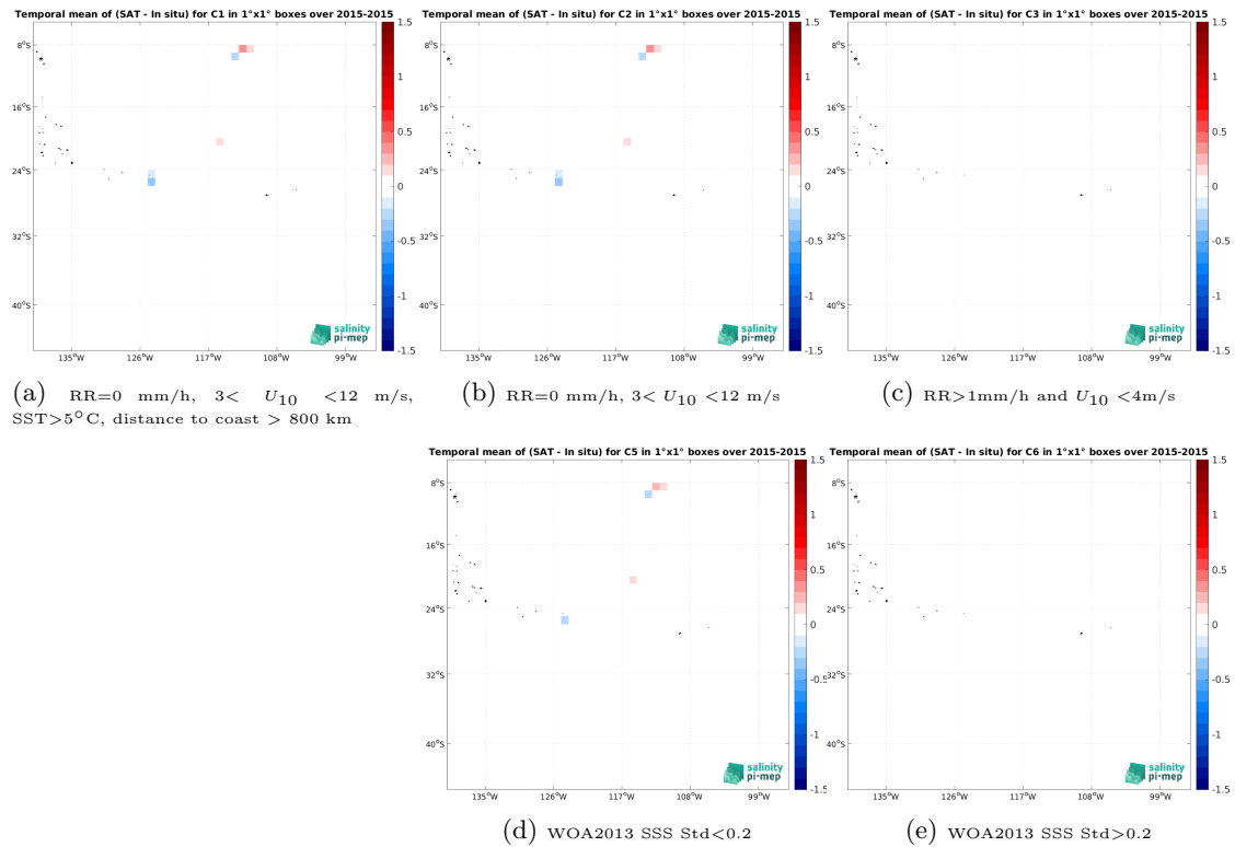
Figure 13: Temporal mean gridded over spatial boxes of size 1^\circ \times 1^\circ of \Delta SSS (Aquarius SSS L2 OR v5 (NASA-GSFC) - Surface drifters) for 5 different subdatasets corresponding to: RR=0 mm/h, 3 < U_{10} < 12 m/s, SST > 5^\circ C , distance to coast > 800 km (a), RR=0 mm/h, 3 < U_{10} < 12 m/s (b), RR > 1 mm/h and U_{10} < 4 m/s (c), WOA2013 SSS Std < 0.2 (d), WOA2013 SSS Std > 0.2 (e).
