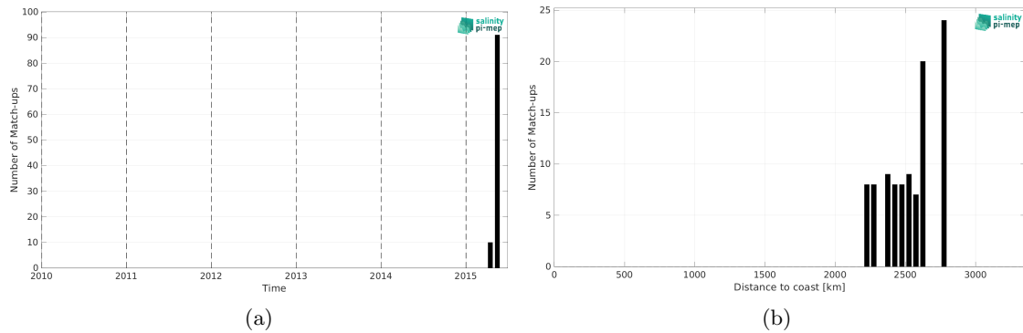
Figure 2: Number of match-ups between Surface drifters and Aquarius SSS L2 OR v5 (NASA-GSFC) SSS as a function of time (a) and as function of the distance to coast (b) over the OTT zone Pi-MEP region and for the full satellite product period.
