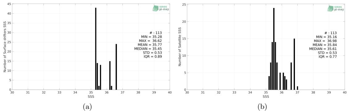
Figure 2: Histograms of SSS from Surface drifters (a) and Aquarius SSS L2 OR v5 (NASA-GSFC) (b) considering all match-up pairs per bins of 0.1 over the OTT zone Pi-MEP region and for the full satellite product period.
