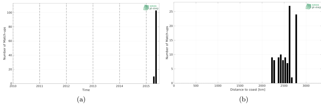
Figure 1: Number of match-ups between Surface drifters and Aquarius SSS L2 OR v5 (NASA-GSFC) SSS as a function of time (a) and as function of the distance to coast (b) over the OTT zone Pi-MEP region and for the full satellite product period.
