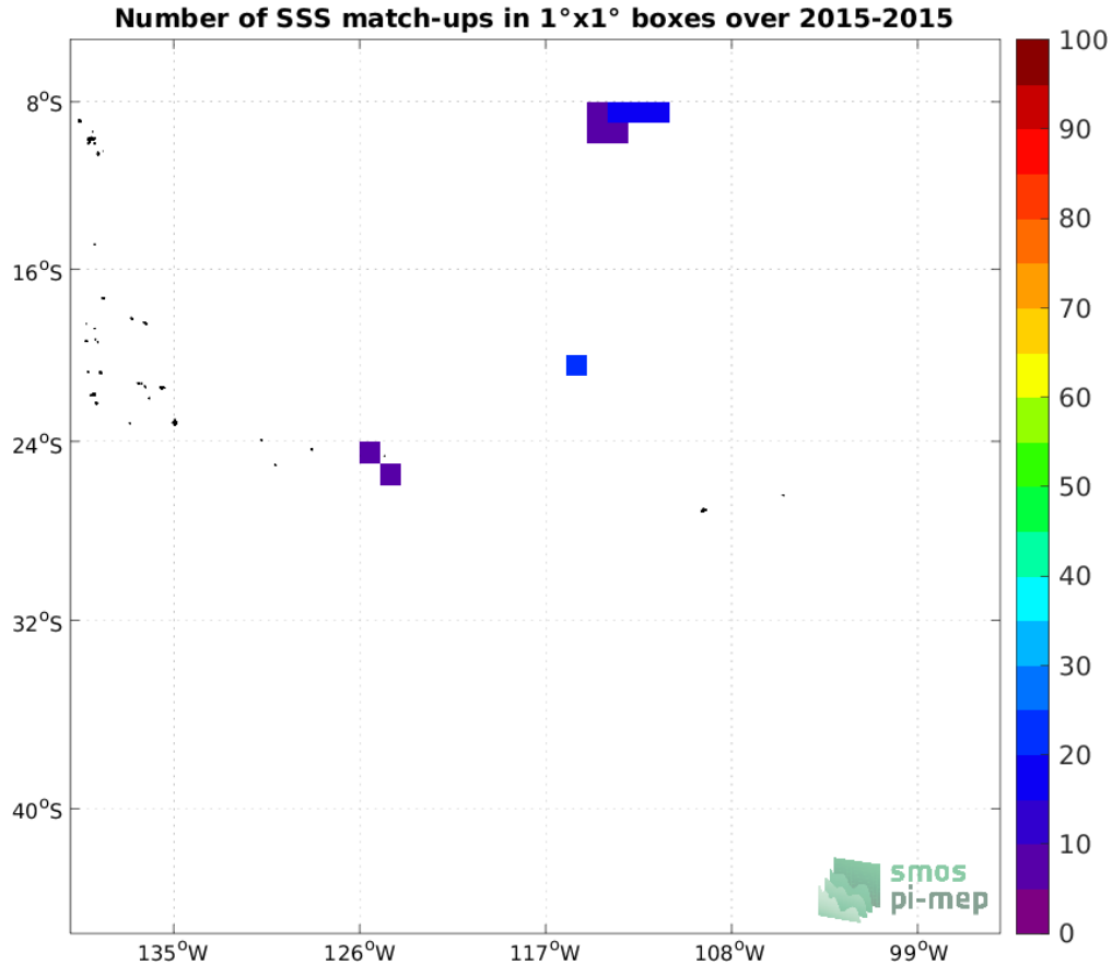
Figure 3: Number of SSS match-ups between Surface drifters SSS and the Aquarius SSS L2 OR v5 (NASA-GSFC) SSS product for the OTT zone Pi-MEP region over 1^\circ \times 1^\circ boxes and for the full satellite product period.
