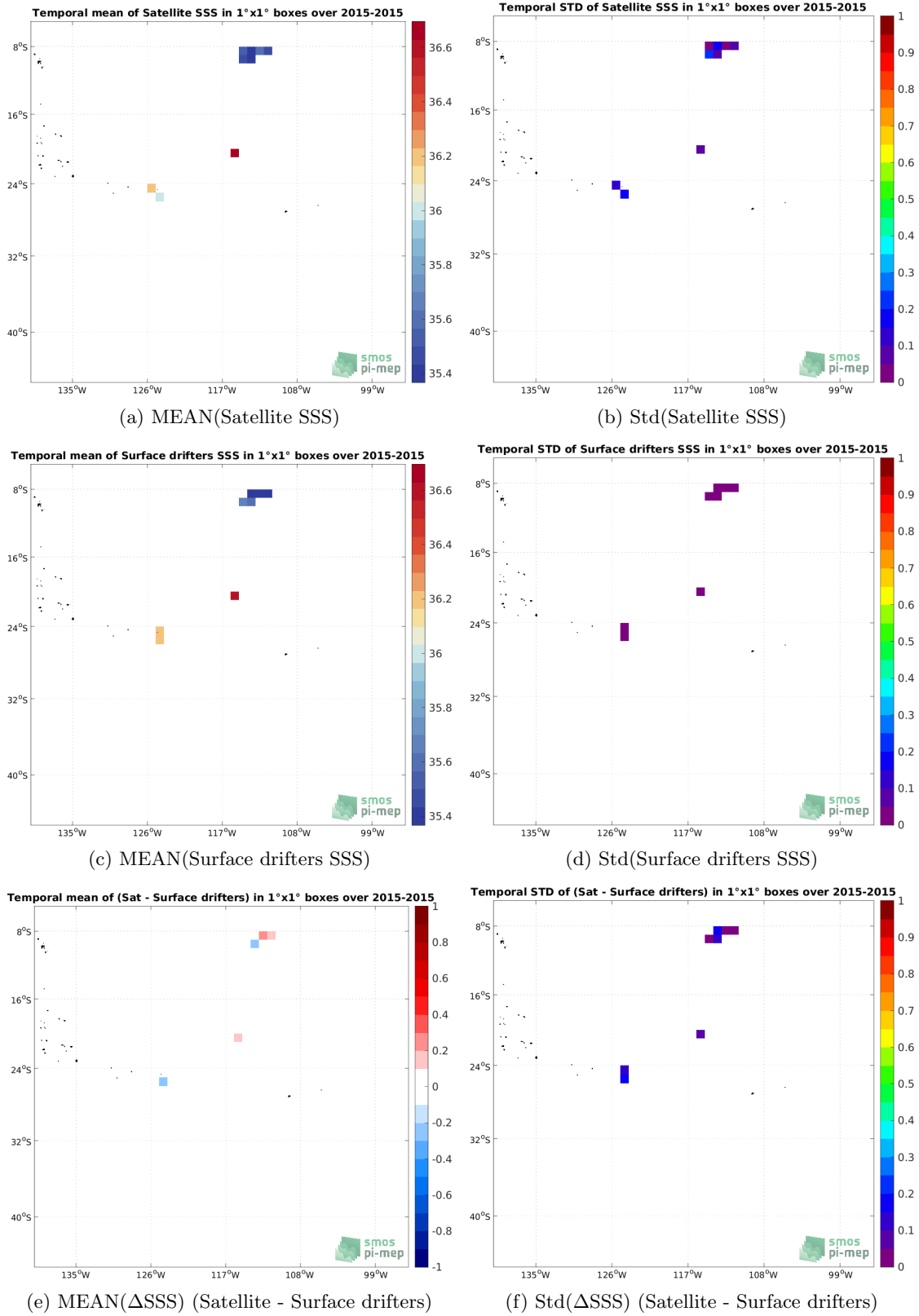
Figure 5: Temporal mean (left) and Std (right) of SSS from Aquarius SSS L2 OR v5 (NASA-GSFC) (top), Surface drifters (middle), and of \Delta SSS (Satellite - Surface drifters). Only match-up pairs are used to generate these maps.
