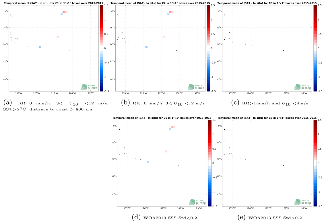
Figure 11: Temporal mean gridded over spatial boxes of size 1^\circ \times 1^\circ of \Delta SSS (Aquarius SSS L2 OR v5 (NASA-GSFC) - Surface drifters) for 5 different subdatasets corresponding to: RR=0 mm/h, 3 < U_{10} < 12 m/s, SST > 5^\circ C , distance to coast > 800 km (a), RR=0 mm/h, 3 < U_{10} < 12 m/s (b), RR > 1 mm/h and U_{10} < 4 m/s (c), WOA2013 SSS Std < 0.2 (d), WOA2013 SSS Std > 0.2 (e).
