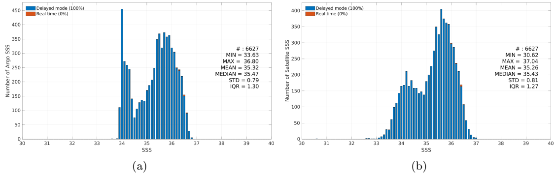
Figure 3: Histograms of SSS from Argo (a) and Aquarius SSS L2 OR v5 (NASA-GSFC) (b) considering all match-up pairs per bins of 0.1 over the OTT zone Pi-MEP region and for the full satellite product period.
