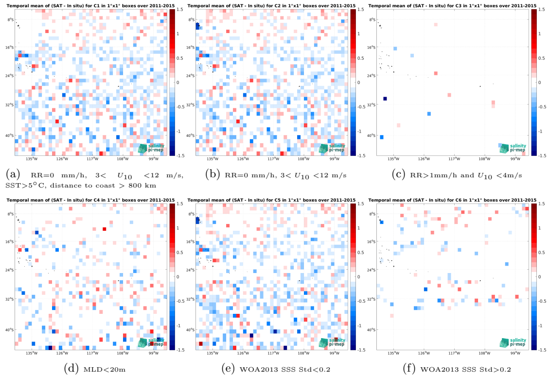
Figure 14: Temporal mean gridded over spatial boxes of size 1^\circ \times 1^\circ of \Delta SSS (Aquarius SSS L2 OR v5 (NASA-GSFC) - Argo) for 6 different subdatasets corresponding to:RR=0 mm/h, 3 < U_{10} < 12 m/s, SST >5^\circ C, distance to coast > 800 km (a), RR=0 mm/h, 3 < U_{10} < 12 m/s (b), RR >1 mm/h and U_{10} < 4 m/s (c),MLD <20 m (d),WOA2013 SSS Std <0.2 (e),WOA2013 SSS Std >0.2 (f).
