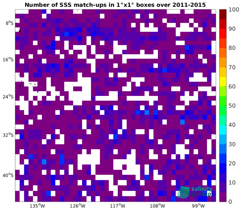
Figure 5: Number of SSS match-ups between Argo SSS and the Aquarius SSS L2 OR v5 (NASA-GSFC) SSS product for the OTT zone Pi-MEP region over 1^\circ \times 1^\circ boxes and for the full satellite product period.
