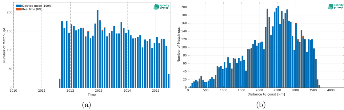
Figure 2: Number of match-ups between Argo and Aquarius SSS L2 OR v5 (NASA-GSFC) SSS as a function of time (a) and as function of the distance to coast (b) over the OTT zone Pi-MEP region and for the full satellite product period.
