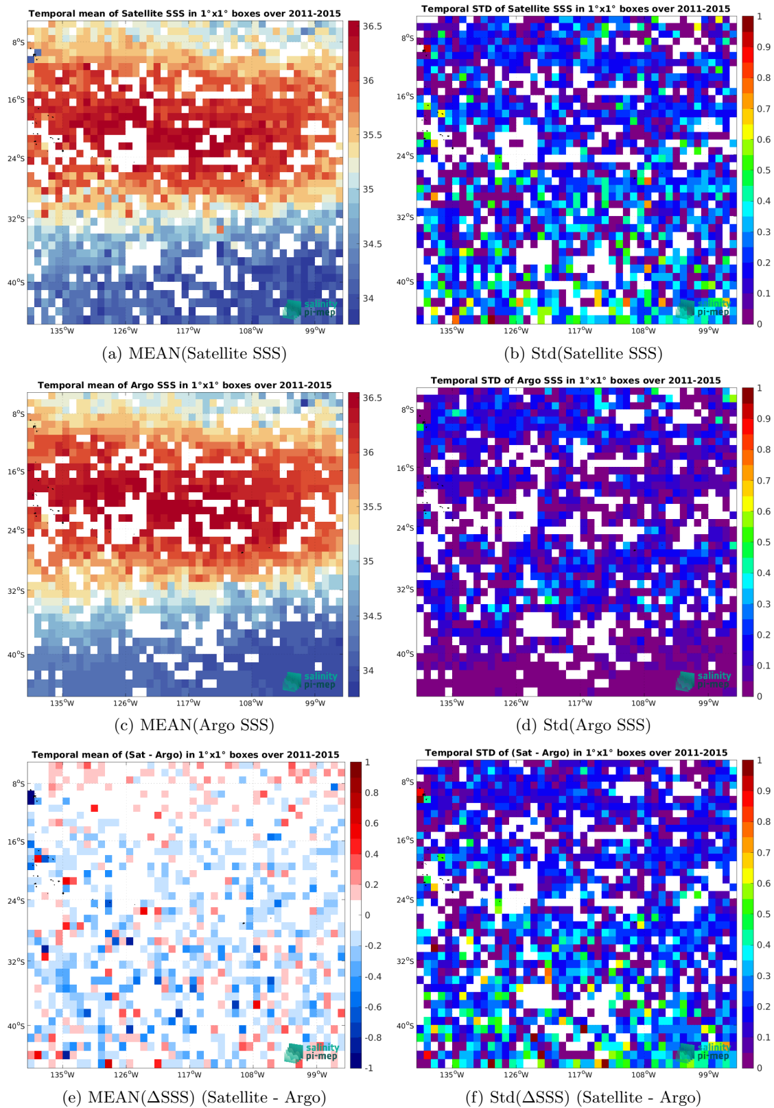
Figure 7: Temporal mean (left) and Std (right) of SSS from Aquarius SSS L2 OR v5 (NASA-GSFC) (top), Argo (middle), and of \Delta SSS (Satellite - Argo). Only match-up pairs are used to generate these maps.
