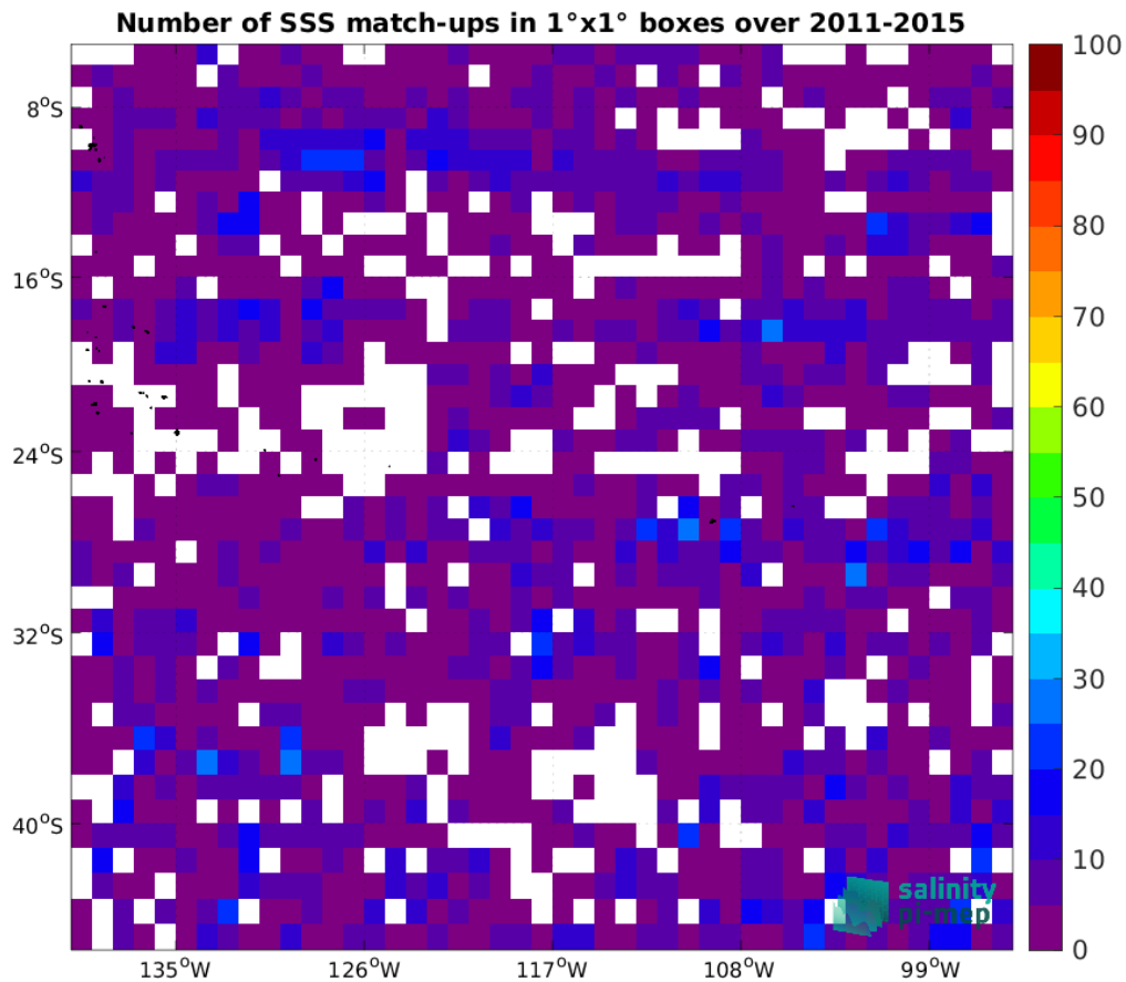
Figure 4: Number of SSS match-ups between Argo SSS and the Aquarius SSS L2 OR v5 (NASA-GSFC) SSS product for the OTT zone Pi-MEP region over 1°x1° boxes and for the full satellite product period.
