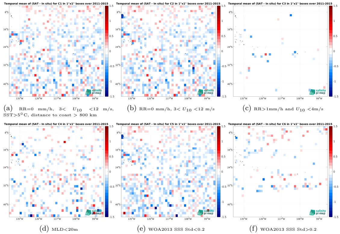
Figure 12: Temporal mean gridded over spatial boxes of size 1^\circ \times 1^\circ of \Delta SSS (Aquarius SSS L2 OR v5 (NASA-GSFC) - Argo) for 6 different subdatasets corresponding to:RR=0 mm/h, 3 < U_{10} < 12 m/s, SST >5^\circ\text{C} , distance to coast > 800 km (a), RR=0 mm/h, 3 < U_{10} < 12 m/s (b), RR >1 mm/h and U_{10} < 4 m/s (c),MLD <20 m (d),WOA2013 SSS Std <0.2 (e),WOA2013 SSS Std >0.2 (f).
