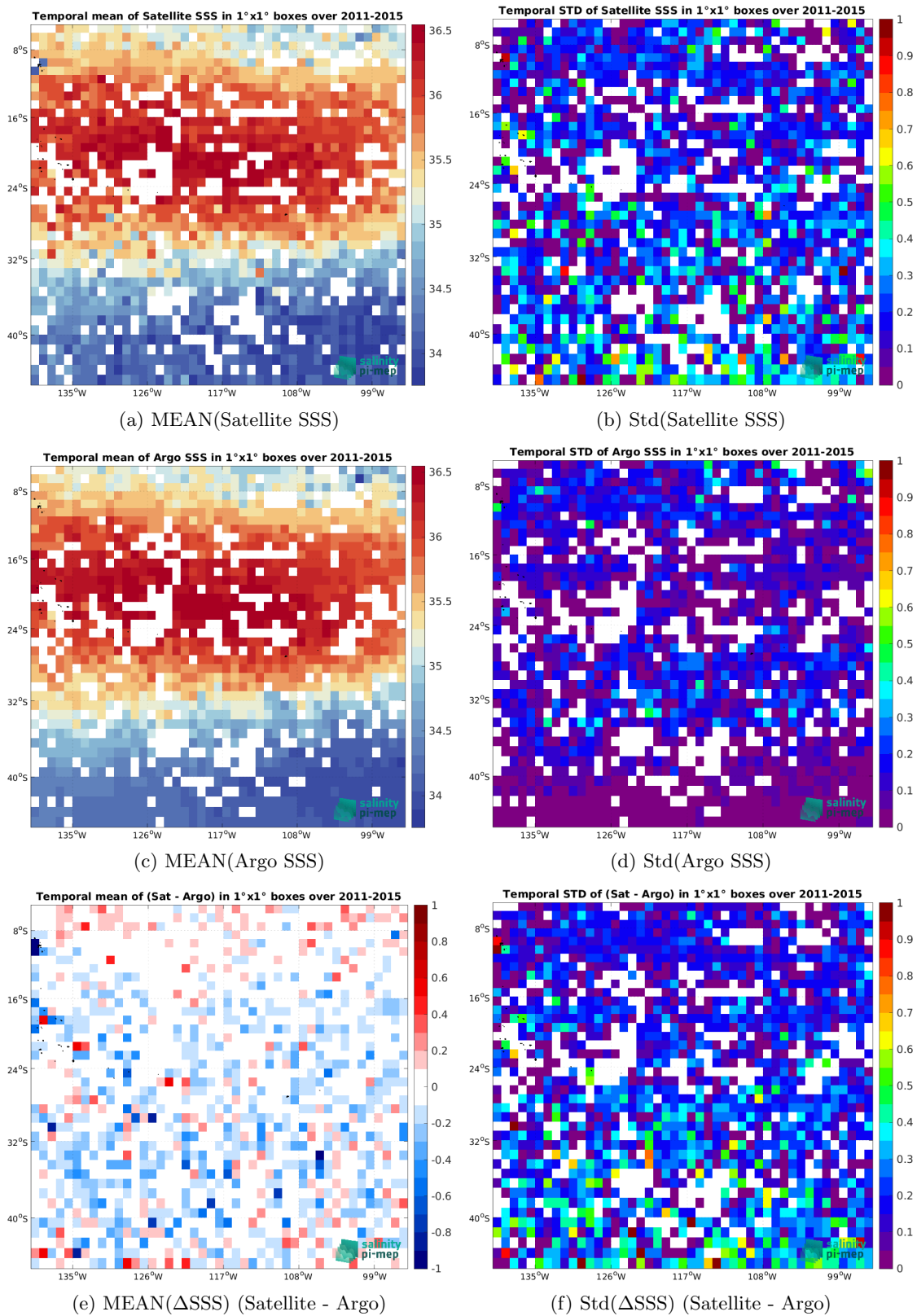
Figure 6: Temporal mean (left) and Std (right) of SSS from Aquarius SSS L2 OR v5 (NASA-GSFC) (top), Argo (middle), and of \Delta SSS (Satellite - Argo). Only match-up pairs are used to generate these maps.
