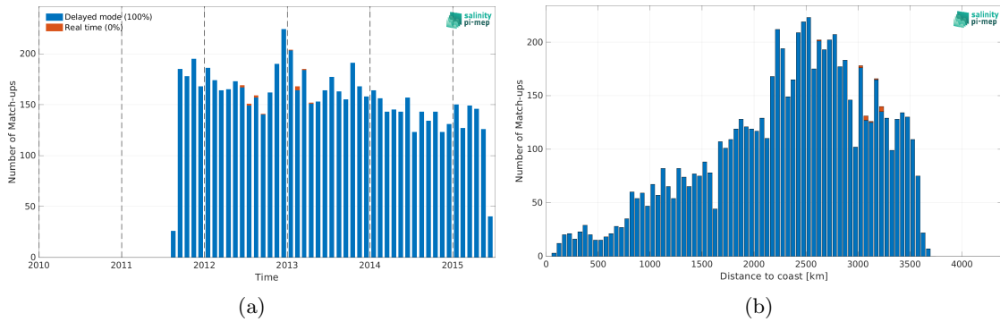
Figure 1: Number of match-ups between Argo and Aquarius SSS L2 OR v5 (NASA-GSFC) SSS as a function of time (a) and as function of the distance to coast (b) over the OTT zone Pi-MEP region and for the full satellite product period.
