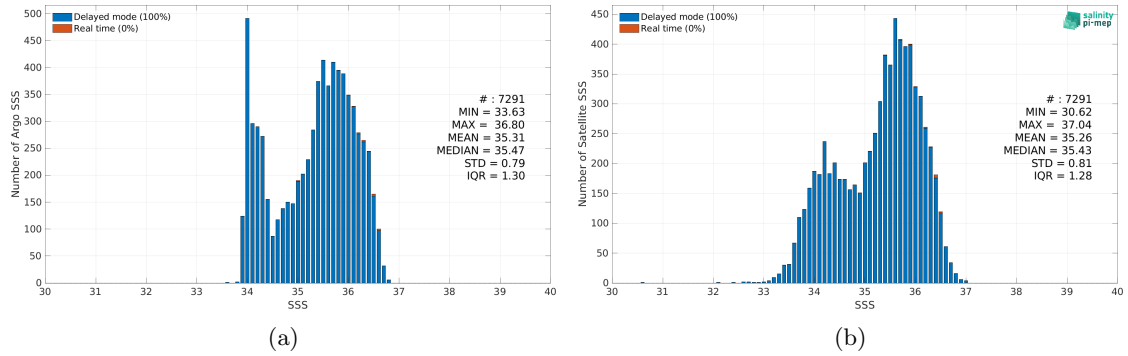
Figure 2: Histograms of SSS from Argo (a) and Aquarius SSS L2 OR v5 (NASA-GSFC) (b) considering all match-up pairs per bins of 0.1 over the OTT zone Pi-MEP region and for the full satellite product period.
