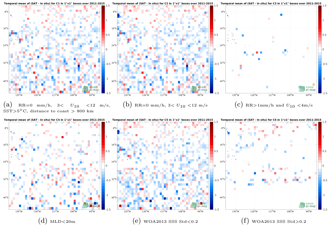
Figure 12: Temporal mean gridded over spatial boxes of size 1^\circ \times 1^\circ of \Delta SSS (Aquarius SSS L2 OR v5 (NASA-GSFC) - Argo) for 6 different subdatasets corresponding to:RR=0 mm/h, 3 < U_{10} < 12 m/s, SST >5^\circ C, distance to coast > 800 km (a), RR=0 mm/h, 3 < U_{10} < 12 m/s (b), RR >1 mm/h and U_{10} < 4 m/s (c),MLD <20 m (d),WOA2013 SSS Std <0.2 (e),WOA2013 SSS Std >0.2 (f).
