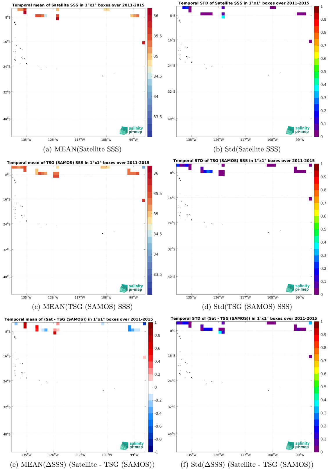
Figure 7: Temporal mean (left) and Std (right) of SSS from Aquarius SSS L2 CAP v5 (JPL) (top), TSG (SAMOS) (middle), and of \Delta SSS (Satellite - TSG (SAMOS)). Only match-up pairs are used to generate these maps.
