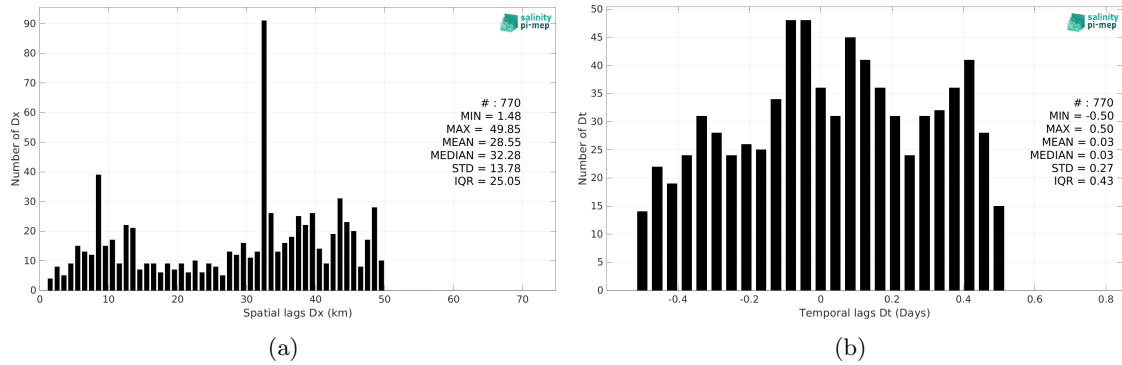
Figure 6: Histograms of the spatial (a) and temporal (b) lags between the location/time of the TSG (SAMOS) measurement and the date of the corresponding Aquarius SSS L2 CAP v5 (JPL) SSS pixel.
