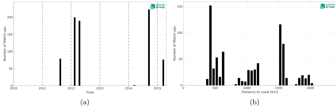
Figure 2: Number of match-ups between TSG (SAMOS) and Aquarius SSS L2 CAP v5 (JPL) SSS as a function of time (a) and as function of the distance to coast (b) over the OTT zone Pi-MEP region and for the full satellite product period.
