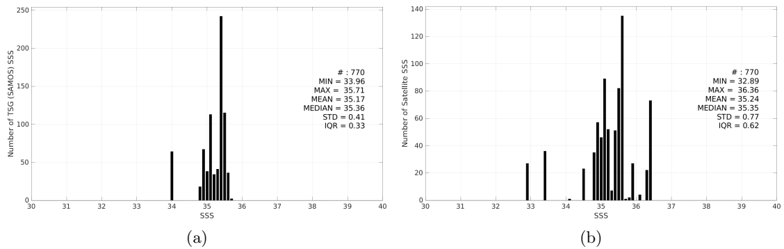
Figure 3: Histograms of SSS from TSG (SAMOS) (a) and Aquarius SSS L2 CAP v5 (JPL) (b) considering all match-up pairs per bins of 0.1 over the OTT zone Pi-MEP region and for the full satellite product period.
