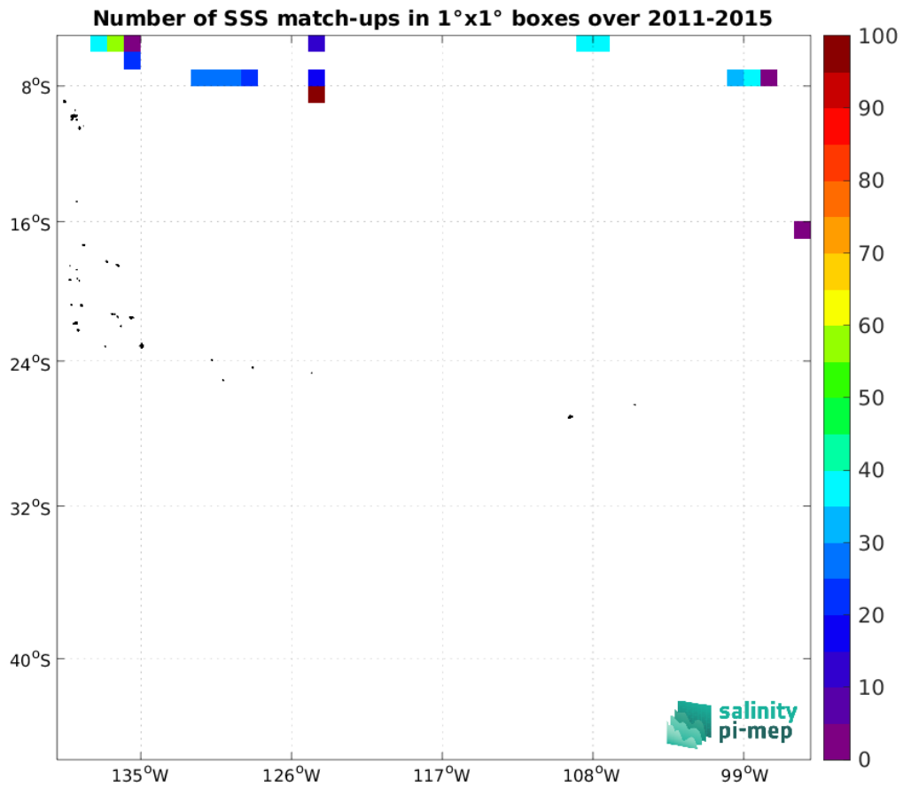
Figure 4: Number of SSS match-ups between TSG (SAMOS) SSS and the Aquarius SSS L2 CAP v5 (JPL) SSS product for the OTT zone Pi-MEP region over 1^\circ \times 1^\circ boxes and for the full satellite product period.
