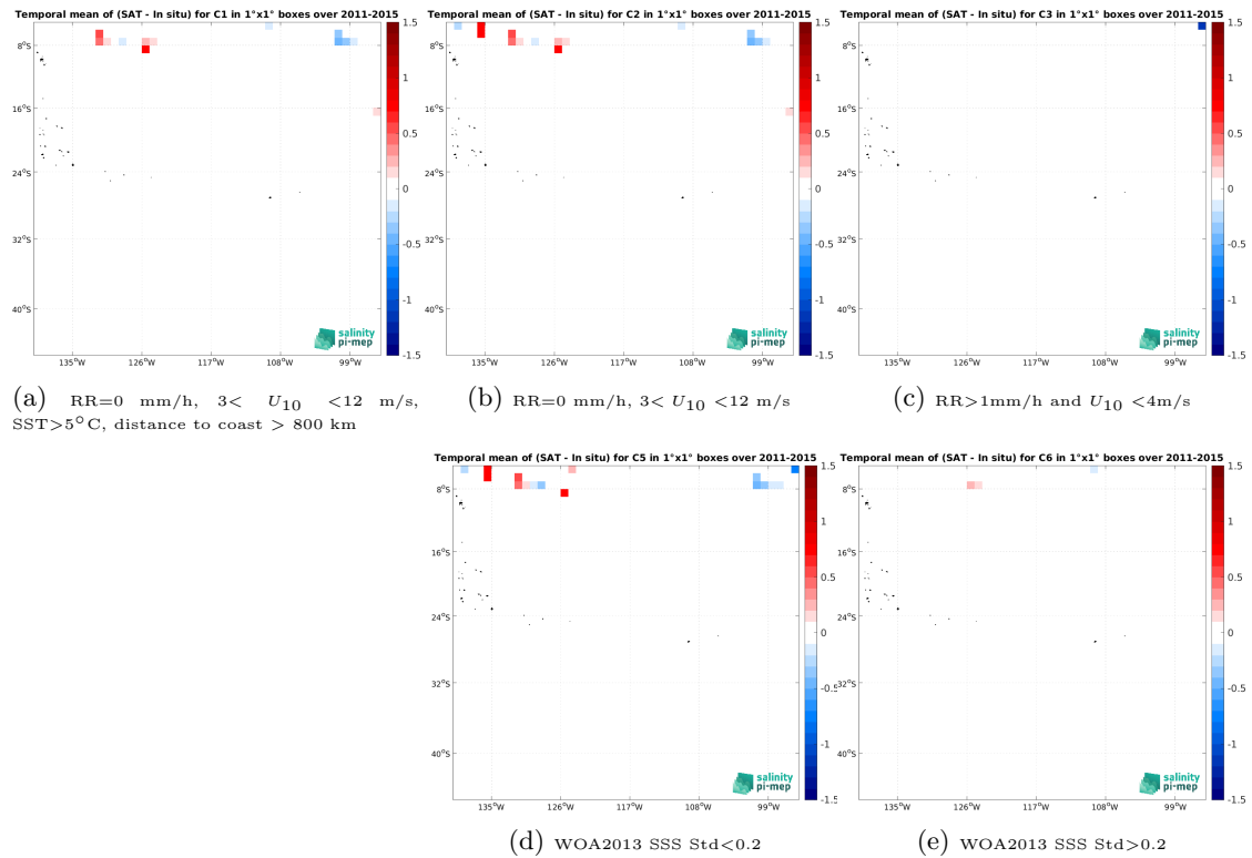
Figure 12: Temporal mean gridded over spatial boxes of size 1^\circ \times 1^\circ of \Delta\text{SSS} (Aquarius SSS L2 CAP v5 (JPL) - TSG (SAMOS)) for 5 different subdatasets corresponding to: \text{RR}=0 mm/h, 3 < U_{10} < 12 m/s, \text{SST} > 5^\circ\text{C} , distance to coast > 800 km (a), \text{RR}=0 mm/h, 3 < U_{10} < 12 m/s (b), \text{RR} > 1 mm/h and U_{10} < 4 m/s (c), WOA2013 SSS Std < 0.2 (d), WOA2013 SSS Std > 0.2 (e).
