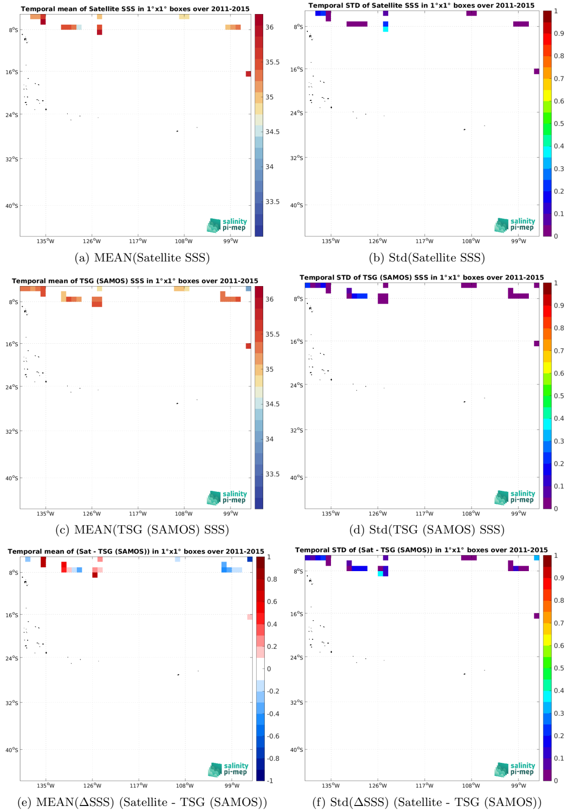
Figure 6: Temporal mean (left) and Std (right) of SSS from Aquarius SSS L2 CAP v5 (JPL) (top), TSG (SAMOS) (middle), and of \Delta SSS (Satellite - TSG (SAMOS)). Only match-up pairs are used to generate these maps.
