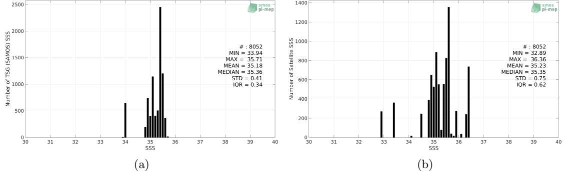
Figure 2: Histograms of SSS from TSG (SAMOS) (a) and Aquarius SSS L2 CAP v5 (JPL) (b) considering all match-up pairs per bins of 0.1 over the OTT zone Pi-MEP region and for the full satellite product period.
