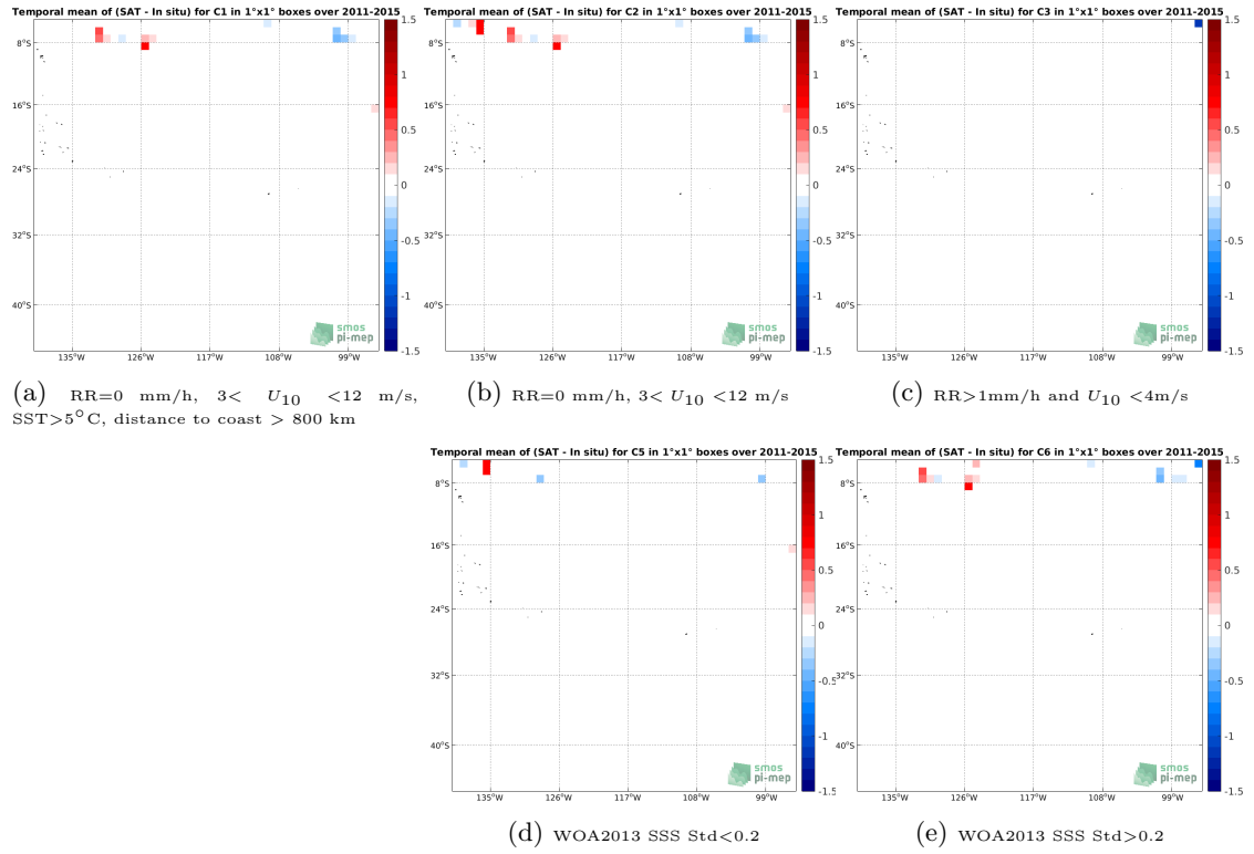
Figure 12: Temporal mean gridded over spatial boxes of size 1^\circ \times 1^\circ of \Delta SSS (Aquarius SSS L2 CAP v5 (JPL) - TSG (SAMOS)) for 5 different subdatasets corresponding to: RR=0 mm/h, 3 < U_{10} < 12 m/s, SST > 5^\circ C , distance to coast > 800 km (a), RR=0 mm/h, 3 < U_{10} < 12 m/s (b), RR > 1 mm/h and U_{10} < 4 m/s (c), WOA2013 SSS Std < 0.2 (d), WOA2013 SSS Std > 0.2 (e).
