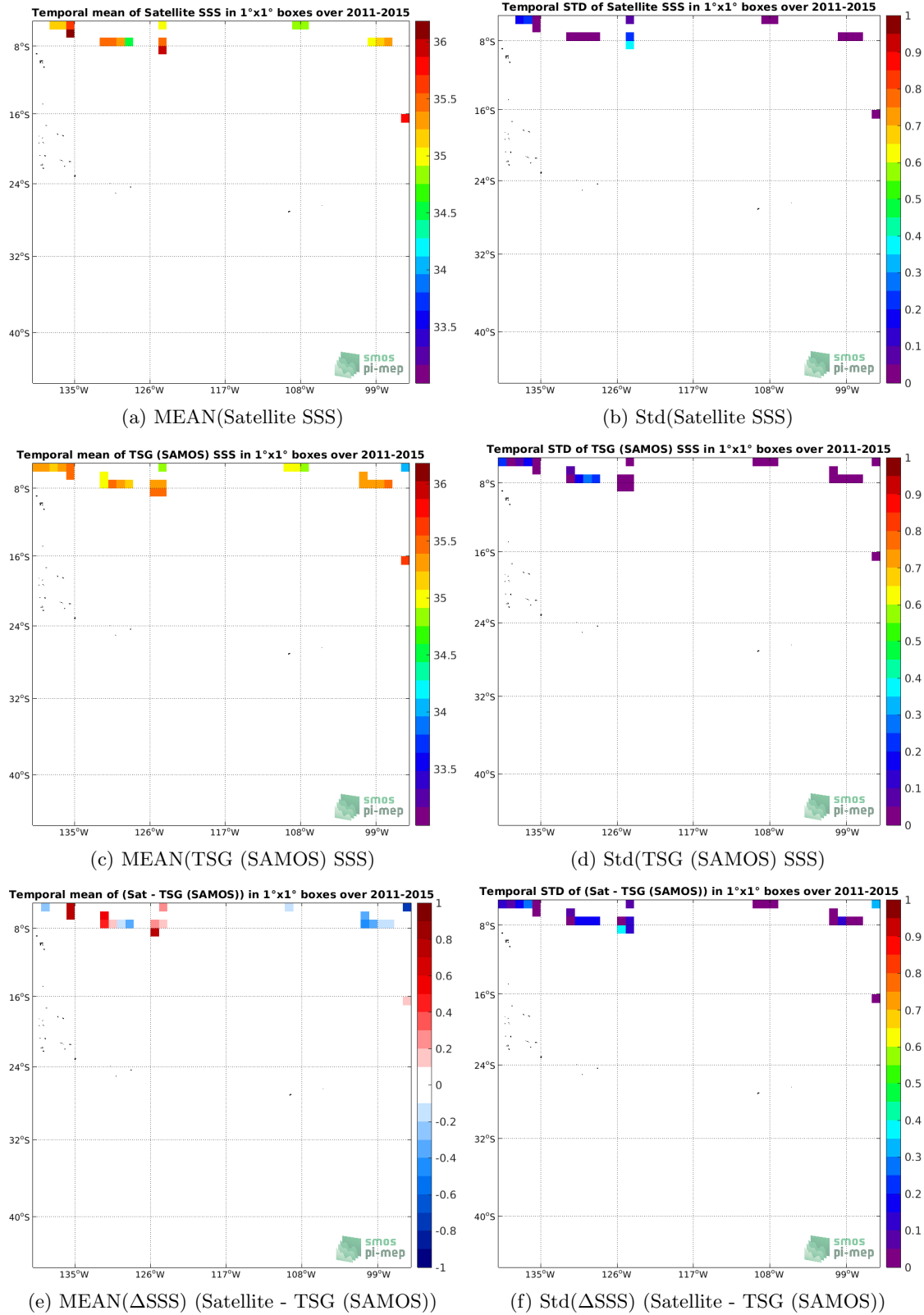
Figure 6: Temporal mean (left) and Std (right) of SSS from Aquarius SSS L2 CAP v5 (JPL) (top), TSG (SAMOS) (middle), and of ΔSSS (Satellite - TSG (SAMOS)). Only match-up pairs are used to generate these maps.
