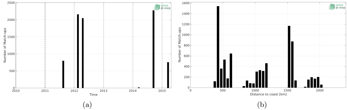
Figure 1: Number of match-ups between TSG (SAMOS) and Aquarius SSS L2 CAP v5 (JPL) SSS as a function of time (a) and as function of the distance to coast (b) over the OTT zone Pi-MEP region and for the full satellite product period.
