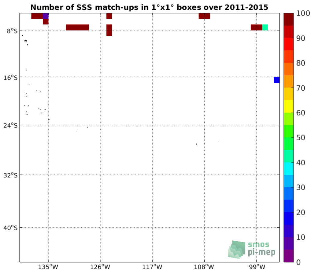
Figure 4: Number of SSS match-ups between TSG (SAMOS) SSS and the Aquarius SSS L2 CAP v5 (JPL) SSS product for the OTT zone Pi-MEP region over 1°x1° boxes and for the full satellite product period.
