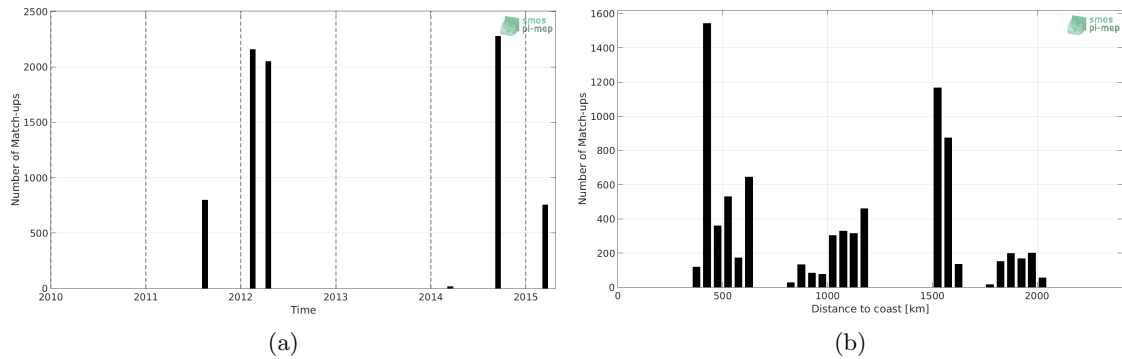
Figure 1: Number of match-ups between TSG-SAMOS and Aquarius-L2-JPL-V5 SSS as a function of time (a) and as function of the distance to coast (b) over the OTT zone Pi-MEP region and for the full satellite product period.
