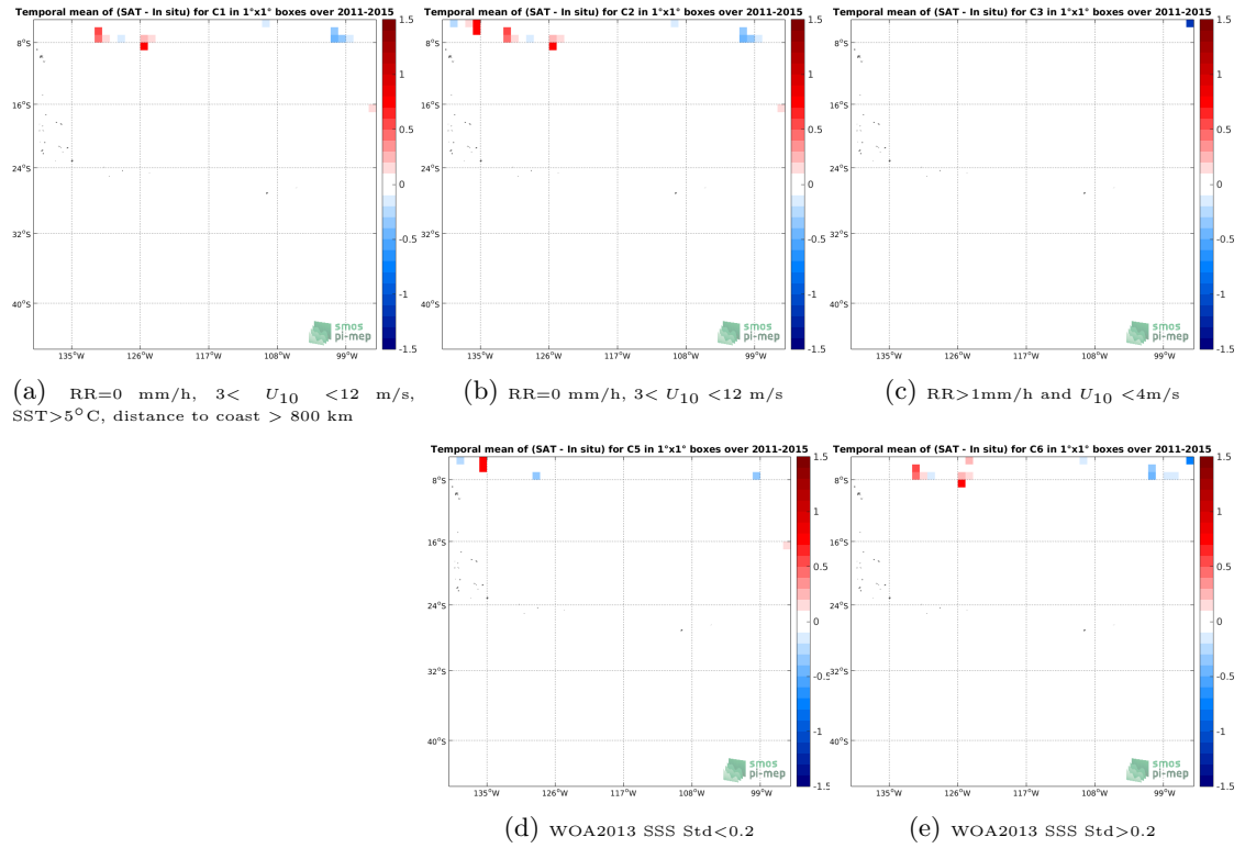
Figure 12: Temporal mean gridded over spatial boxes of size 1^\circ \times 1^\circ of \Delta SSS (Aquarius-L2-JPL-V5 - TSG-SAMOS) for 5 different subdatasets corresponding to: RR=0 mm/h, 3 < U_{10} < 12 m/s, SST > 5^\circ C , distance to coast > 800 km (a), RR=0 mm/h, 3 < U_{10} < 12 m/s (b), RR > 1 mm/h and U_{10} < 4 m/s (c), WOA2013 SSS Std < 0.2 (d), WOA2013 SSS Std > 0.2 (e).
