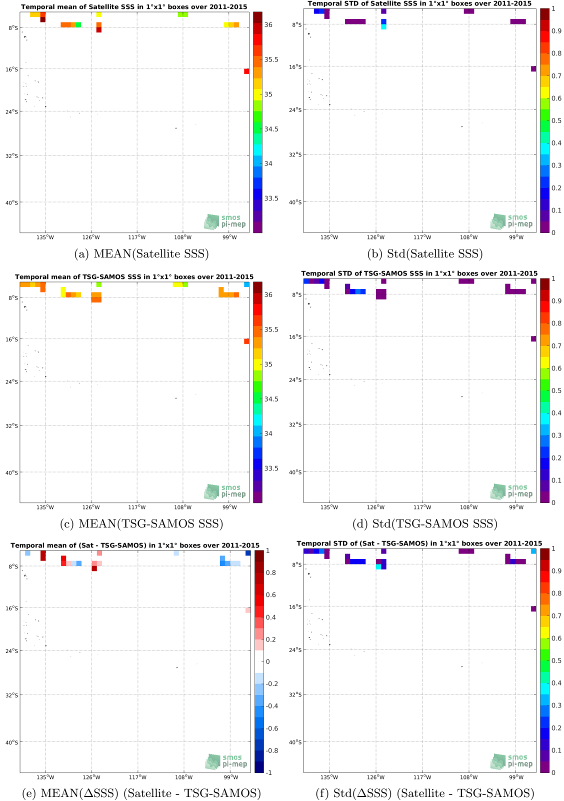
Figure 6: Temporal mean (left) and Std (right) of SSS from Aquarius-L2-JPL-V5 (top), TSG-SAMOS (middle), and of \Delta SSS (Satellite - TSG-SAMOS). Only match-up pairs are used to generate these maps.
