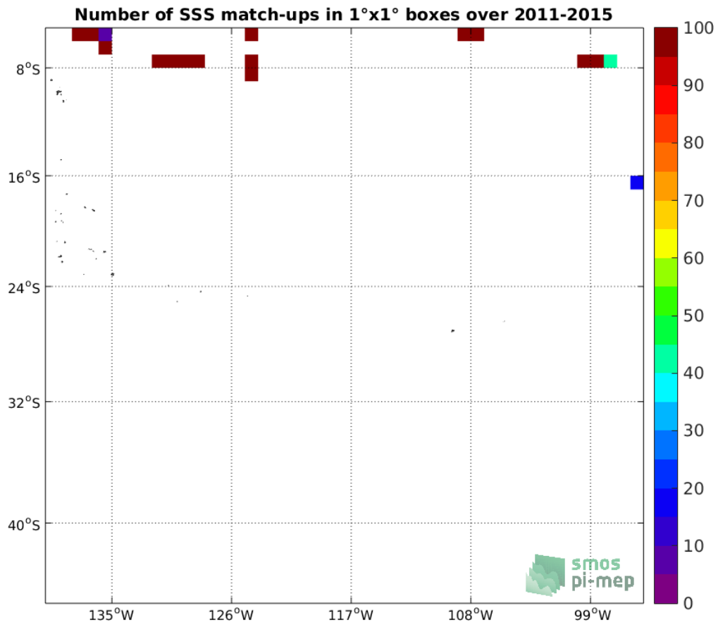
Figure 4: Number of SSS match-ups between TSG-SAMOS SSS and the Aquarius-L2-JPL-V5 SSS product for the OTT zone Pi-MEP region over 1°x1° boxes and for the full satellite product period.
