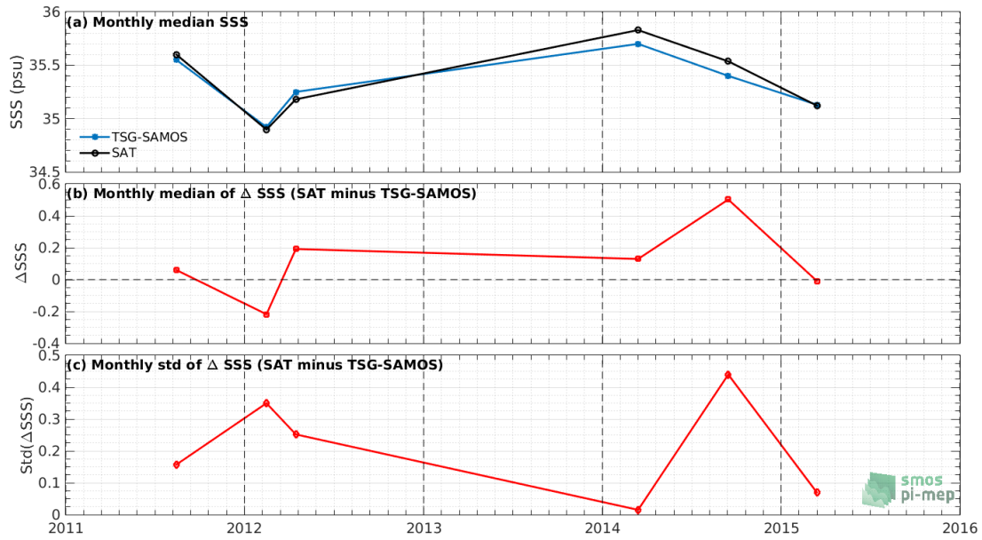
Figure 7: Time series of the monthly median SSS (top), median of \Delta SSS (Satellite - TSG-SAMOS) and Std of \Delta SSS (Satellite - TSG-SAMOS) over the OTT zone Pi-MEP region considering all match-ups collected by the Pi-MEP.
