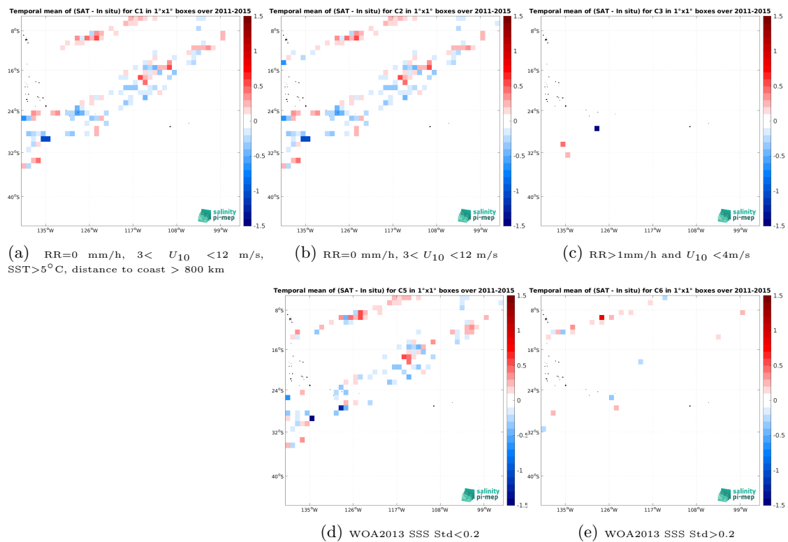
Figure 14: Temporal mean gridded over spatial boxes of size 1^\circ \times 1^\circ of \Delta SSS (Aquarius SSS L2 CAP v5 (JPL) - TSG (LEGOS-DM)) for 5 different subdatasets corresponding to:RR=0 mm/h, 3 < U_{10} < 12 m/s, SST >5^\circ\text{C} , distance to coast > 800 km (a), RR=0 mm/h, 3 < U_{10} < 12 m/s (b), RR >1 mm/h and U_{10} < 4 m/s (c), WOA2013 SSS Std <0.2 (d), WOA2013 SSS Std >0.2 (e).
