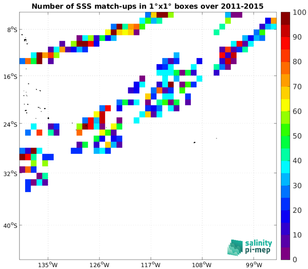
Figure 5: Number of SSS match-ups between TSG (LEGOS-DM) SSS and the Aquarius SSS L2 CAP v5 (JPL) SSS product for the OTT zone Pi-MEP region over 1°x1° boxes and for the full satellite product period.
