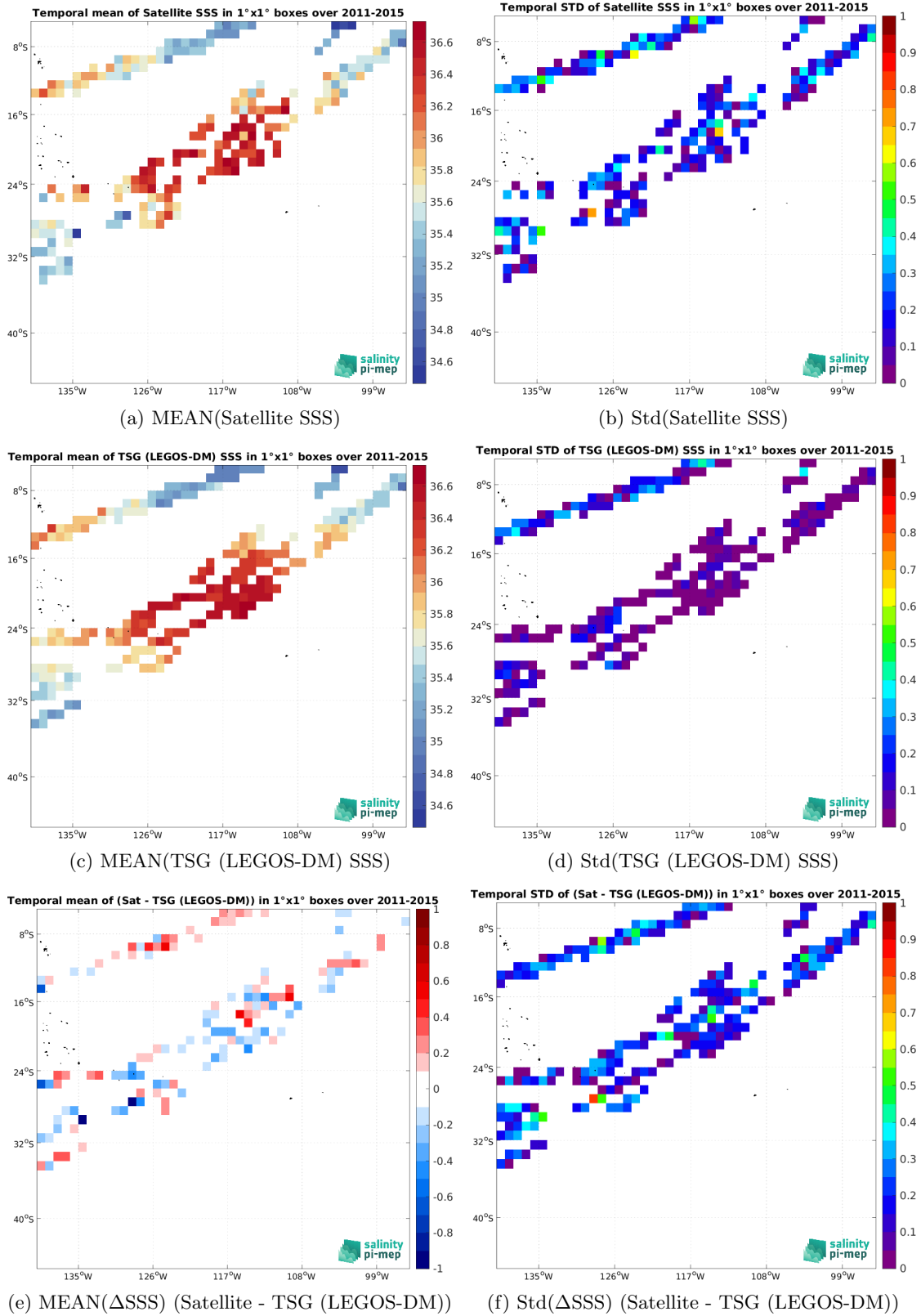
Figure 7: Temporal mean (left) and Std (right) of SSS from Aquarius SSS L2 CAP v5 (JPL) (top), TSG (LEGOS-DM) (middle), and of \Delta SSS (Satellite - TSG (LEGOS-DM)). Only match-up pairs are used to generate these maps.
