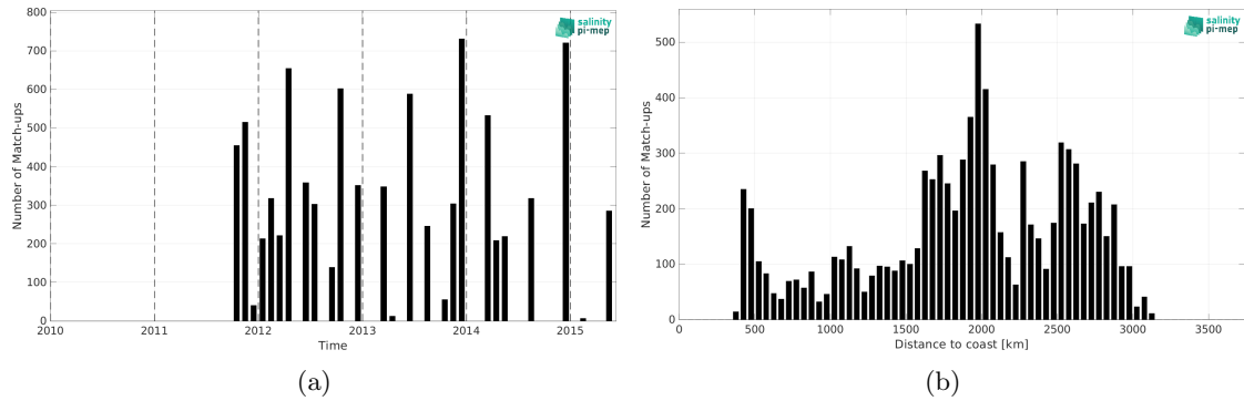
Figure 2: Number of match-ups between TSG (LEGOS-DM) and Aquarius SSS L2 CAP v5 (JPL) SSS as a function of time (a) and as function of the distance to coast (b) over the OTT zone Pi-MEP region and for the full satellite product period.
