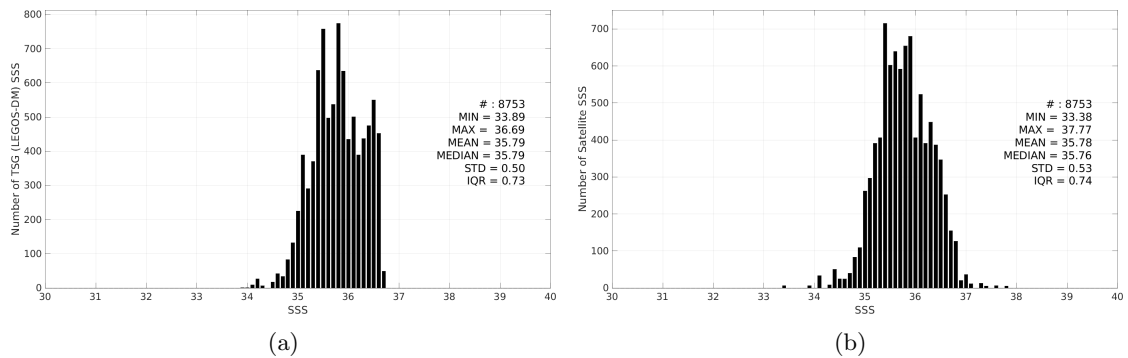
Figure 3: Histograms of SSS from TSG (LEGOS-DM) (a) and Aquarius SSS L2 CAP v5 (JPL) (b) considering all match-up pairs per bins of 0.1 over the OTT zone Pi-MEP region and for the full satellite product period.
