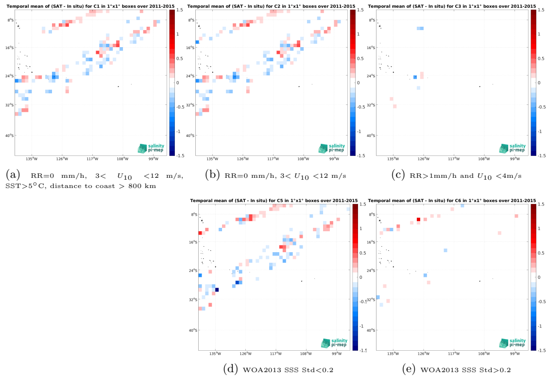
Figure 12: Temporal mean gridded over spatial boxes of size 1^\circ \times 1^\circ of \Delta\text{SSS} (Aquarius SSS L2 CAP v5 (JPL) - TSG (LEGOS-DM)) for 5 different subdatasets corresponding to:RR=0 mm/h, 3 < U_{10} < 12 m/s, SST > 5^\circ\text{C} , distance to coast > 800 km (a), RR=0 mm/h, 3 < U_{10} < 12 m/s (b), RR > 1 mm/h and U_{10} < 4 m/s (c), WOA2013 SSS Std < 0.2 (d), WOA2013 SSS Std > 0.2 (e).
