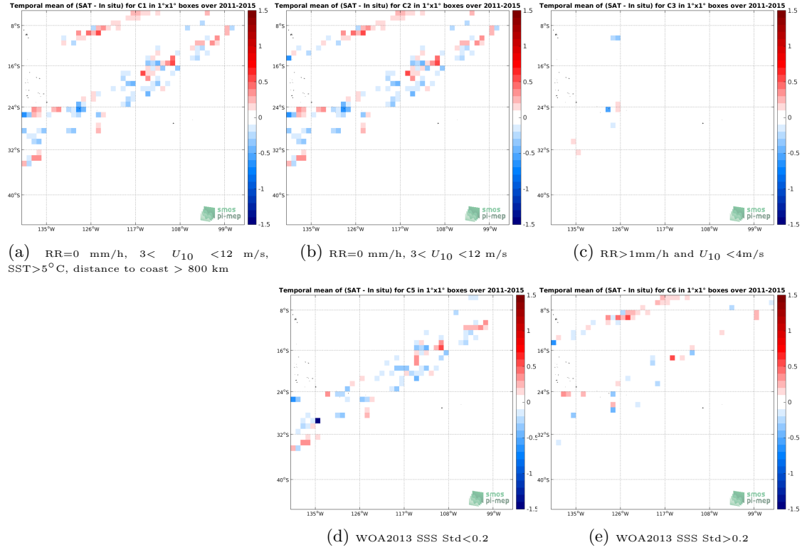
Figure 12: Temporal mean gridded over spatial boxes of size 1^\circ \times 1^\circ of \Delta SSS (Aquarius-L2-JPL-V5 - TSG-LEGOS-DM) for 5 different subdatasets corresponding to: RR=0 mm/h, 3 < U_{10} < 12 m/s, SST > 5^\circ C , distance to coast > 800 km (a), RR=0 mm/h, 3 < U_{10} < 12 m/s (b), RR > 1 mm/h and U_{10} < 4 m/s (c), WOA2013 SSS Std < 0.2 (d), WOA2013 SSS Std > 0.2 (e).
