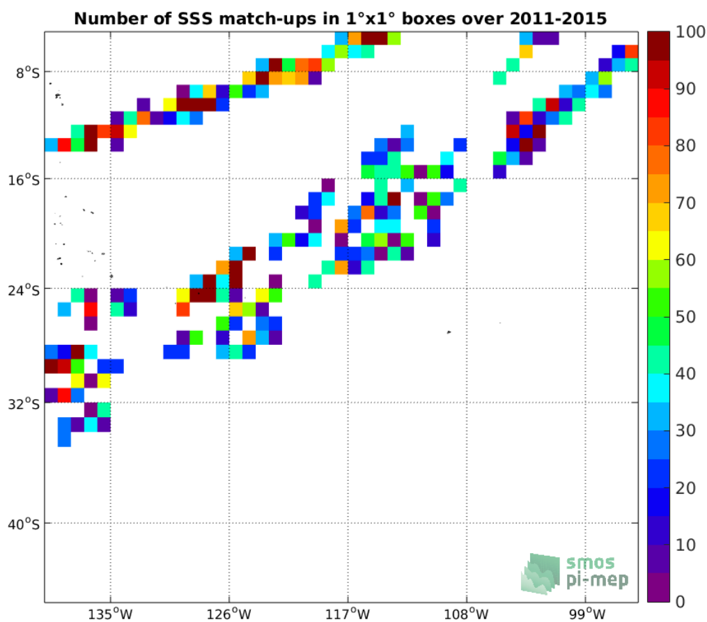
Figure 4: Number of SSS match-ups between TSG-LEGOS-DM SSS and the Aquarius-L2-JPL-V5 SSS product for the OTT zone Pi-MEP region over 1°x1° boxes and for the full satellite product period.
