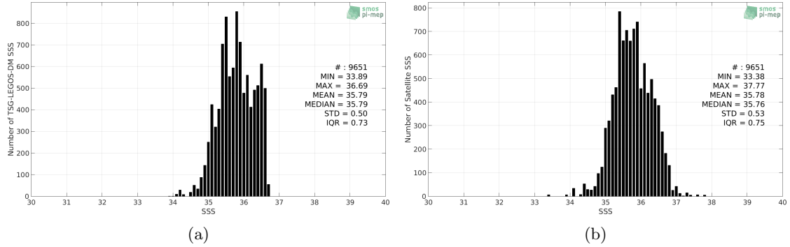
Figure 2: Histograms of SSS from TSG-LEGOS-DM (a) and Aquarius-L2-JPL-V5 (b) considering all match-up pairs per bins of 0.1 over the OTT zone Pi-MEP region and for the full satellite product period.
