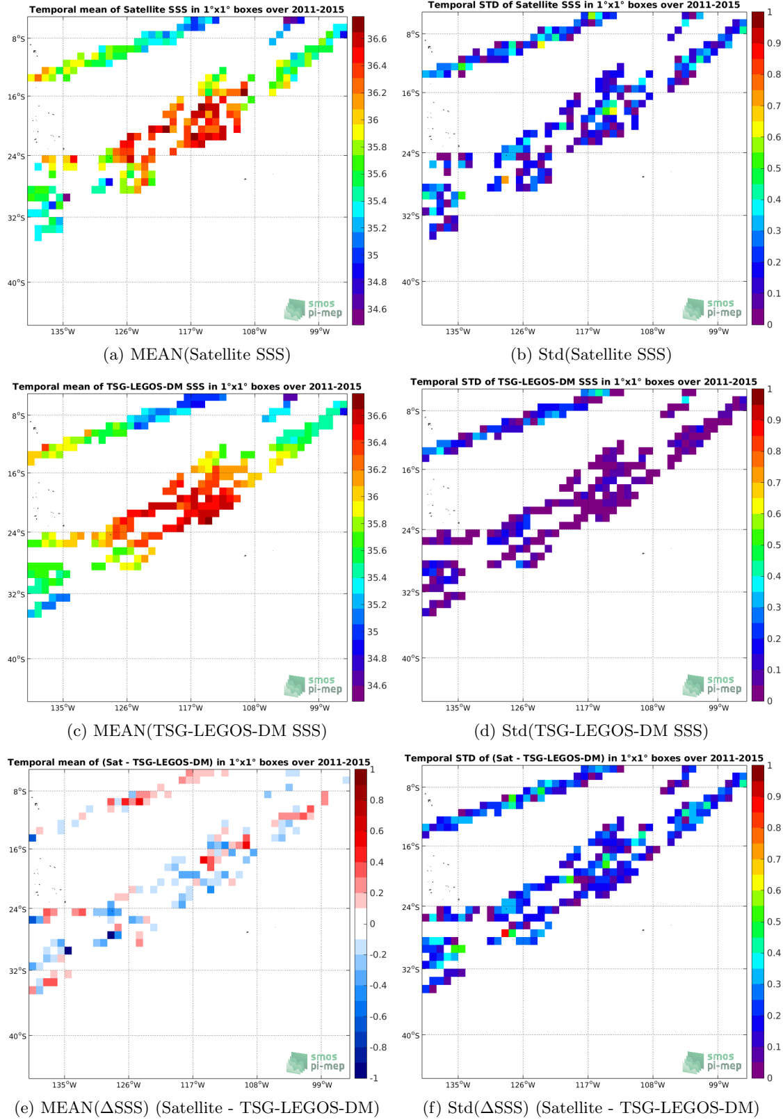
Figure 6: Temporal mean (left) and Std (right) of SSS from Aquarius-L2-JPL-V5 (top), TSG-LEGOS-DM (middle), and of \Delta SSS (Satellite - TSG-LEGOS-DM). Only match-up pairs are used to generate these maps.
