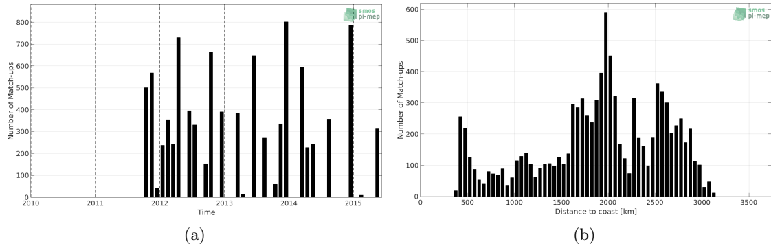
Figure 1: Number of match-ups between TSG-LEGOS-DM and Aquarius-L2-JPL-V5 SSS as a function of time (a) and as function of the distance to coast (b) over the OTT zone Pi-MEP region and for the full satellite product period.
