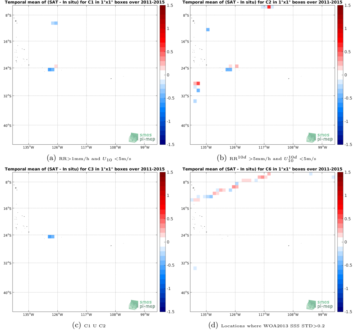
Figure 12: Temporal mean gridded over spatial boxes of size 1^\circ \times 1^\circ of \Delta SSS (Aquarius-L2-JPL-V5 - TSG-LEGOS-DM) for 4 different subdatasets corresponding to: RR > 1\text{mm/h} and U_{10} < 5\text{m/s} (a), RR^{10d} > 5\text{mm/h} and U_{10}^{10d} < 5\text{m/s} (b), C1 U C2 (c), Locations where WOA2013 SSS STD > 0.2 (d).
