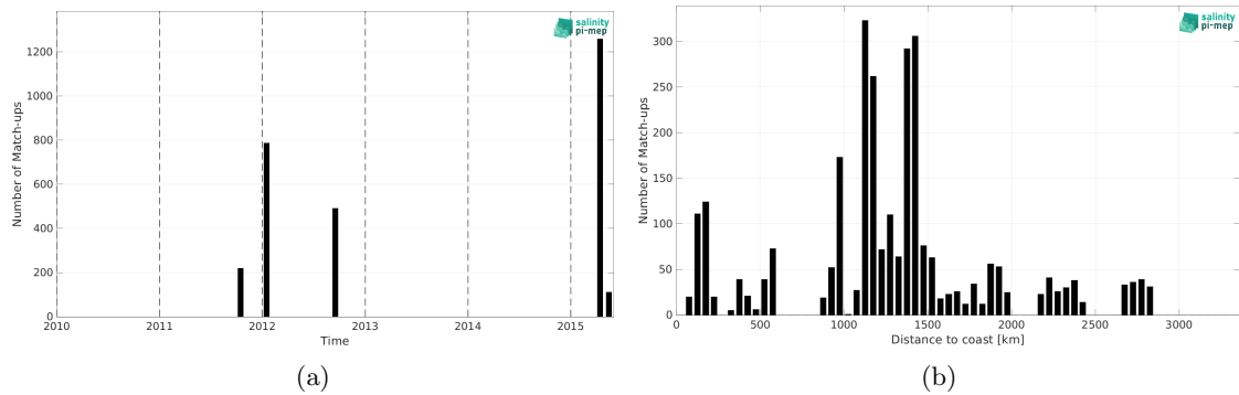
Figure 2: Number of match-ups between TSG (GOSUD-Research-vessel) and Aquarius SSS L2 CAP v5 (JPL) SSS as a function of time (a) and as function of the distance to coast (b) over the OTT zone Pi-MEP region and for the full satellite product period.
