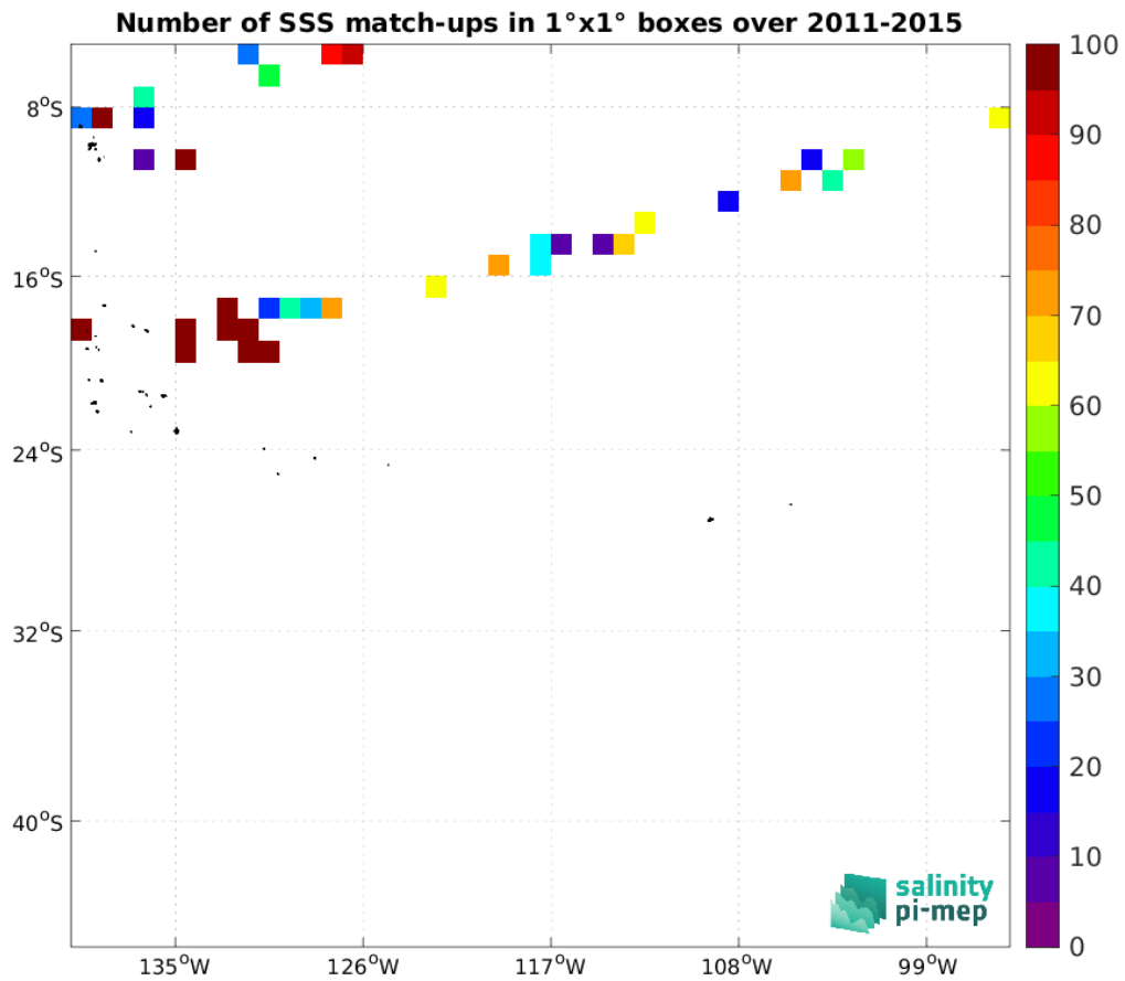
Figure 5: Number of SSS match-ups between TSG (GOSUD-Research-vessel) SSS and the Aquarius SSS L2 CAP v5 (JPL) SSS product for the OTT zone Pi-MEP region over 1^\circ \times 1^\circ boxes and for the full satellite product period.
