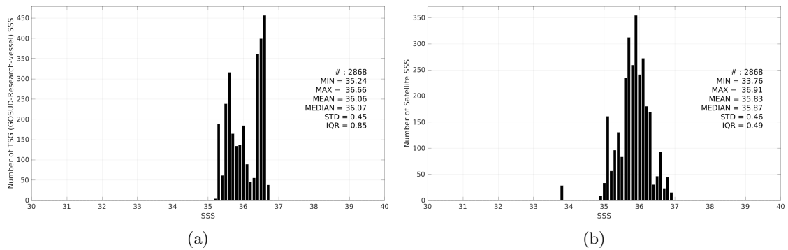
Figure 3: Histograms of SSS from TSG (GOSUD-Research-vessel) (a) and Aquarius SSS L2 CAP v5 (JPL) (b) considering all match-up pairs per bins of 0.1 over the OTT zone Pi-MEP region and for the full satellite product period.
