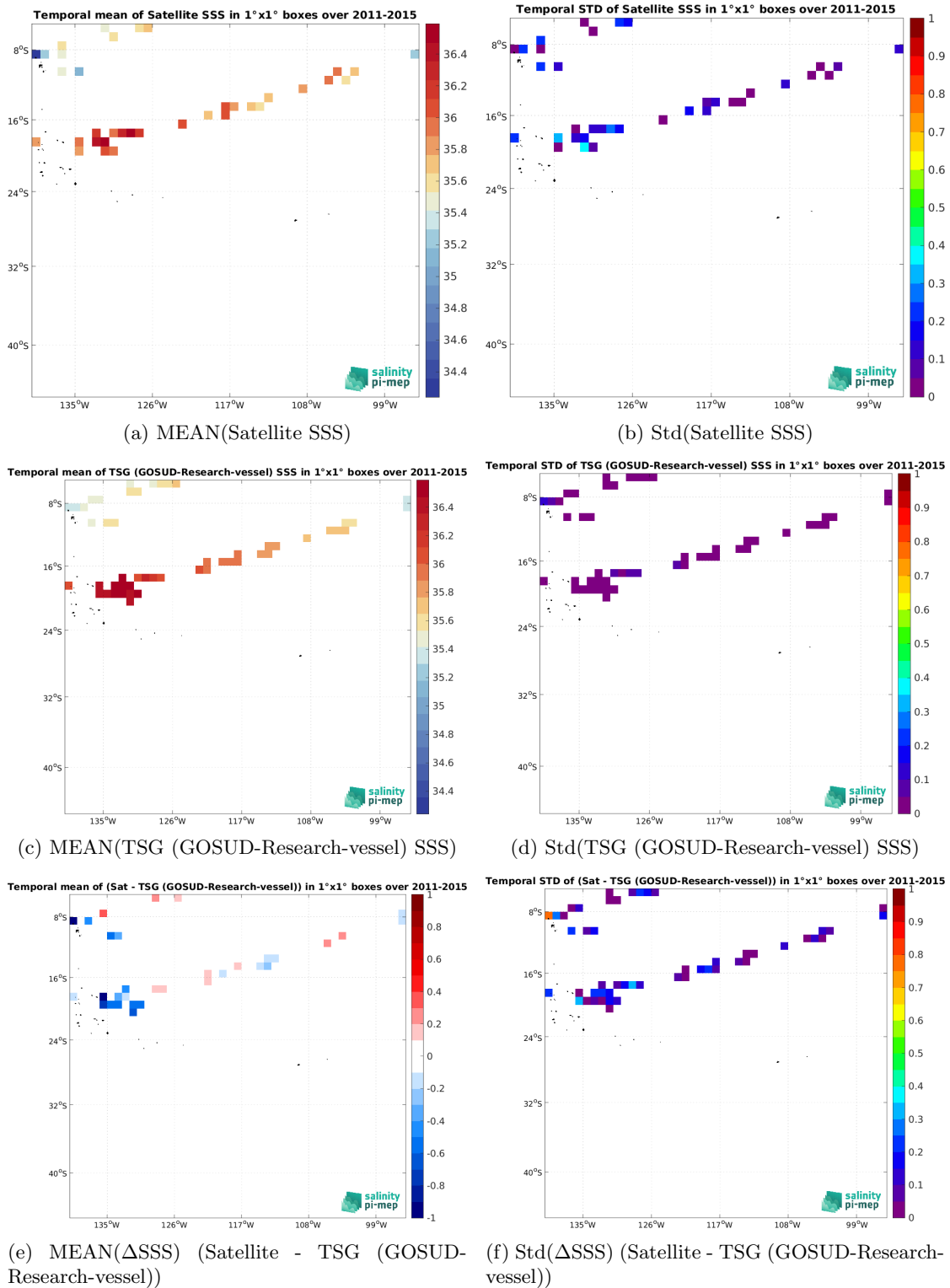
Figure 7: Temporal mean (left) and Std (right) of SSS from Aquarius SSS L2 CAP v5 (JPL) (top), TSG (GOSUD-Research-vessel) (middle), and of \Delta SSS (Satellite - TSG (GOSUD-Research-vessel)). Only match-up pairs are used to generate these maps.
