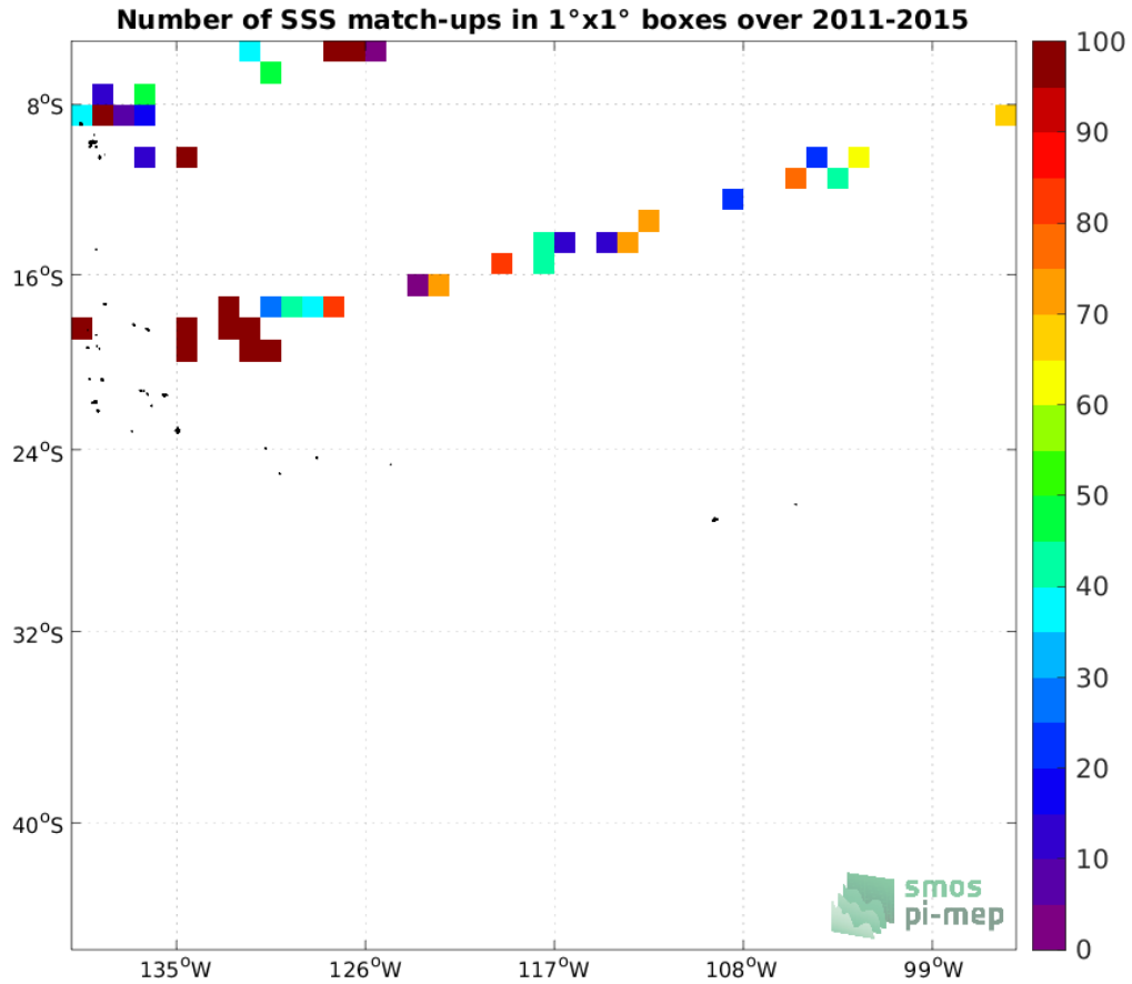
Figure 4: Number of SSS match-ups between TSG (GOSUD-Research-vessel) SSS and the Aquarius SSS L2 CAP v5 (JPL) SSS product for the OTT zone Pi-MEP region over 1°x1° boxes and for the full satellite product period.
