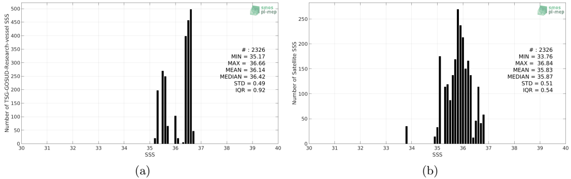
Figure 2: Histograms of SSS from TSG-GOSUD-Research-vessel (a) and Aquarius-L2-JPL-V5 (b) considering all match-up pairs per bins of 0.1 over the OTT zone Pi-MEP region and for the full satellite product period.
