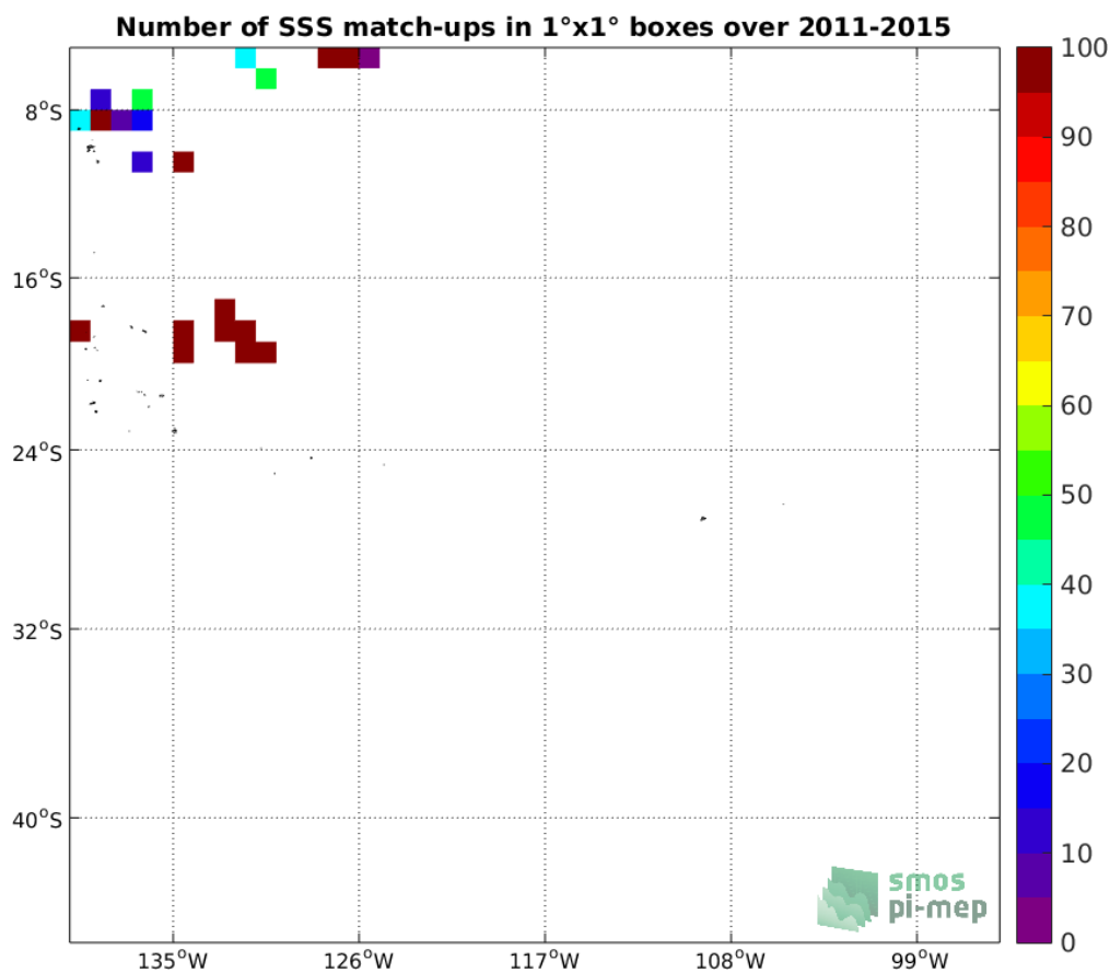
Figure 4: Number of SSS match-ups between TSG-GOSUD-Research-vessel SSS and the Aquarius-L2-JPL-V5 SSS product for the OTT zone Pi-MEP region over 1°x1° boxes and for the full satellite product period.
