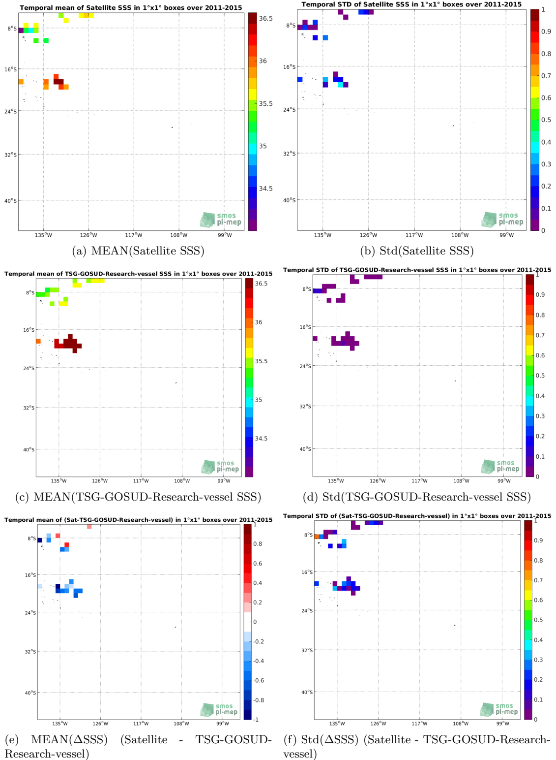
Figure 6: Temporal mean (left) and Std (right) of SSS from Aquarius-L2-JPL-V5 (top), TSG-GOSUD-Research-vessel (middle), and of \Delta SSS (Satellite - TSG-GOSUD-Research-vessel). Only match-up pairs are used to generate these maps
