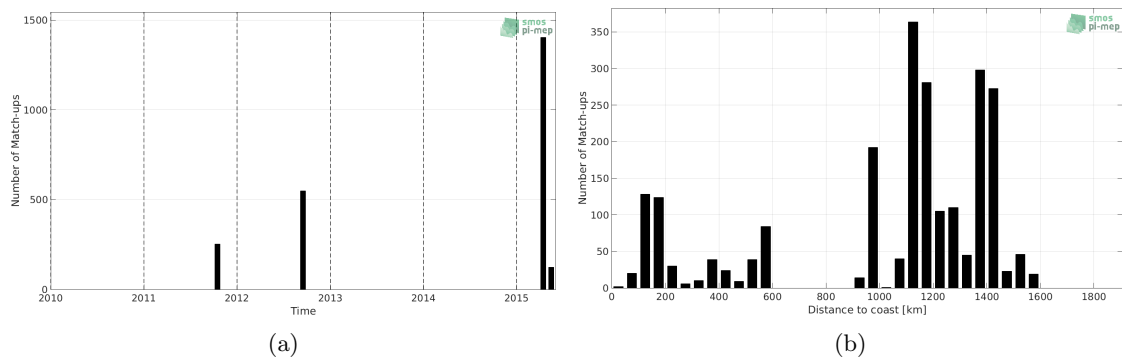
Figure 1: Number of match-ups between TSG-GOSUD-Research-vessel and Aquarius-L2-JPL-V5 SSS as a function of time (a) and as function of the distance to coast (b) over the OTT zone Pi-MEP region and for the full satellite product period.
