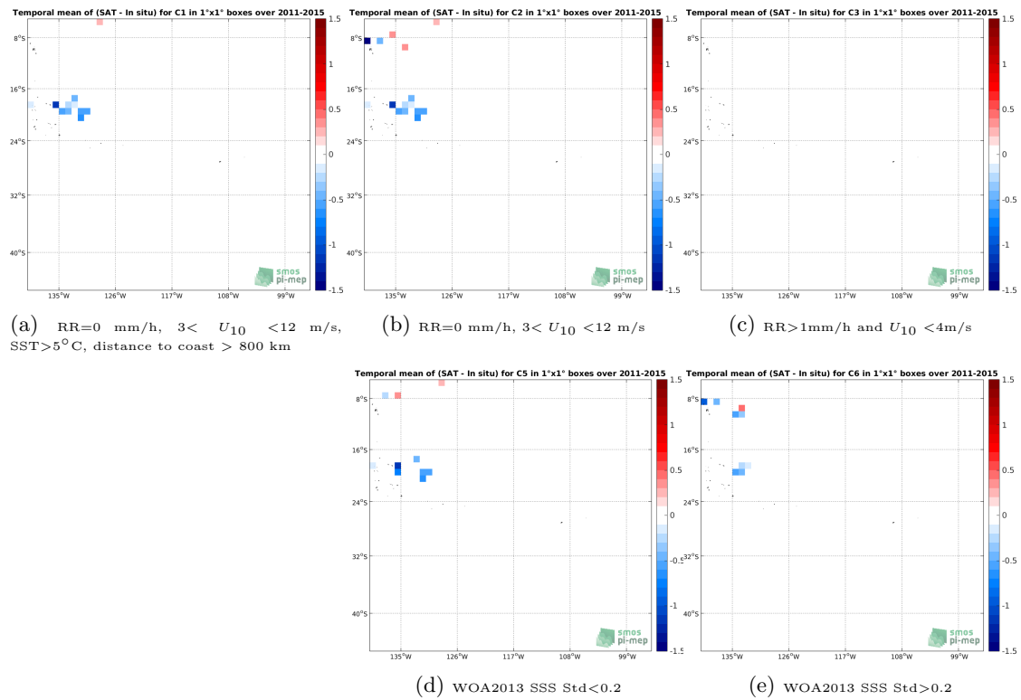
Figure 12: Temporal mean gridded over spatial boxes of size 1^\circ \times 1^\circ of \Delta SSS (Aquarius-L2-JPL-V5 - TSG-GOSUD-Research-vessel) for 5 different subdatasets corresponding to:RR=0 mm/h, 3 < U_{10} < 12 m/s, SST >5^\circ C, distance to coast > 800 km (a), RR=0 mm/h, 3 < U_{10} < 12 m/s (b), RR >1 mm/h and U_{10} < 4 m/s (c), WOA2013 SSS Std <0.2 (d), WOA2013 SSS Std >0.2 (e).
