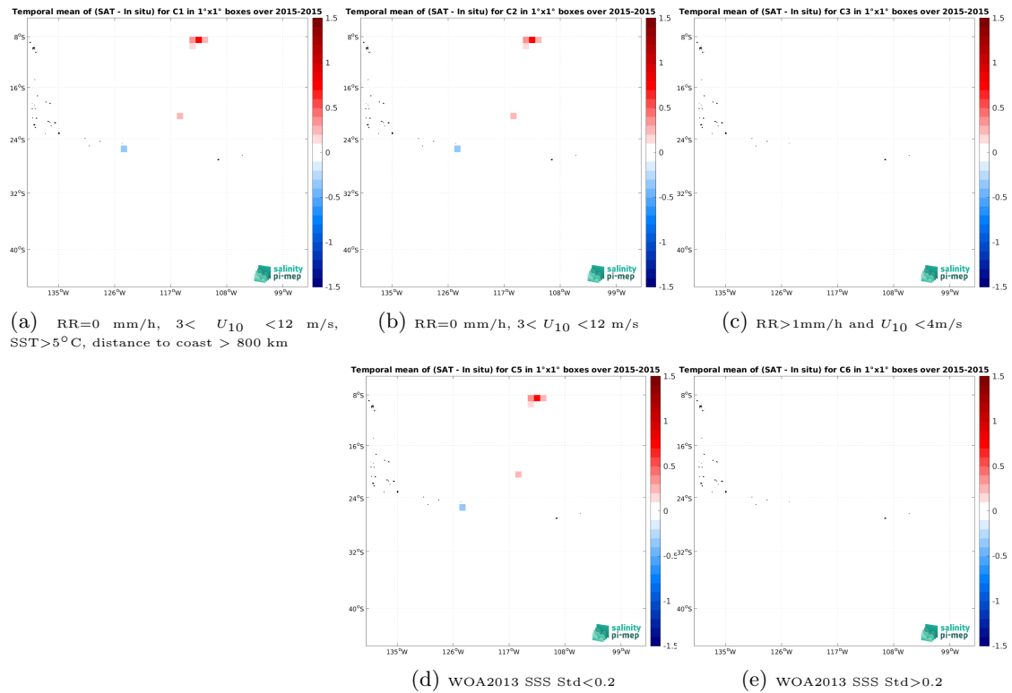
Figure 13: Temporal mean gridded over spatial boxes of size 1^\circ \times 1^\circ of \Delta SSS (Aquarius SSS L2 CAP v5 (JPL) - Surface drifters) for 5 different subdatasets corresponding to:RR=0 mm/h, 3 < U_{10} < 12 m/s, SST > 5^\circ\text{C} , distance to coast > 800 km (a), RR=0 mm/h, 3 < U_{10} < 12 m/s (b), RR > 1 mm/h and U_{10} < 4 m/s (c), WOA2013 SSS Std < 0.2 (d), WOA2013 SSS Std > 0.2 (e).
