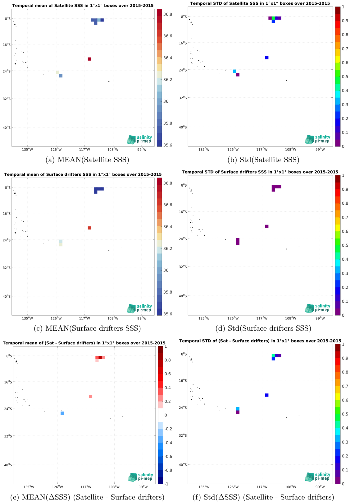
Figure 6: Temporal mean (left) and Std (right), of SSS from Aquarius SSS L2 CAP v5 (JPL) (top), Surface drifters (middle), and of \Delta SSS (Satellite - Surface drifters). Only match-up pairs are used to generate these maps.
