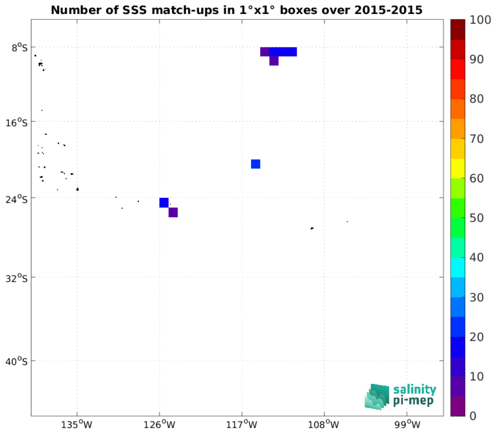
Figure 4: Number of SSS match-ups between Surface drifters SSS and the Aquarius SSS L2 CAP v5 (JPL) SSS product for the OTT zone Pi-MEP region over 1°x1° boxes and for the full satellite product period.
