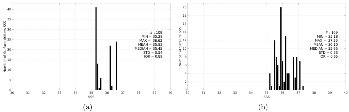
Figure 3: Histograms of SSS from Surface drifters (a) and Aquarius SSS L2 CAP v5 (JPL) (b) considering all match-up pairs per bins of 0.1 over the OTT zone Pi-MEP region and for the full satellite product period.
