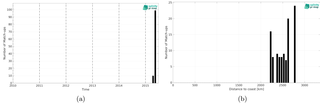
Figure 2: Number of match-ups between Surface drifters and Aquarius SSS L2 CAP v5 (JPL) SSS as a function of time (a) and as function of the distance to coast (b) over the OTT zone Pi-MEP region and for the full satellite product period.
