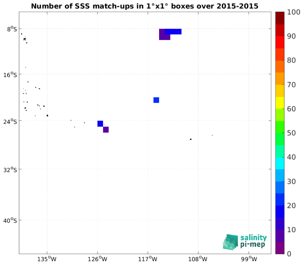
Figure 3: Number of SSS match-ups between Surface drifters SSS and the Aquarius SSS L2 CAP v5 (JPL) SSS product for the OTT zone Pi-MEP region over 1^\circ \times 1^\circ boxes and for the full satellite product period.
