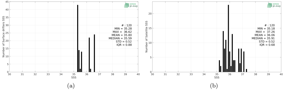
Figure 2: Histograms of SSS from Surface drifters (a) and Aquarius SSS L2 CAP v5 (JPL) (b) considering all match-up pairs per bins of 0.1 over the OTT zone Pi-MEP region and for the full satellite product period.
