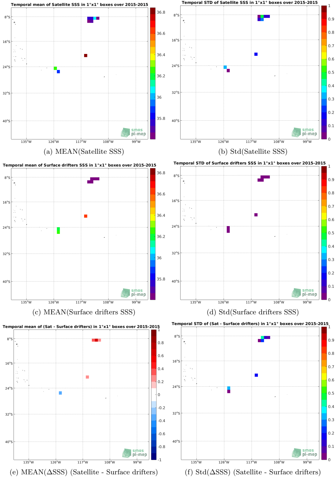
Figure 5: Temporal mean (left) and Std (right) of SSS from Aquarius SSS L2 CAP v5 (JPL) (top), Surface drifters (middle), and of \Delta SSS (Satellite - Surface drifters). Only match-up pairs are used to generate these maps.
