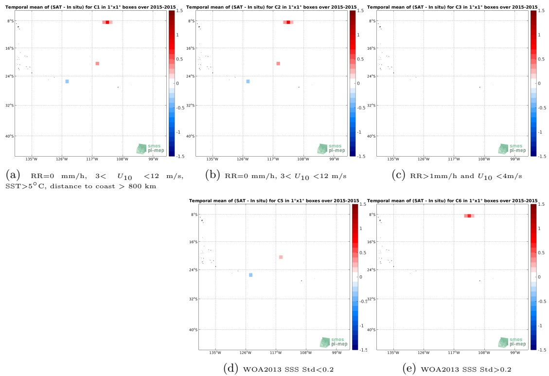
Figure 11: Temporal mean gridded over spatial boxes of size 1^\circ \times 1^\circ of \Delta SSS (Aquarius SSS L2 CAP v5 (JPL) - Surface drifters) for 5 different subdatasets corresponding to: RR=0 mm/h, 3 < U_{10} < 12 m/s, SST > 5^\circ C , distance to coast > 800 km (a), RR=0 mm/h, 3 < U_{10} < 12 m/s (b), RR > 1 mm/h and U_{10} < 4 m/s (c), WOA2013 SSS Std < 0.2 (d), WOA2013 SSS Std > 0.2 (e).
