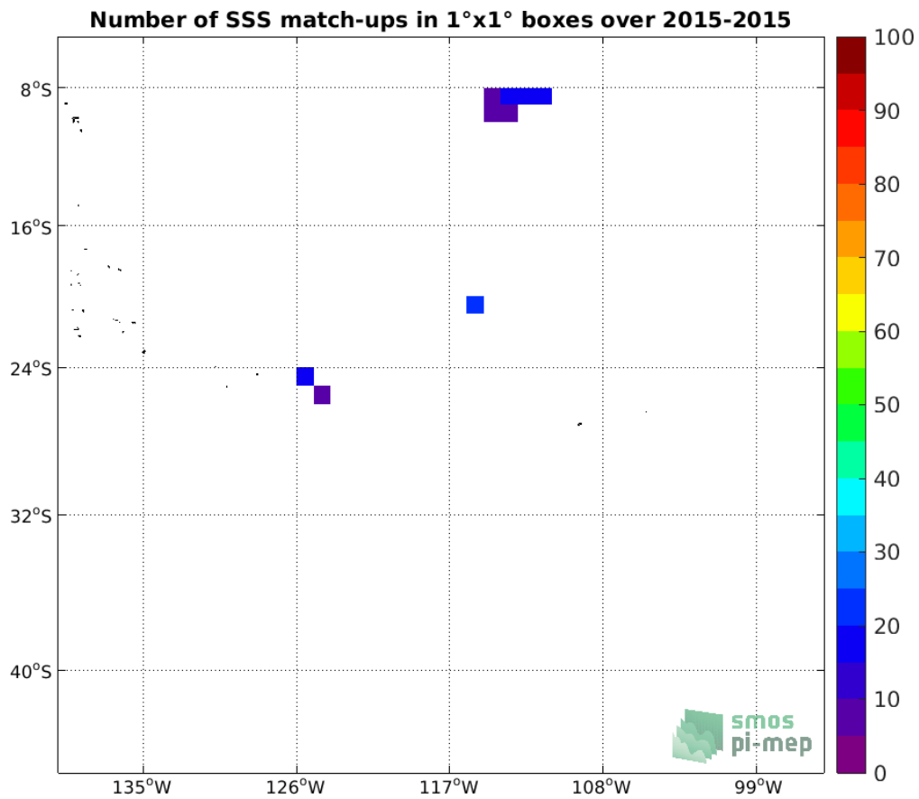
Figure 3: Number of SSS match-ups between Surface drifters SSS and the Aquarius SSS L2 CAP v5 (JPL) SSS product for the OTT zone Pi-MEP region over 1°x1° boxes and for the full satellite product period.
