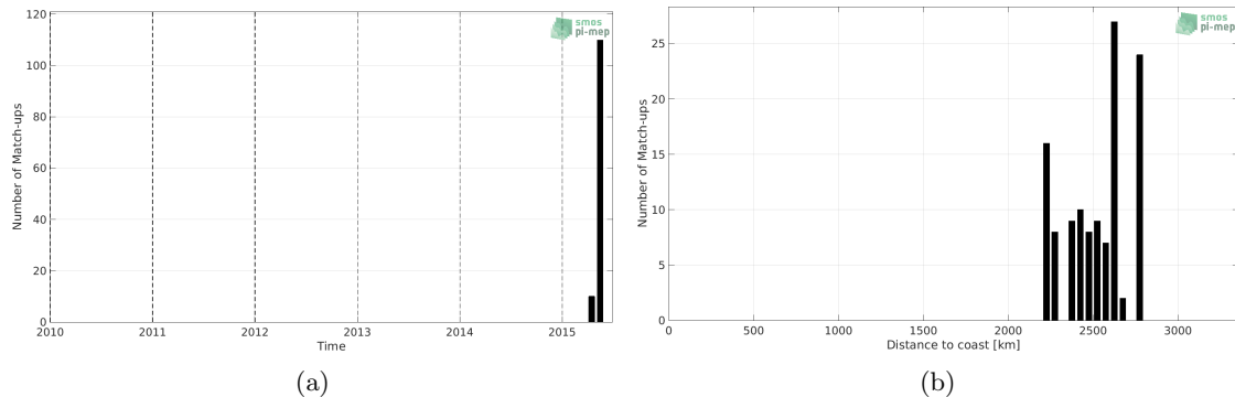
Figure 1: Number of match-ups between Surface drifters and Aquarius SSS L2 CAP v5 (JPL) SSS as a function of time (a) and as function of the distance to coast (b) over the OTT zone Pi-MEP region and for the full satellite product period.
