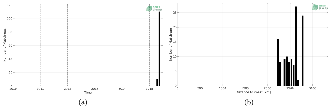
Figure 1: Number of match-ups between Surface drifters and Aquarius-L2-JPL-V5 SSS as a function of time (a) and as function of the distance to coast (b) over the OTT zone Pi-MEP region and for the full satellite product period.
