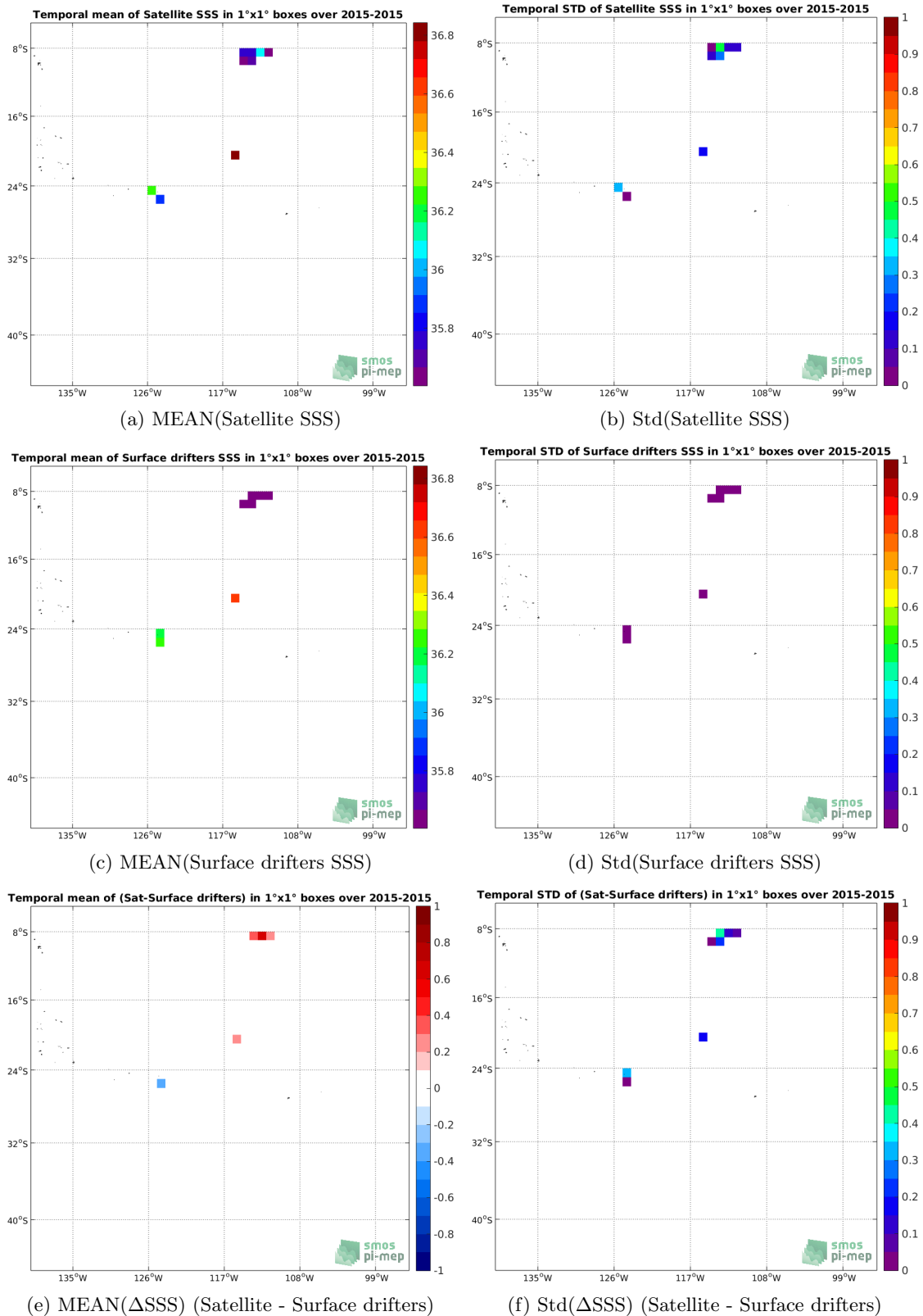
Figure 5: Temporal mean (left) and Std (right), of SSS from Aquarius-L2-JPL-V5 (top), Surface drifters (middle), and of \Delta SSS (Satellite - Surface drifters). Only match-up pairs are used to generate these maps.
