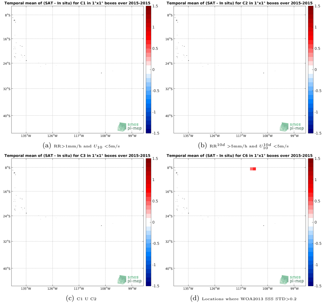
Figure 11: Temporal mean gridded over spatial boxes of size 1^\circ \times 1^\circ of \Delta SSS (Aquarius-L2-JPL-V5 - Surface drifters) for 4 different subdatasets corresponding to: RR > 1mm/h and U_{10} < 5\text{m/s} (a), RR^{10d} > 5\text{mm/h} and U_{10}^{10d} < 5\text{m/s} (b), C1 U C2 (c), Locations where WOA2013 SSS STD > 0.2 (d).
