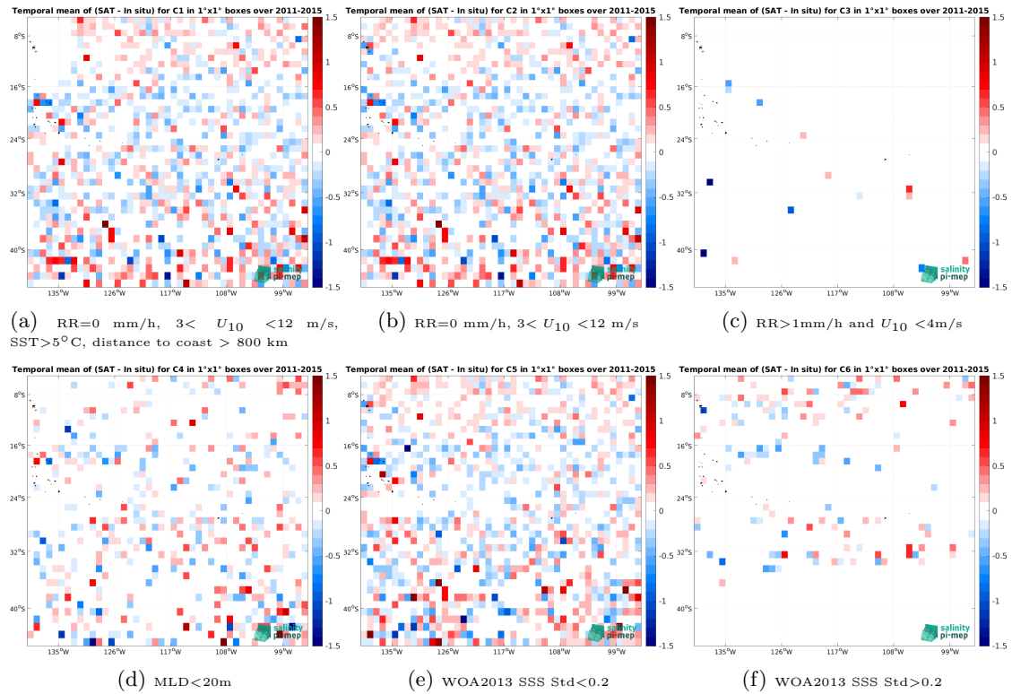
Figure 14: Temporal mean gridded over spatial boxes of size 1^\circ \times 1^\circ of \Delta SSS (Aquarius SSS L2 CAP v5 (JPL) - Argo) for 6 different subdatasets corresponding to:RR=0 mm/h, 3 < U_{10} < 12 m/s, SST >5^\circ C, distance to coast > 800 km (a), RR=0 mm/h, 3 < U_{10} < 12 m/s (b), RR >1 mm/h and U_{10} < 4 m/s (c),MLD <20 m (d),WOA2013 SSS Std <0.2 (e),WOA2013 SSS Std >0.2 (f).
