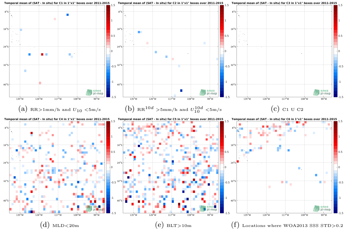
Figure 12: Temporal mean gridded over spatial boxes of size 1^\circ \times 1^\circ of \Delta\text{SSS} (Aquarius-L2-JPL-V5 - Argo) for 6 different subdatasets corresponding to: \text{RR} > 1\text{mm/h} and U_{10} < 5\text{m/s} (a), \text{RR}^{10d} > 5\text{mm/h} and U_{10}^{10d} < 5\text{m/s} (b), C1 U C2 (c), \text{MLD} < 20\text{m} (d), \text{BLT} > 10\text{m} (e), Locations where WOA2013 SSS STD > 0.2 (f).
