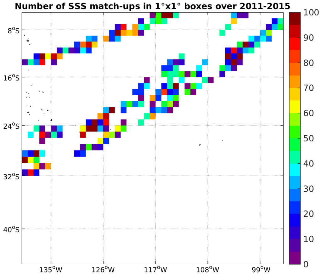
Figure 4: Number of SSS match-ups between TSG-LEGOS-DM SSS and the AQUARIUS-L2-JPL-V4 SSS product for the OTT zone Pi-MEP region over 1°x1° boxes and for the full satellite product period.
