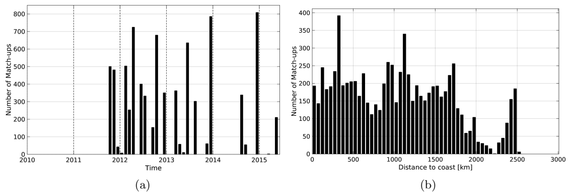
Figure 1: Number of match-ups between TSG-LEGOS-DM and AQUARIUS-L2-JPL-V4 SSS as a function of time (a) and as function of the distance to coast (b) over the OTT zone Pi-MEP region and for the full satellite product period.
