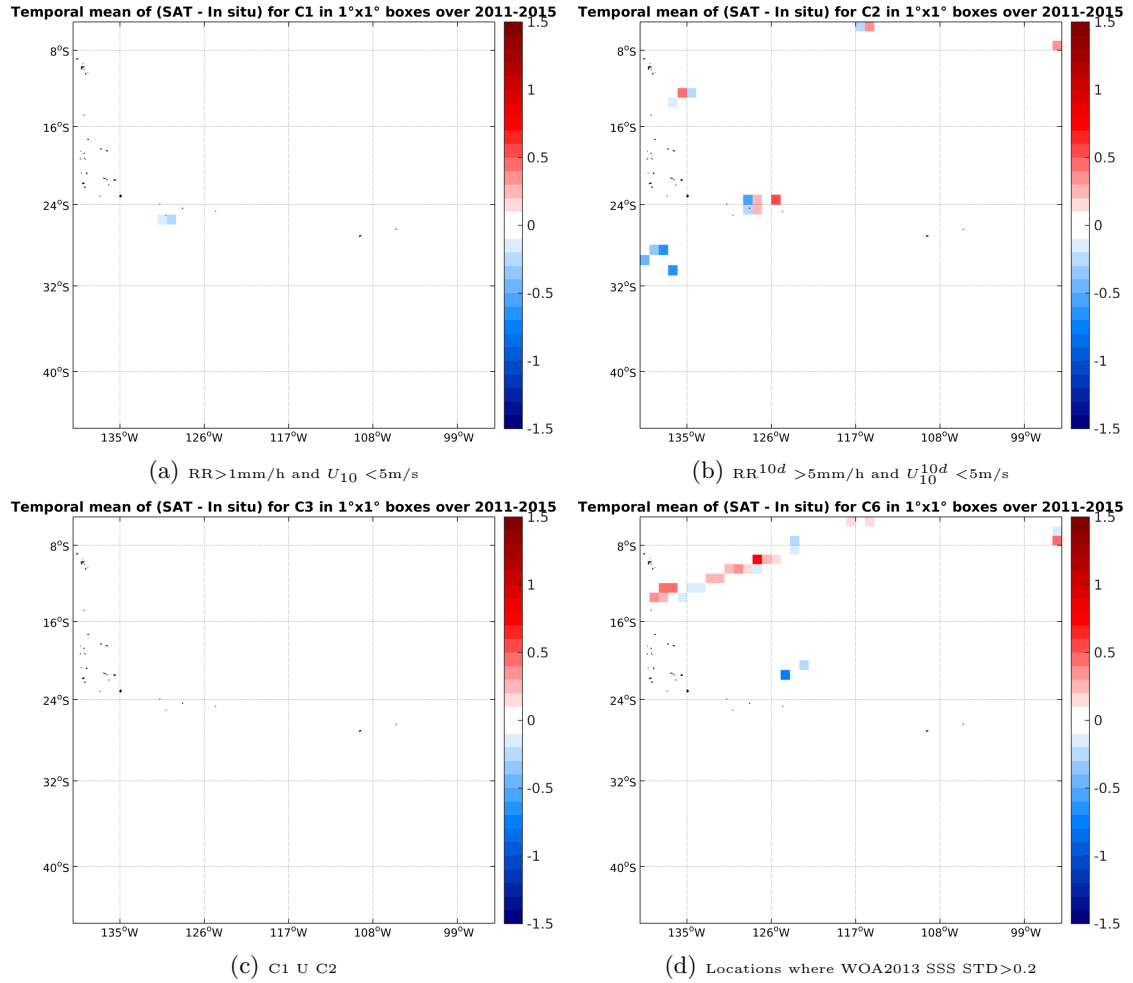
Figure 12: Temporal mean gridded over spatial boxes of size 1°x1° of \Delta SSS (AQUARIUS-L2-JPL-V4 - TSG-LEGOS-DM) for 4 different subdatasets corresponding to: RR > 1\text{mm/h} and U_{10} < 5\text{m/s} (a), RR^{10d} > 5\text{mm/h} and U_{10}^{10d} < 5\text{m/s} (b), C1 U C2 (c), Locations where WOA2013 SSS STD > 0.2 (d).
