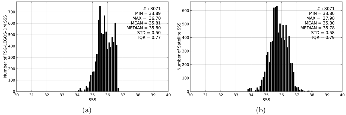
Figure 2: Histograms of SSS from TSG-LEGOS-DM (a) and AQUARIUS-L2-JPL-V4 (b) considering all match-up pairs per bins of 0.1 over the OTT zone Pi-MEP region and for the full satellite product period.
