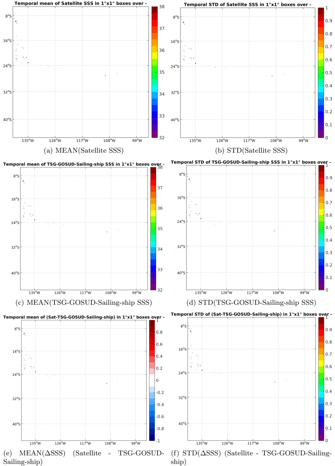
Figure 6: Temporal mean (left) and STD (right) of SSS from AQUARIUS-L2-JPL-V4 (top), TSG-GOSUD-Sailing-ship (middle), and of \Delta SSS (Satellite - TSG-GOSUD-Sailing-ship). Only match-up pairs are used to generate these maps.
