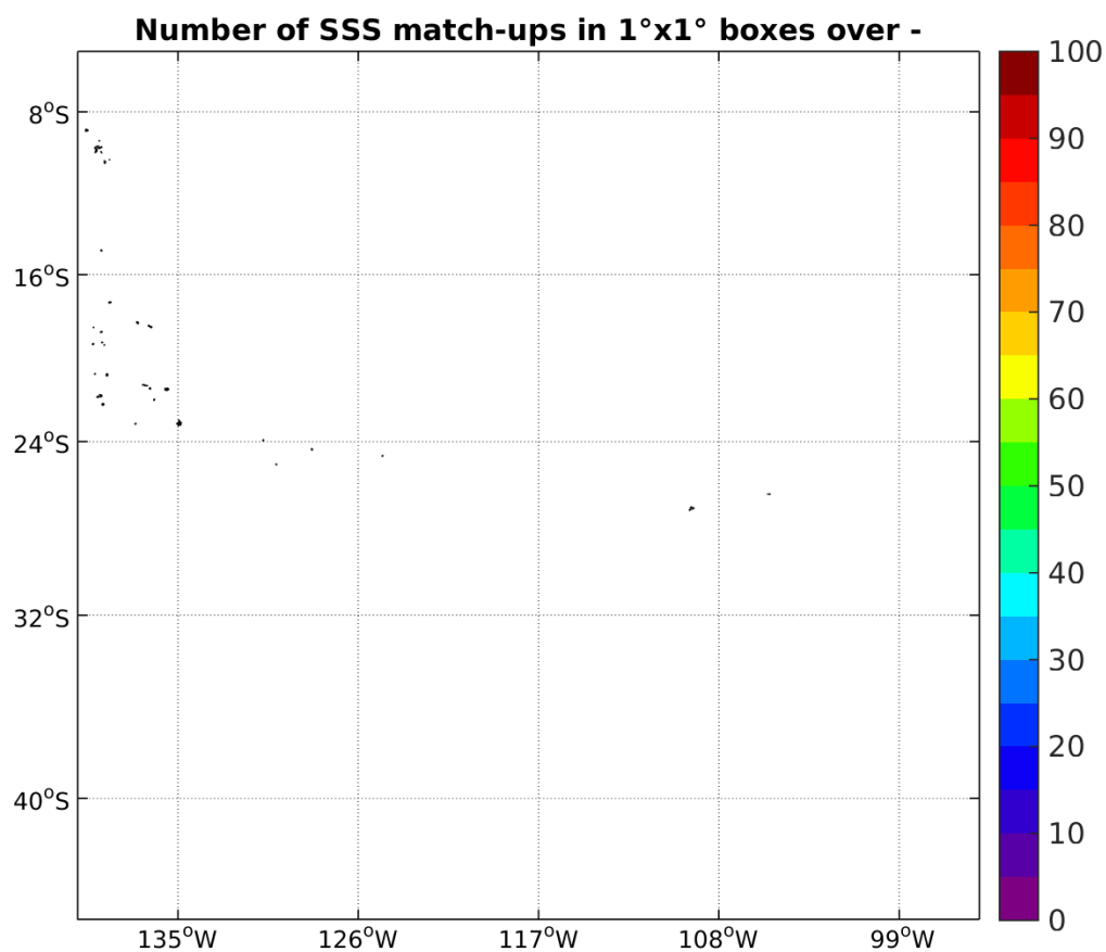
Figure 4: Number of SSS match-ups between TSG-GOSUD-Sailing-ship SSS and the AQUARIUS-L2-JPL-V4 SSS product for the OTT zone Pi-MEP region over 1°x1° boxes and for the full satellite product period.
