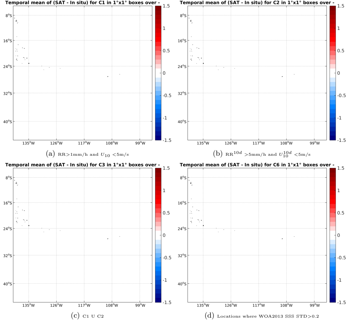
Figure 12: Temporal mean gridded over spatial boxes of size 1^\circ \times 1^\circ of \Delta SSS (AQUARIUS-L2-JPL-V4 - TSG-GOSUD-Sailing-ship) for 4 different subdatasets corresponding to: RR > 1\text{mm/h} and U_{10} < 5\text{m/s} (a), RR^{10d} > 5\text{mm/h} and U_{10}^{10d} < 5\text{m/s} (b), C1 U C2 (c), Locations where WOA2013 SSS STD > 0.2 (d).
