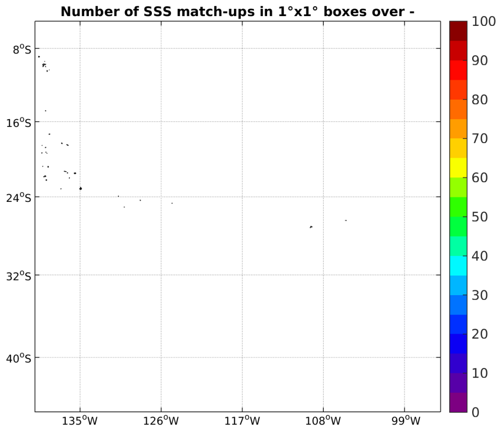
Figure 3: Number of SSS match-ups between Surface drifters SSS and the AQUARIUS-L2-JPL-V4 SSS product for the OTT zone Pi-MEP region over 1°x1° boxes and for the full satellite product period.
