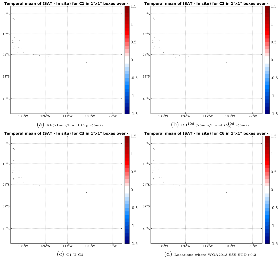
Figure 11: Temporal mean gridded over spatial boxes of size 1°x1° of \Delta SSS (AQUARIUS-L2-JPL-V4 - Surface drifters) for 4 different subdatasets corresponding to: RR > 1mm/h and U_{10} < 5\text{m/s} (a), RR^{10d} > 5\text{mm/h} and U_{10}^{10d} < 5\text{m/s} (b), C1 U C2 (c), Locations where WOA2013 SSS STD > 0.2 (d).
