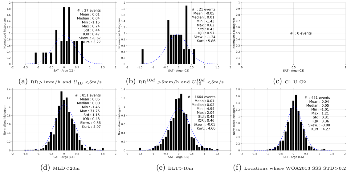
Figure 13: Normalized histogram of \Delta SSS (AQUARIUS-L2-JPL-V4 - Argo) for 6 different sub-datasets corresponding to: RR > 1mm/h and U_{10} < 5 m/s (a), RR^{10d} > 5 mm/h and U_{10}^{10d} < 5 m/s (b), C1 U C2 (c), MLD < 20m (d), BLT > 10m (e), Locations where WOA2013 SSS STD > 0.2 (f).
