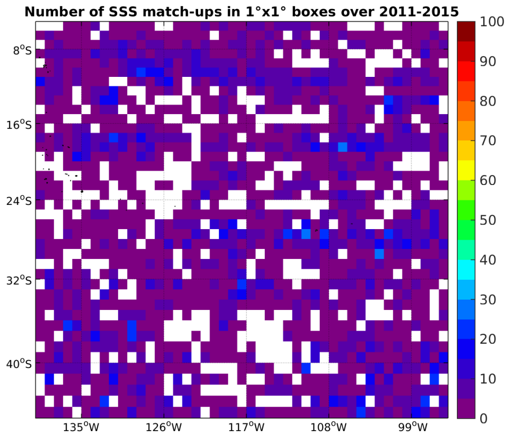
Figure 4: Number of SSS match-ups between Argo SSS and the AQUARIUS-L2-JPL-V4 SSS product for the OTT zone Pi-MEP region over 1°x1° boxes and for the full satellite product period.
