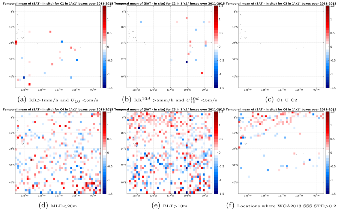
Figure 12: Temporal mean gridded over spatial boxes of size 1^\circ \times 1^\circ of \Delta\text{SSS} (AQUARIUS-L2-JPL-V4 - Argo) for 6 different subdatasets corresponding to: \text{RR} > 1\text{mm/h} and U_{10} < 5\text{m/s} (a), \text{RR}^{10d} > 5\text{mm/h} and U_{10}^{10d} < 5\text{m/s} (b), C1 U C2 (c), \text{MLD} < 20\text{m} (d), \text{BLT} > 10\text{m} (e), Locations where WOA2013 SSS STD > 0.2 (f).
