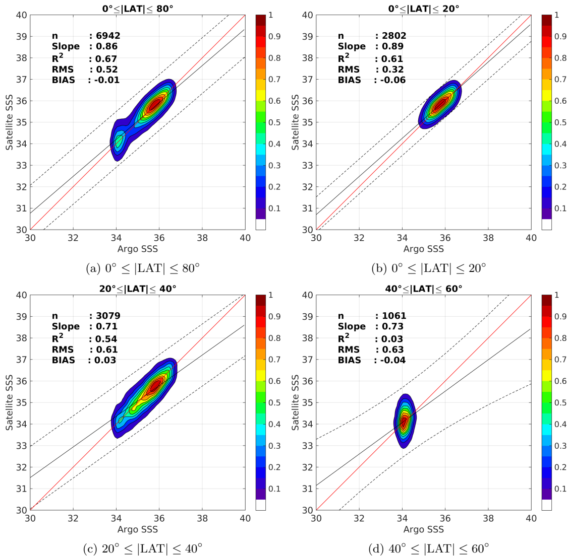
Figure 9: Contour maps of the concentration of AQUARIUS-L2-JPL-V4 SSS (y-axis) versus Argo SSS (x-axis) at match-up pairs for different latitude bands. For each plot, the red line shows x=y . The black thin and dashed lines indicate a linear fit through the data cloud and the \pm 95\% confidence levels, respectively. The number match-up pairs n , the slope and R^2 coefficient of the linear fit, the root mean square (RMS) and the mean bias between satellite and in situ data are indicated for each latitude band in each plots.
