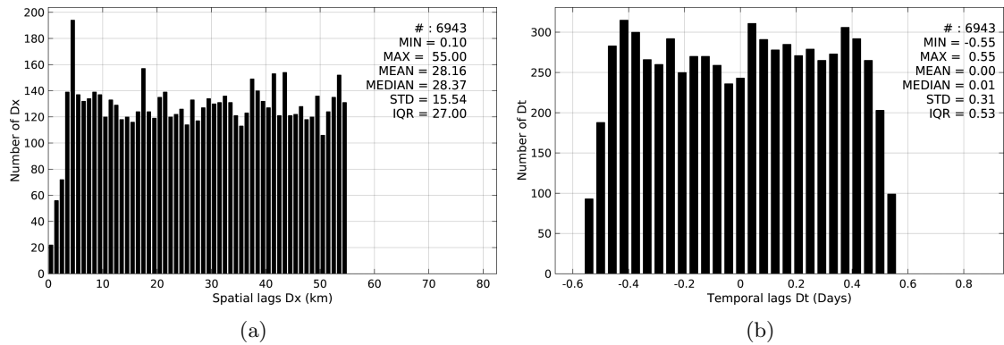
Figure 5: Histograms of the spatial (a) and temporal (b) lags between the time of the Argo measurements and the date of the corresponding AQUARIUS-L2-JPL-V4 SSS product.
