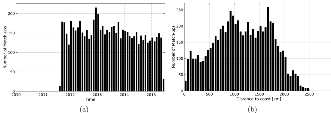
Figure 1: Number of match-ups between Argo and AQUARIUS-L2-JPL-V4 SSS as a function of time (a) and as function of the distance to coast (b) over the OTT zone Pi-MEP region and for the full satellite product period.
