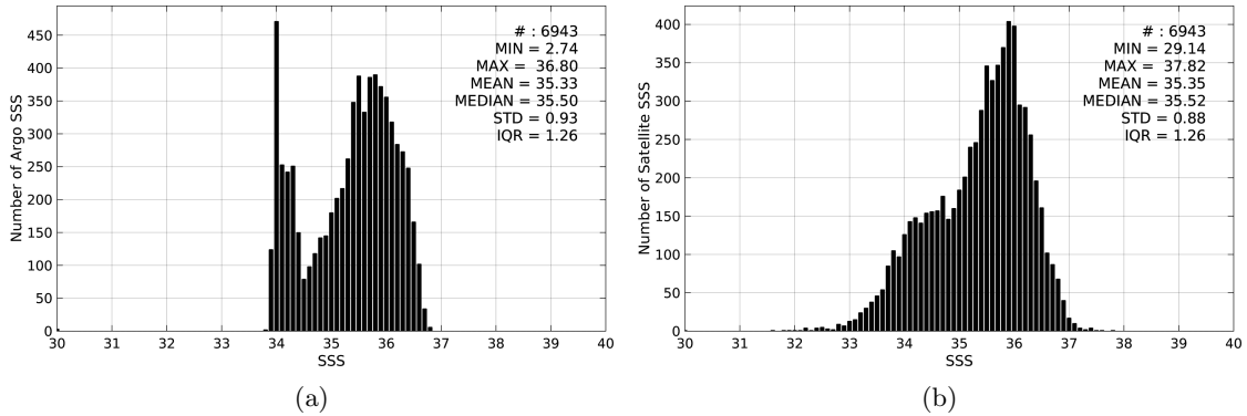
Figure 2: Histograms of SSS from Argo (a) and AQUARIUS-L2-JPL-V4 (b) considering all match-up pairs per bins of 0.1 over the OTT zone Pi-MEP region and for the full satellite product period.
