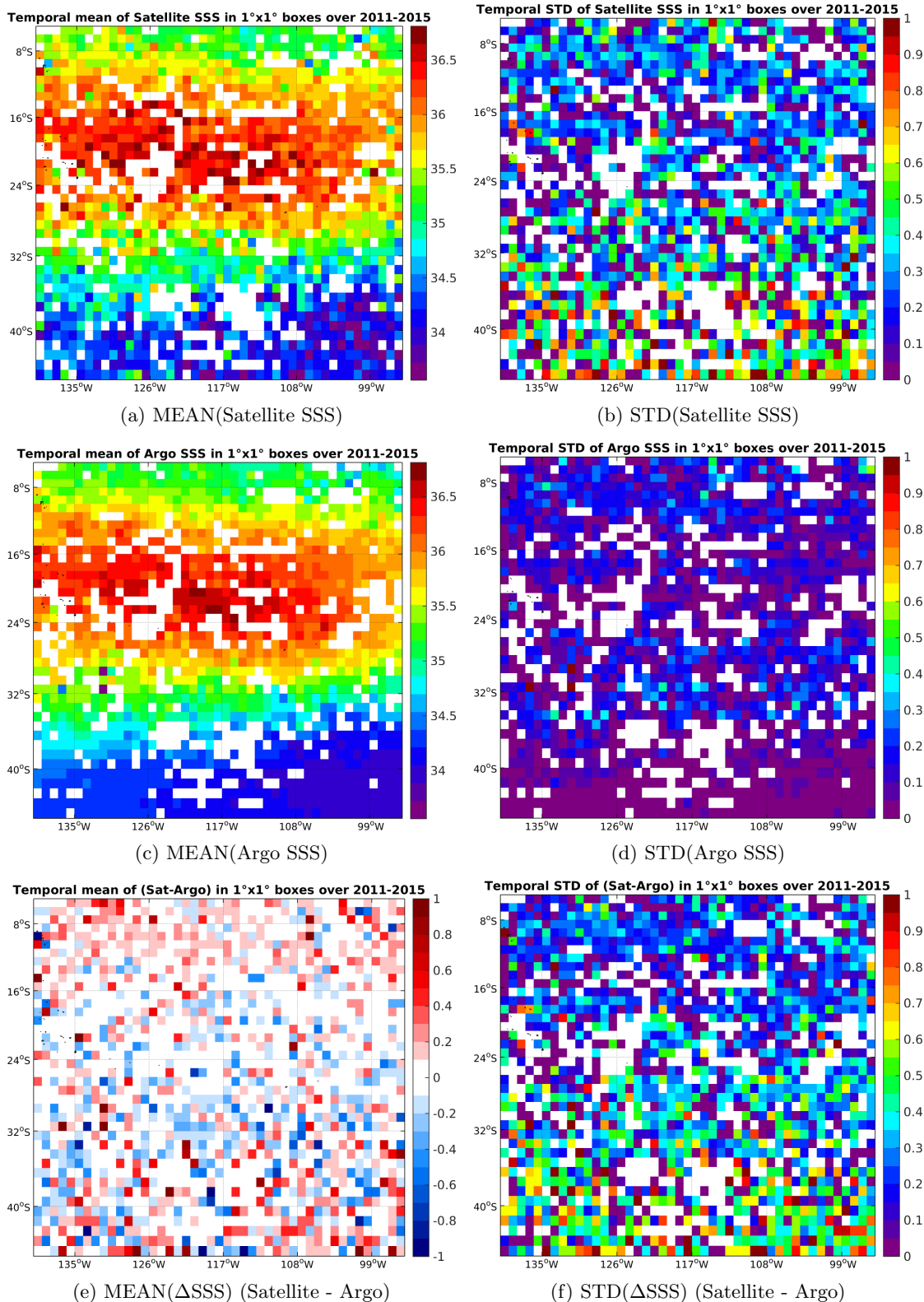
Figure 6: Temporal mean (left) and STD (right) of SSS from AQUARIUS-L2-JPL-V4 (top), Argo (middle), and of \Delta SSS (Satellite - Argo). Only match-up pairs are used to generate these maps.
