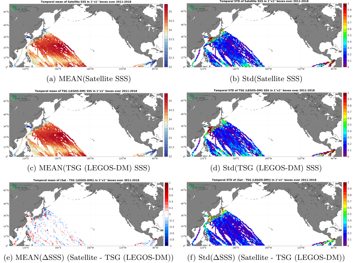
Figure 6: Temporal mean (left) and Std (right) of SSS from SMOS and SMAP SSS L4 OI v1 - 7 Days (LOPS) (top), TSG (LEGOS-DM) (middle), and of \Delta\text{SSS}(\text{Satellite} - \text{TSG}(\text{LEGOS-DM})) . Only match-up pairs are used to generate these maps.
