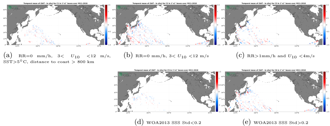
Figure 12: Temporal mean gridded over spatial boxes of size 1^\circ \times 1^\circ of \Delta SSS (SMOS and SMAP SSS L4 OI v1 - 7 Days (LOPS) - TSG (LEGOS-DM)) for 5 different subdatasets corresponding to:RR=0 mm/h, 3 < U_{10} < 12 m/s, SST >5^\circ\text{C} , distance to coast > 800 km (a), RR=0 mm/h, 3 < U_{10} < 12 m/s (b), RR >1 mm/h and U_{10} < 4 m/s (c), WOA2013 SSS Std <0.2 (d), WOA2013 SSS Std >0.2 (e).
