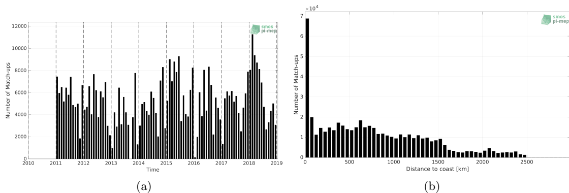
Figure 1: Number of match-ups between TSG (LEGOS-DM) and SMOS and SMAP SSS L4 OI v1 - 7 Days (LOPS) SSS as a function of time (a) and as function of the distance to coast (b) over the North Pacific Ocean Pi-MEP region and for the full satellite product period.
