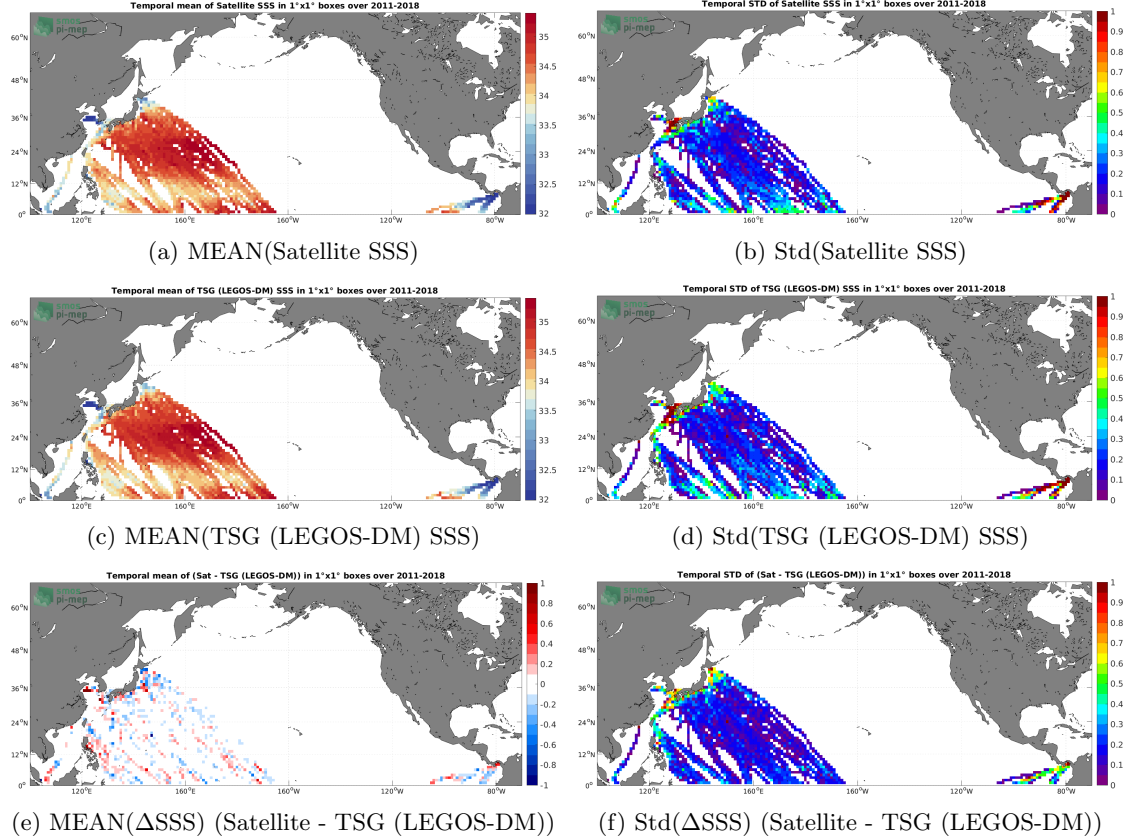
Figure 6: Temporal mean (left) and Std (right) of SSS from SMOS and SMAP SSS L4 OI v1 - 7 Days (LOPS) (top), TSG (LEGOS-DM) (middle), and of \Delta\text{SSS} (Satellite - TSG (LEGOS-DM)). Only match-up pairs are used to generate these maps.
