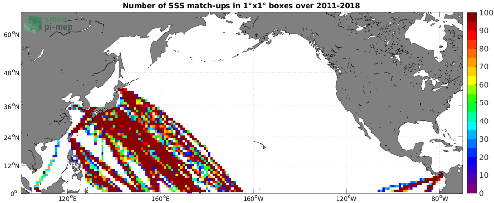
Figure 4: Number of SSS match-ups between TSG (LEGOS-DM) SSS and the SMOS and SMAP SSS L4 OI v1 - 7 Days (LOPS) SSS product for the North Pacific Ocean Pi-MEP region over 1^\circ \times 1^\circ boxes and for the full satellite product period.
