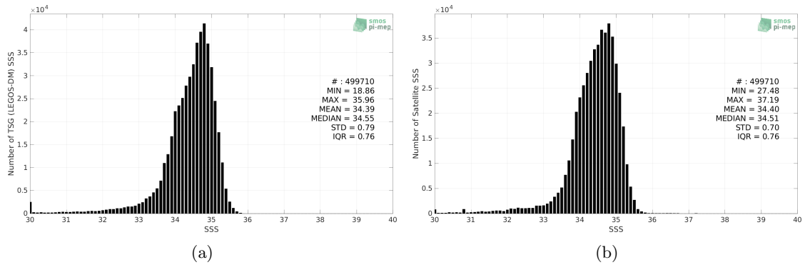
Figure 2: Histograms of SSS from TSG (LEGOS-DM) (a) and SMOS and SMAP SSS L4 OI v1 - 7 Days (LOPS) (b) considering all match-up pairs per bins of 0.1 over the North Pacific Ocean Pi-MEP region and for the full satellite product period.
